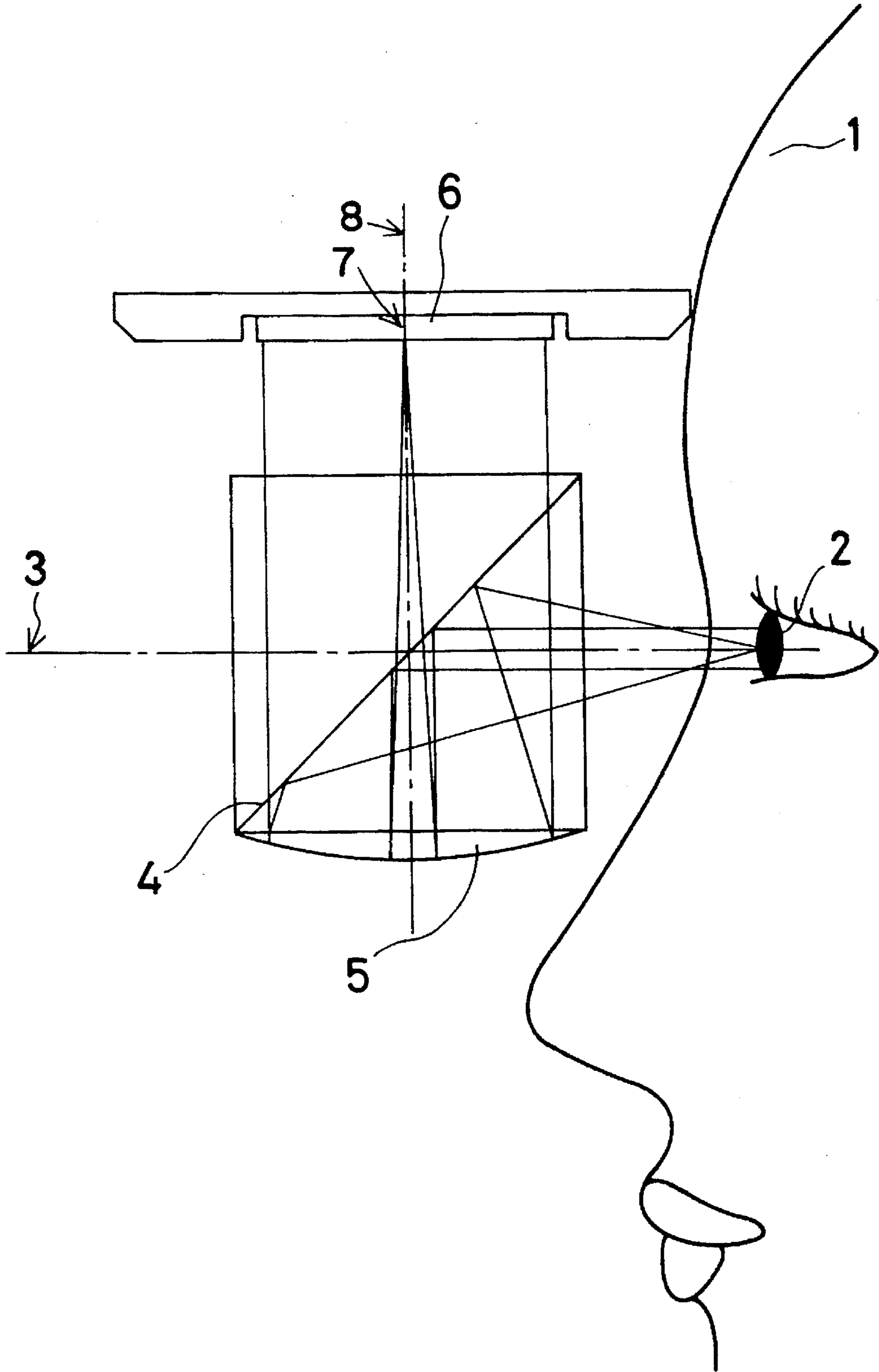
FIG. 18 (PRIOR ART)
