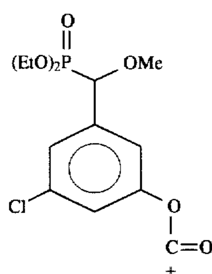
Diethyl 1-methoxy-1-(3-chloro-5-pivaloyloxyphenyl)methane phosphonate ( 14 )
