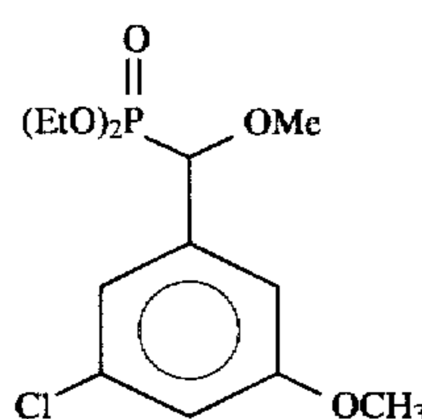
Diethyl 1-methoxy, 1-(3-chloro-5-methoxyphenyl)methane phosphonate (8)
