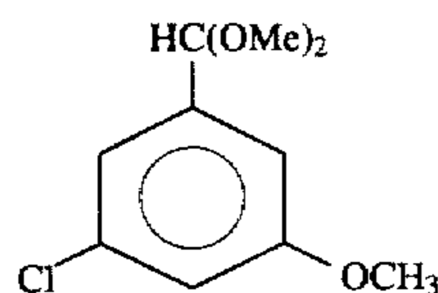
3-Chloro-5-methoxybenzaldehyde dimethyl acetal (7)
