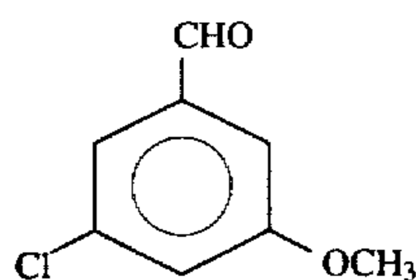
3-Chloro-5-methoxybenzaldehyde (6)
