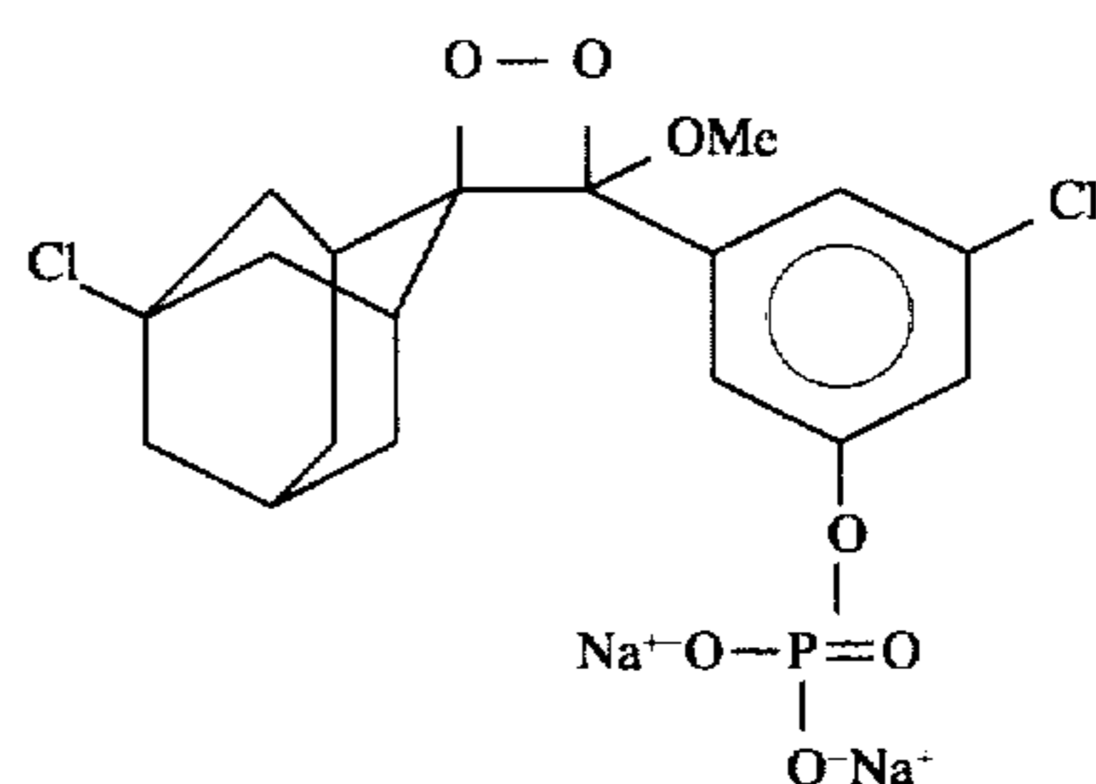
Disodium 3-chloro-5-(methoxyspiro[1,2-dioxetane-3,2'-(5-chloro)-tricyclo[3.3.1.1 3,7 ]-decan]-4-yl)-1-phenyl phosphate ( 2 )
