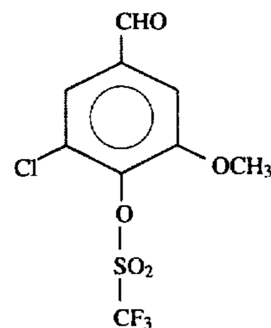
3-Chloro-5-methoxy-4-trifluoromethanesulfonyloxy benzaldehyde (5).
