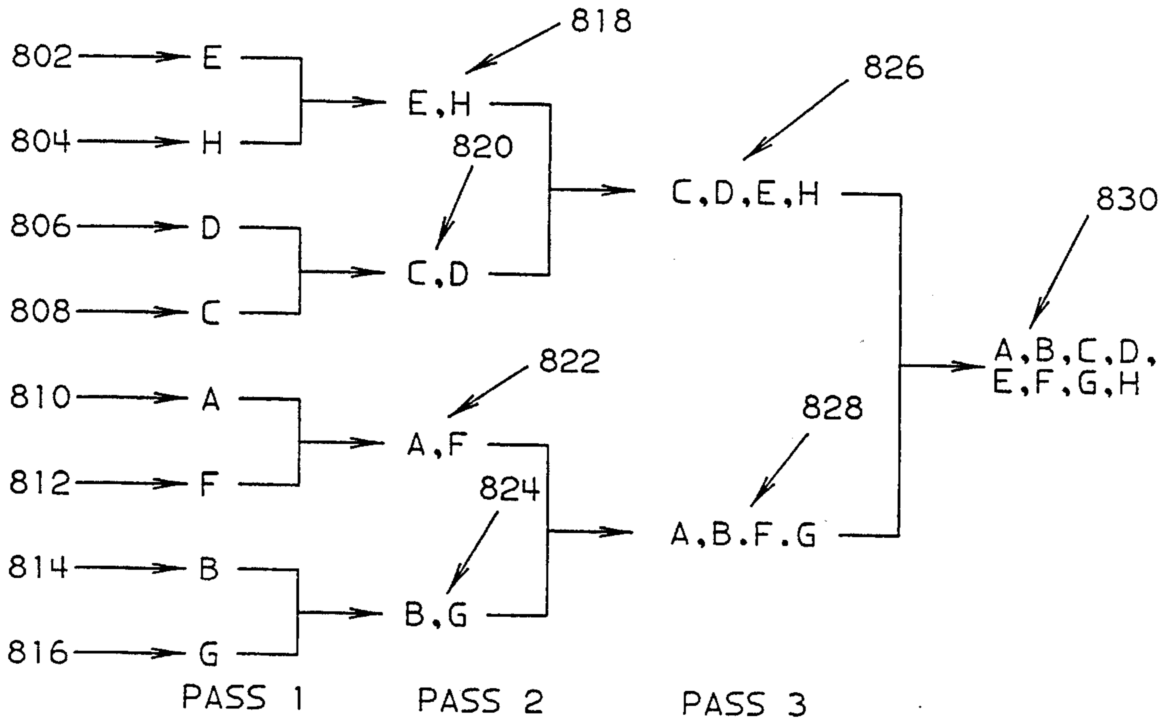
FIG. 8 BLOCK SORT (BINARY MERGE/SORT)
