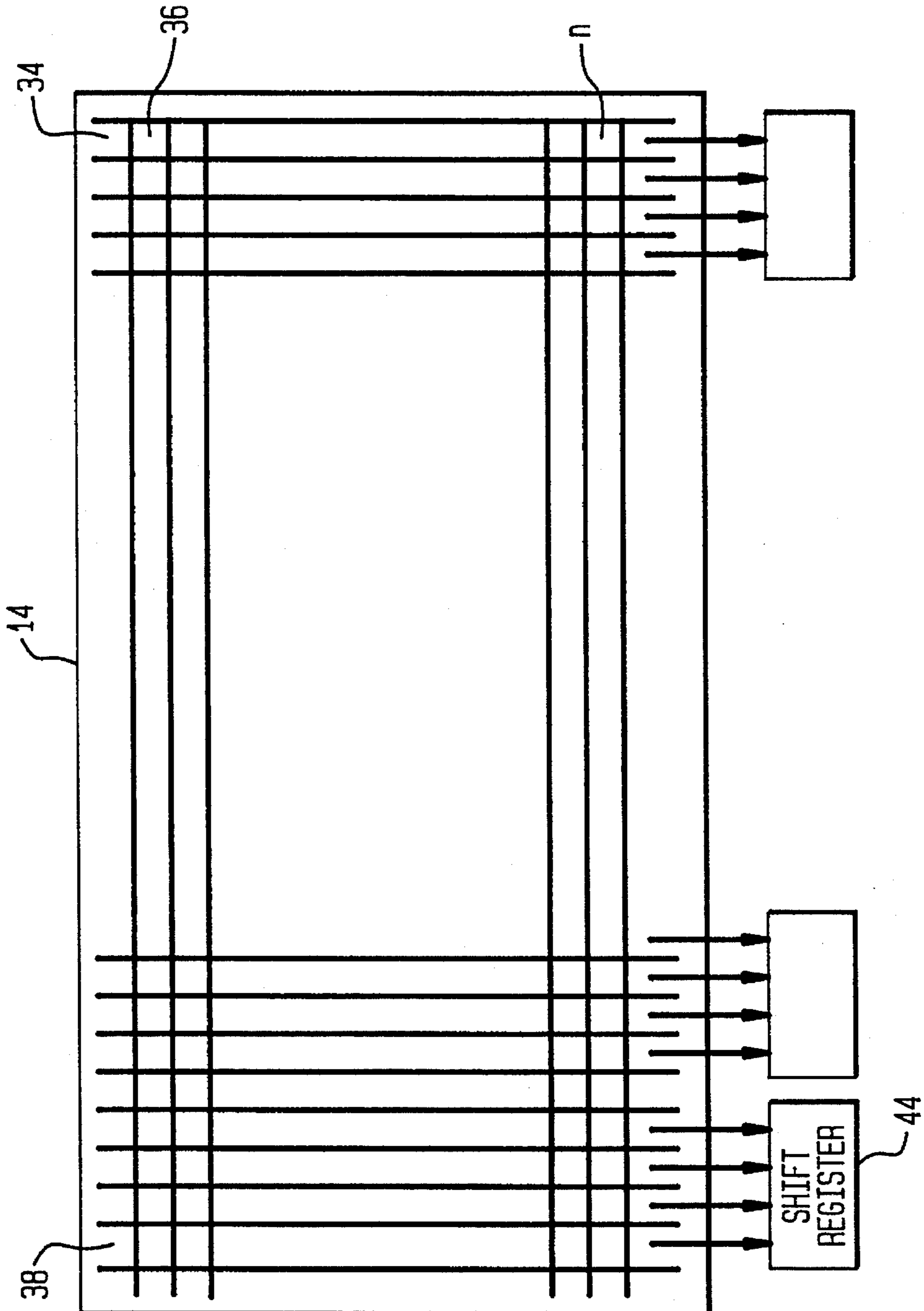
FIG. 6 (PRIOR ART)
