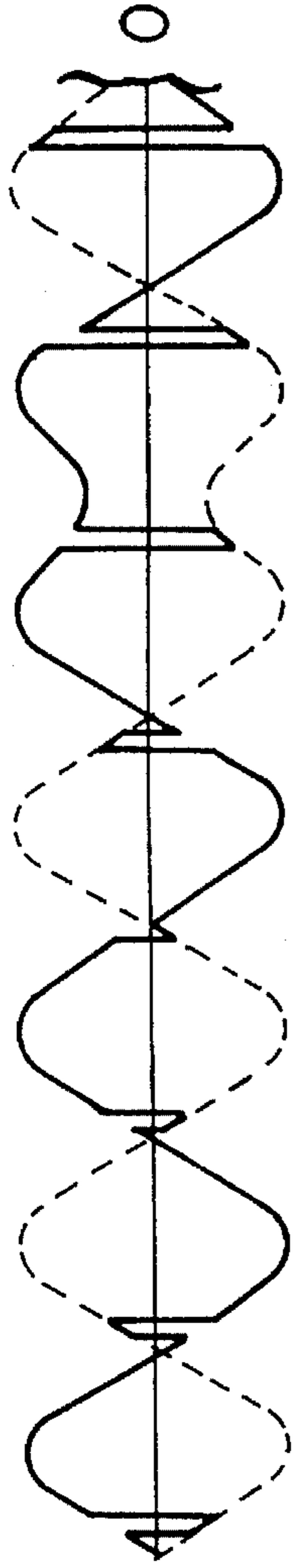
FIG.14 ENVELOPE WAVEFORM OF PUSH-PULL SIGNAL WITHOUT OFFSET
