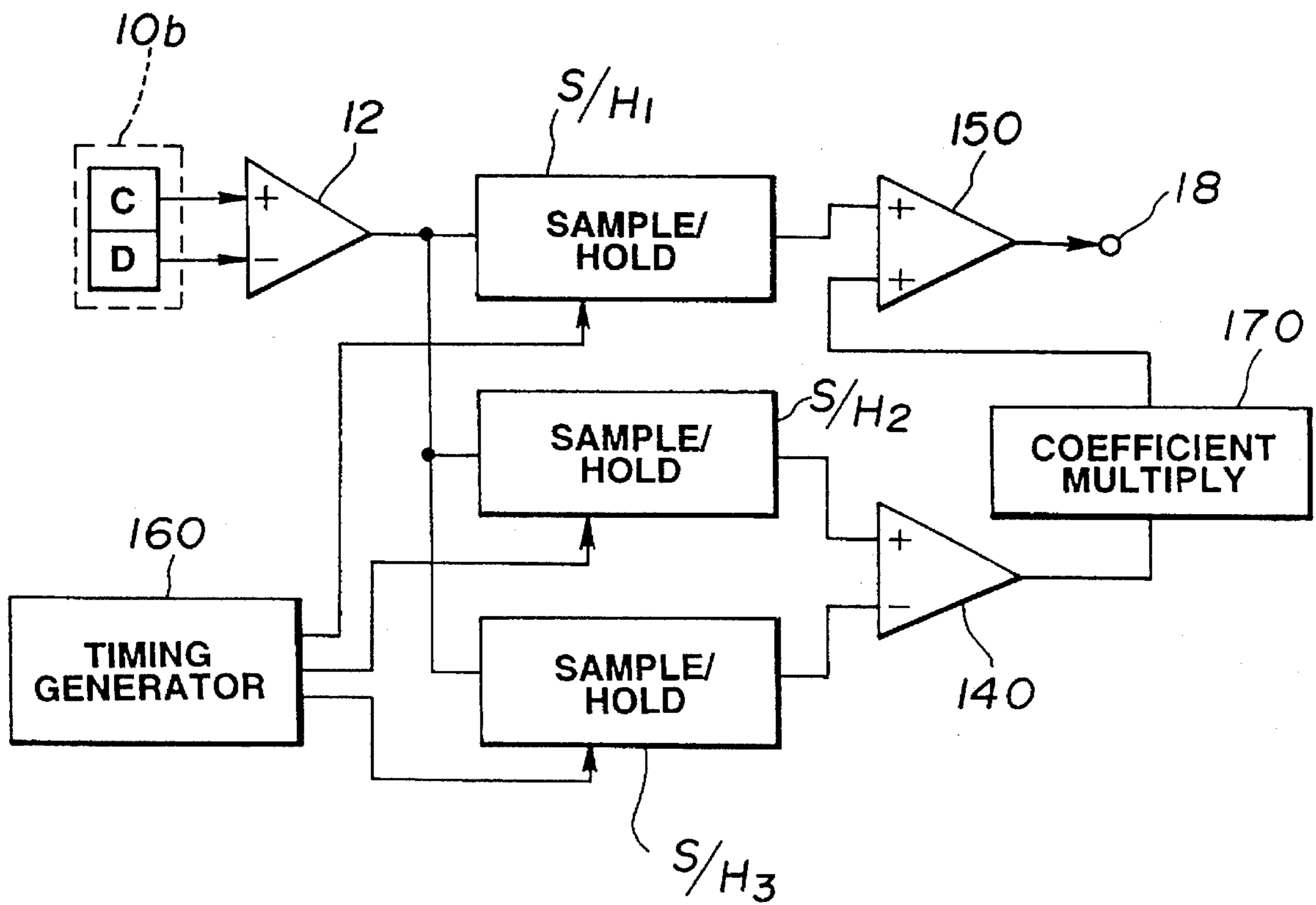
FIG. 4 (PRIOR ART)
