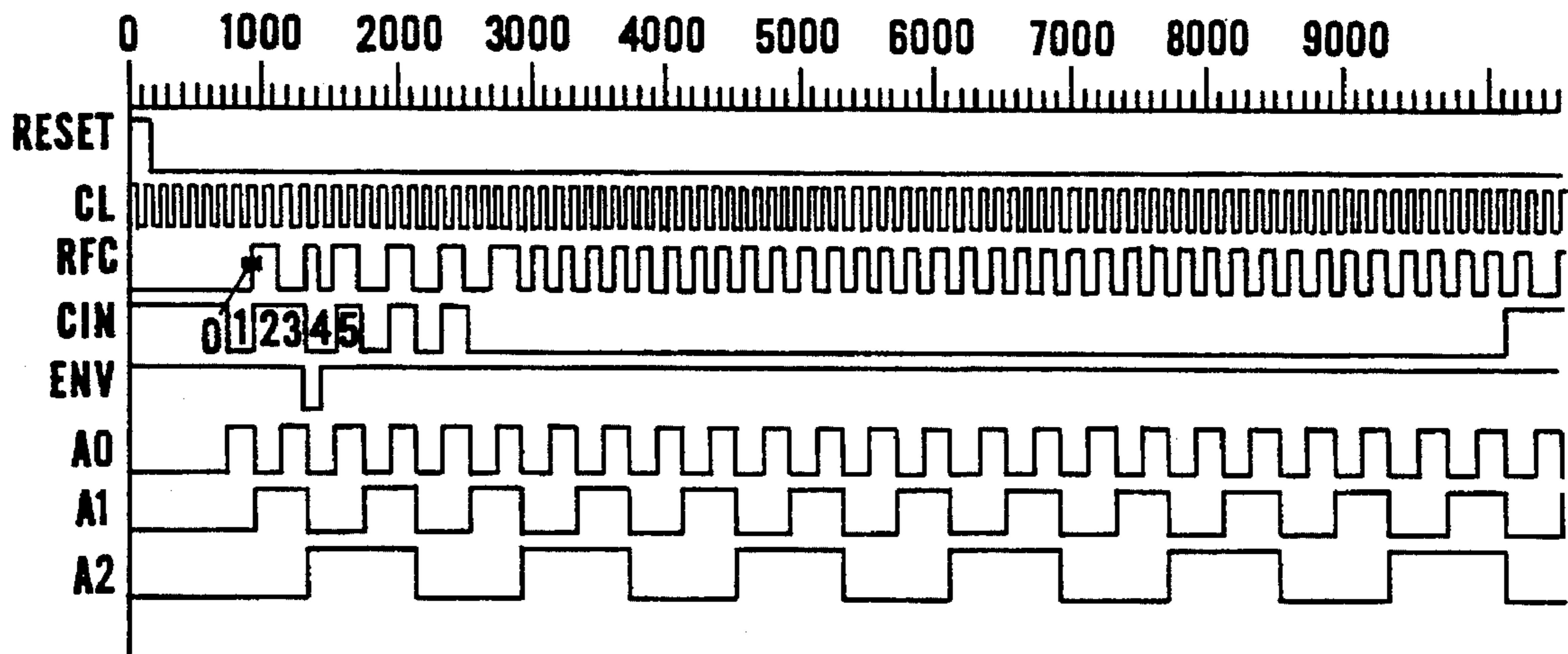
WAVEFORMS WITH NO GAP DETECTION OR SYNCHRONIZATION
