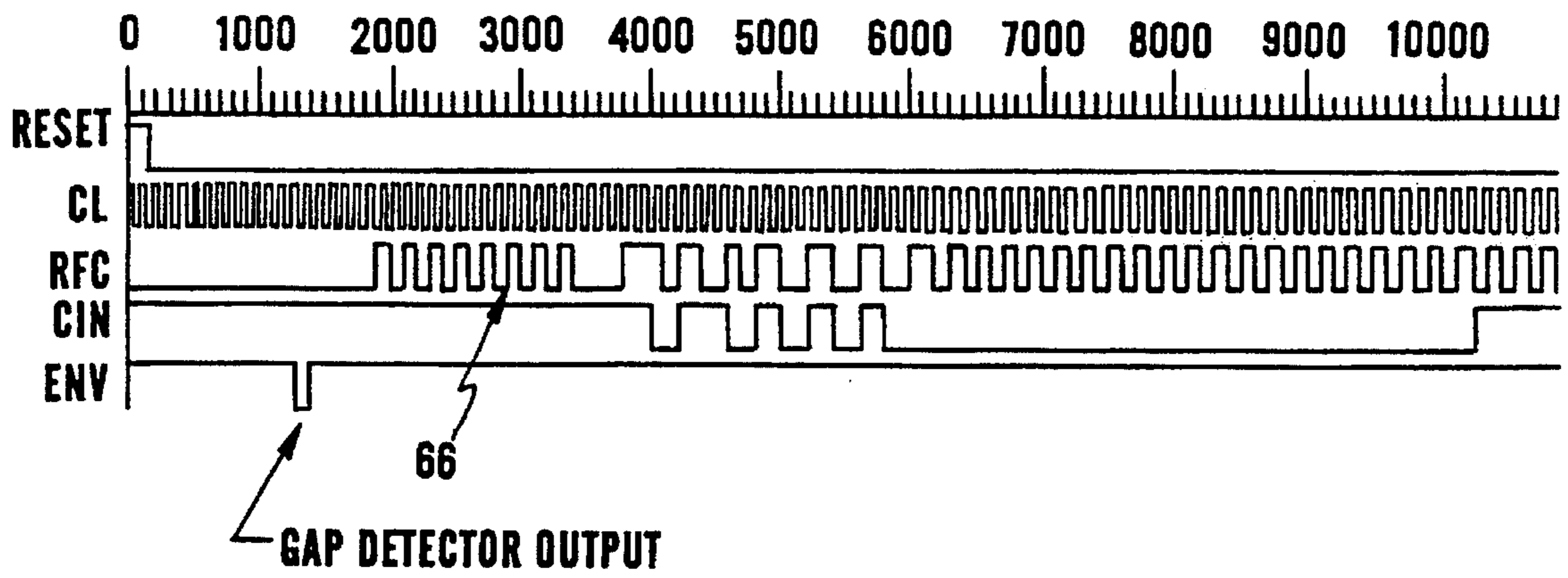
WAVEFORMS WITH GAP DETECTION AND SYNCHRONIZATION
