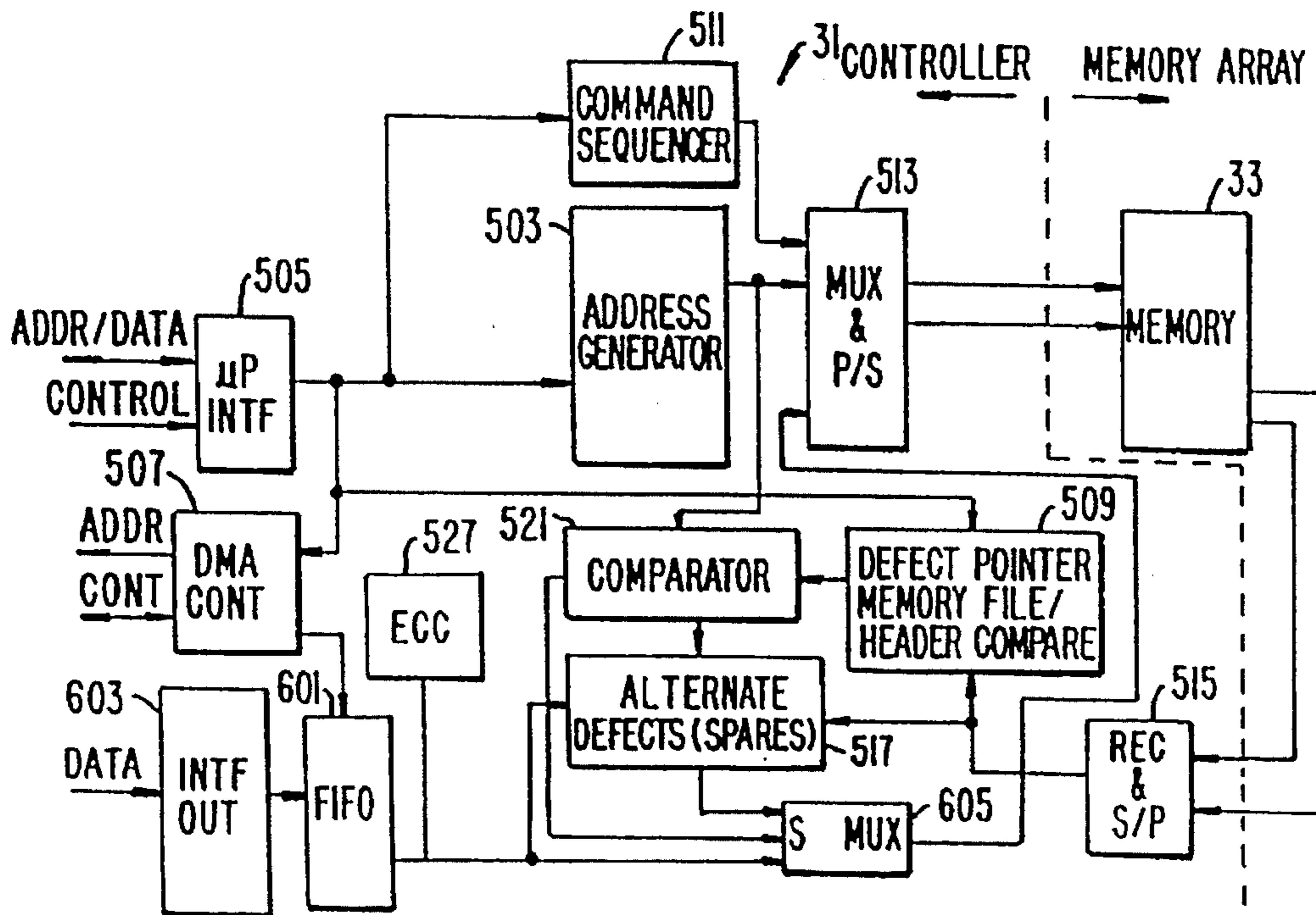
WRITE DATA PATH CONTROL
