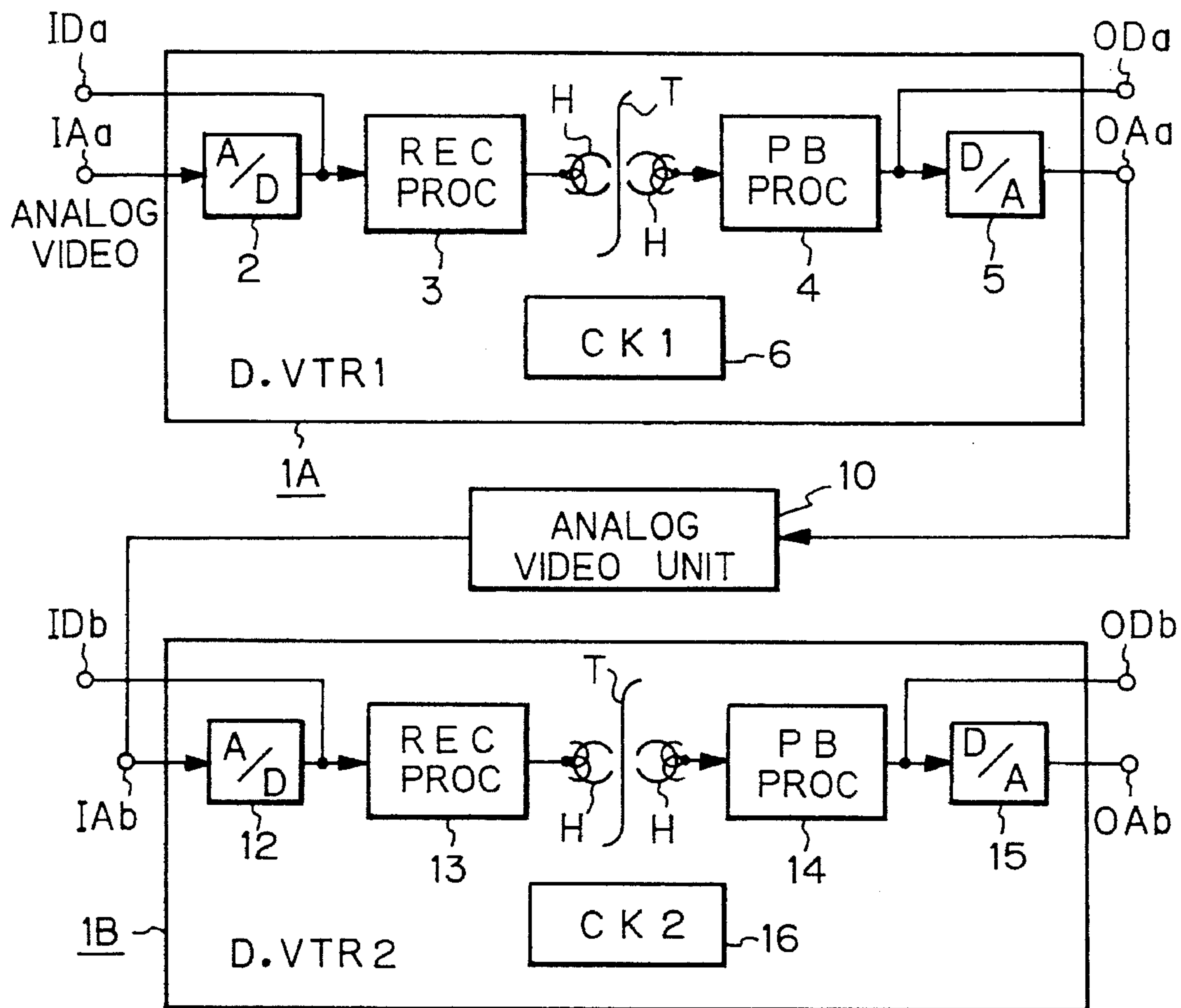
Fig. 5 (RELATED ART)
