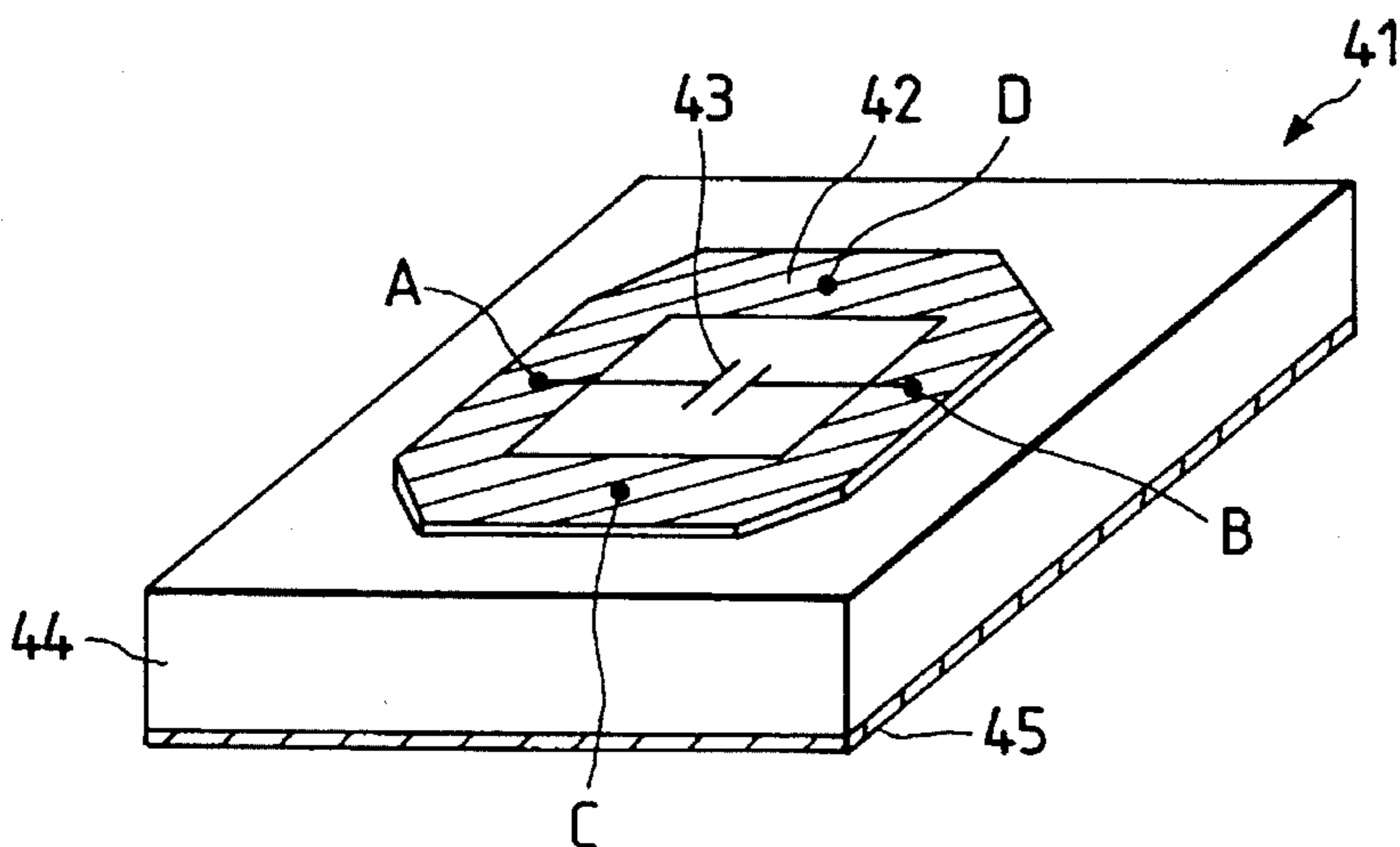
FIG. 4 PRIOR ART
