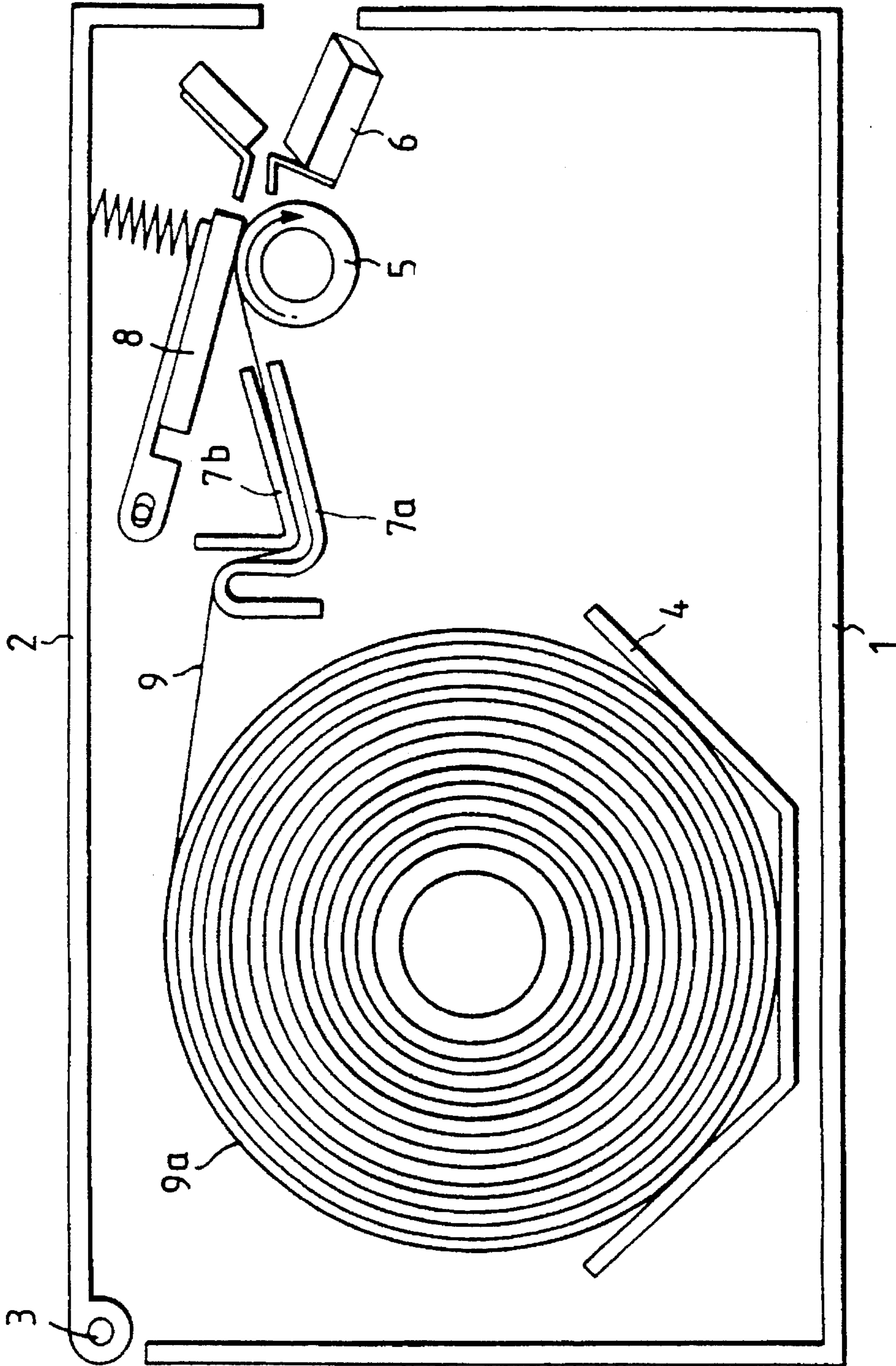
FIG. 23 PRIOR ART
