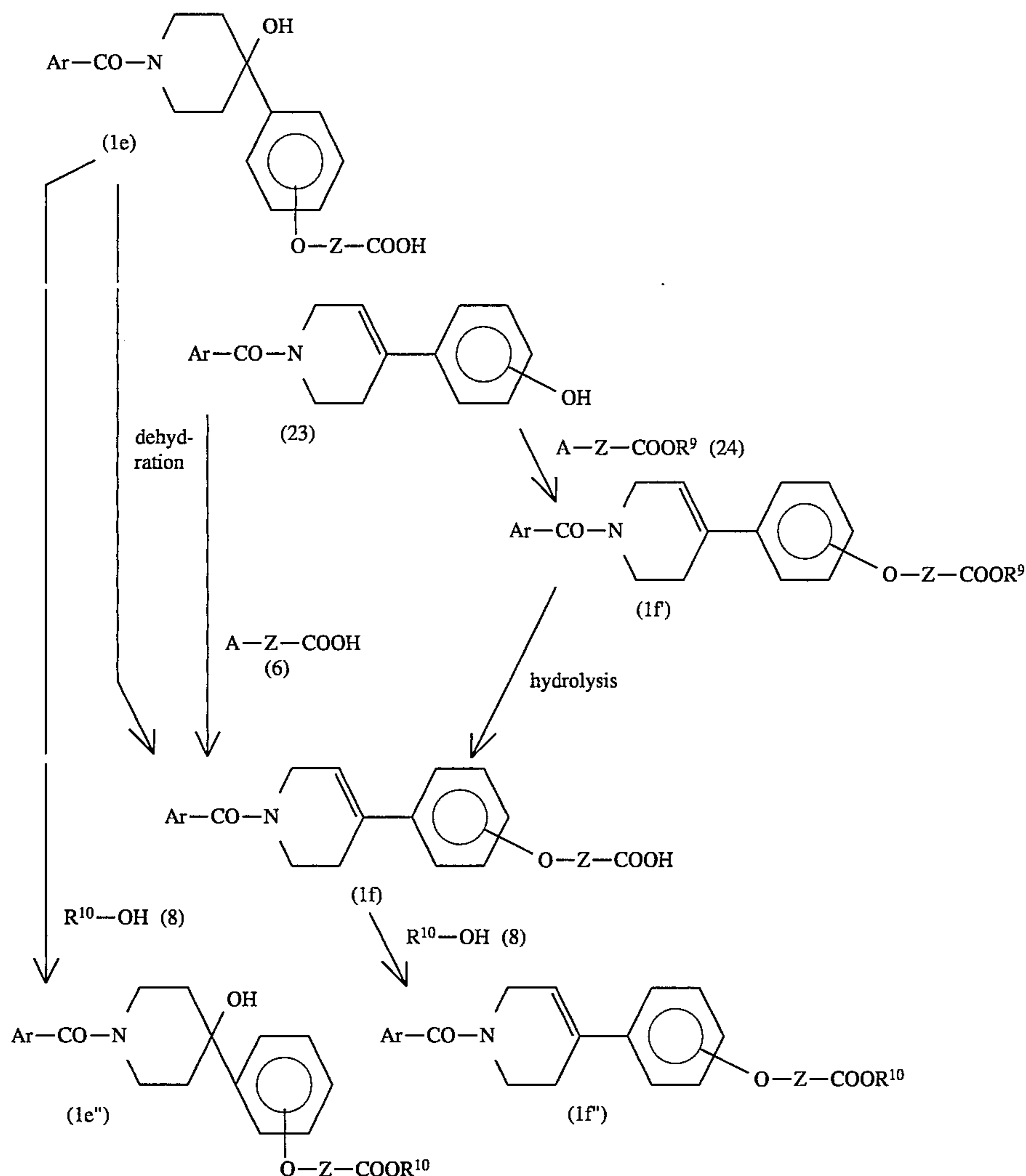
Reaction Scheme 3-2:
