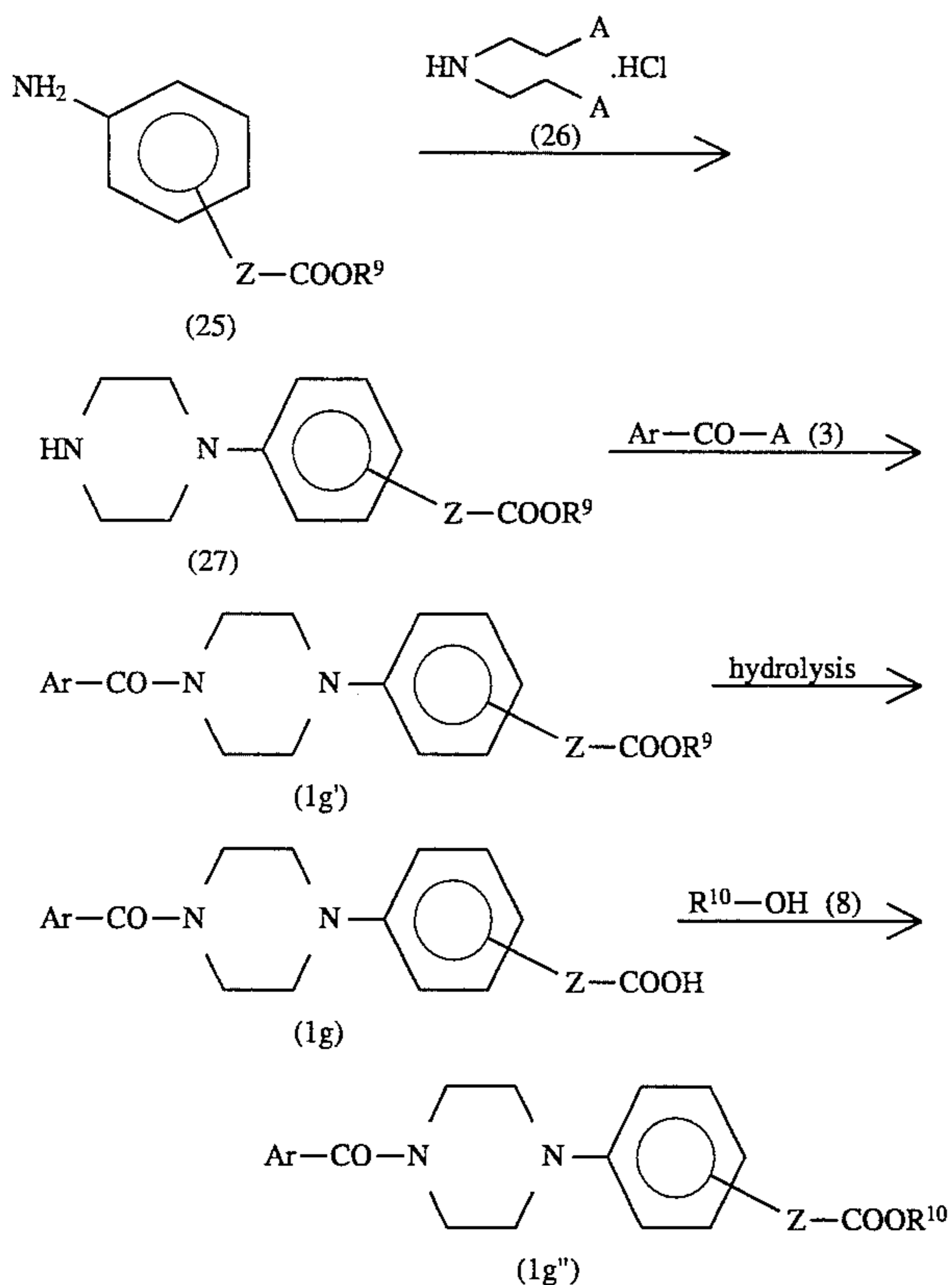
Reaction Scheme 4:
