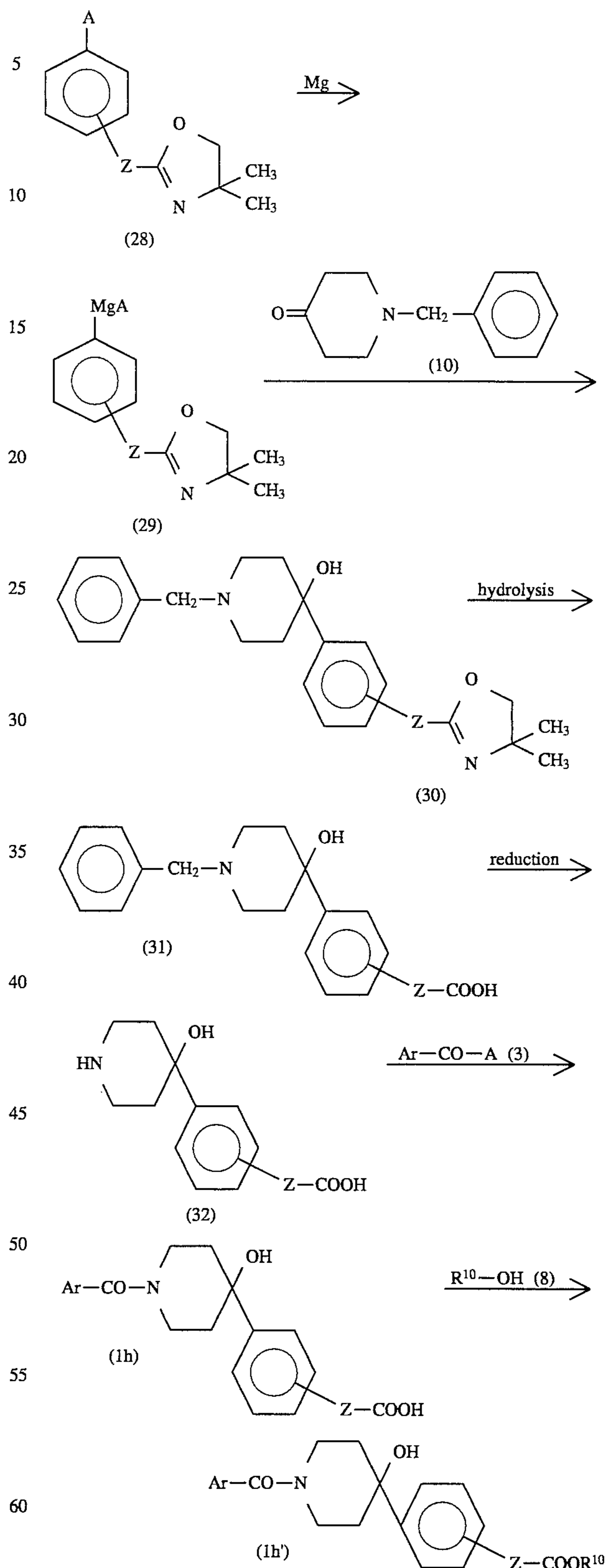
Reaction Scheme 5:
