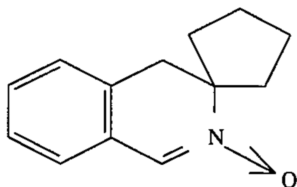
Spiro [cyclopentane-1,3']-[1H]dihydroisoquinoline 2-oxide
