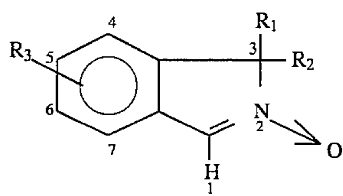
Formula I, n = 0 isoindole-N-oxide
