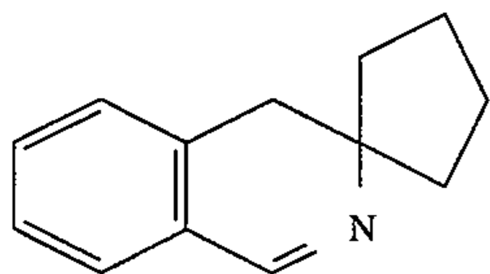
Spiro [cyclopentane-1,3']-[1H]dihydroisoquinoline
