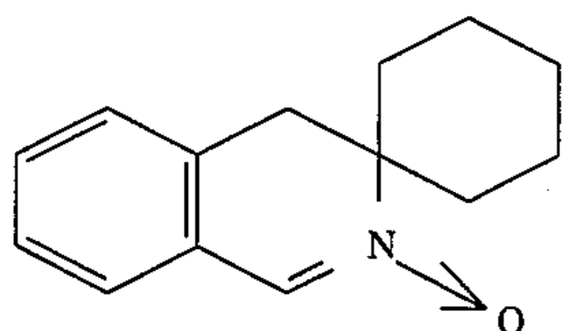
Spiro [cyclohexane-1,3']-3,4-dihydroisoquinoline-N-oxide
