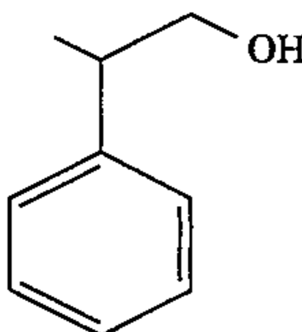
2-phenol-1-propanol
