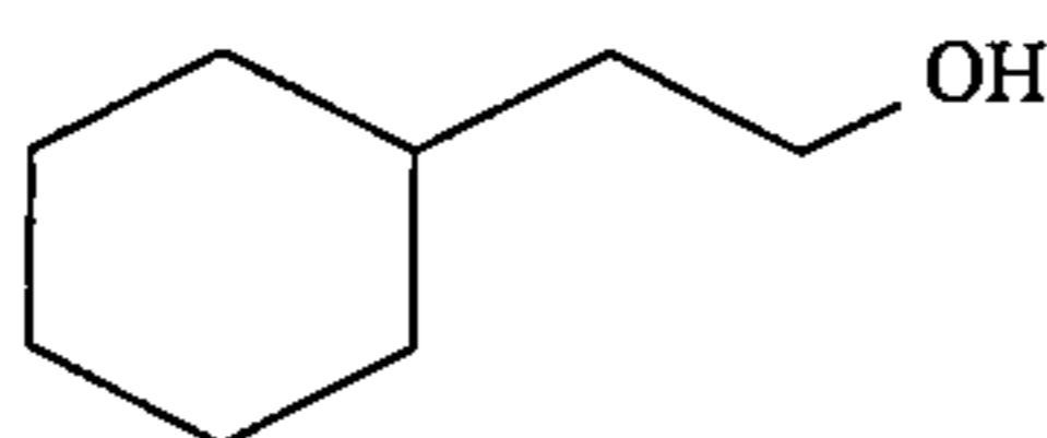
nonadyl alcohol;
