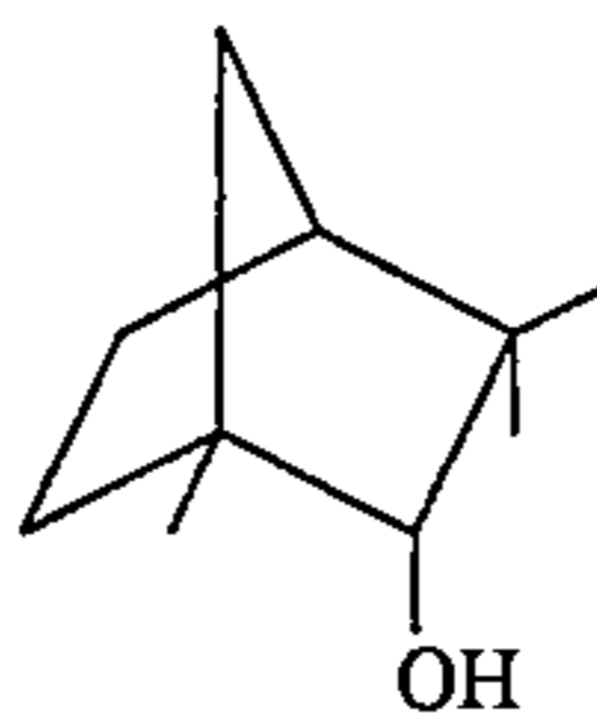
fenchol;
