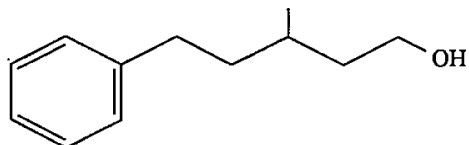
phenoxanol;
