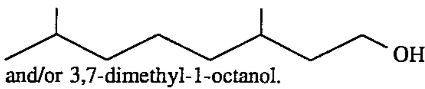
and/or 3,7-dimethyl-1-octanol.
