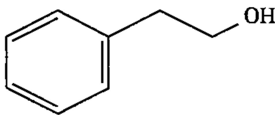
phenyl ethanol;
