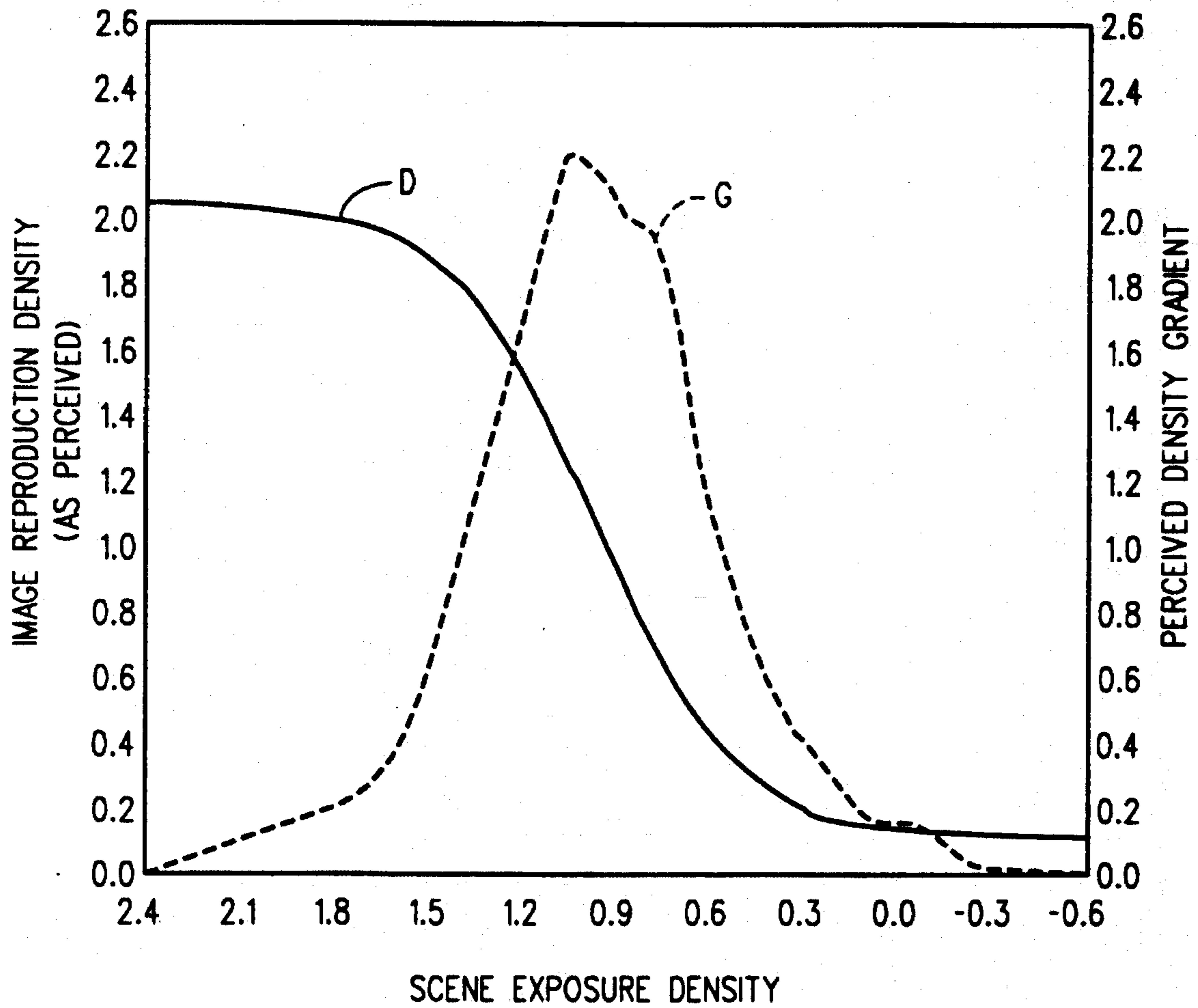
FIG. 1 PRIOR ART
