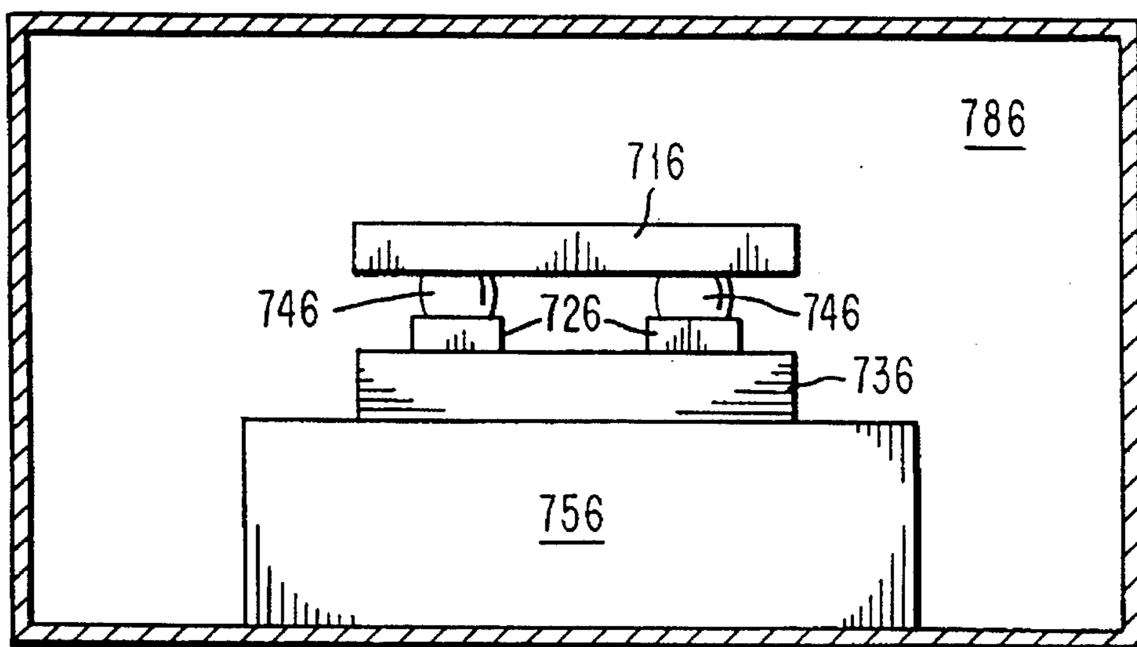
FIG. 7C PRIOR ART
