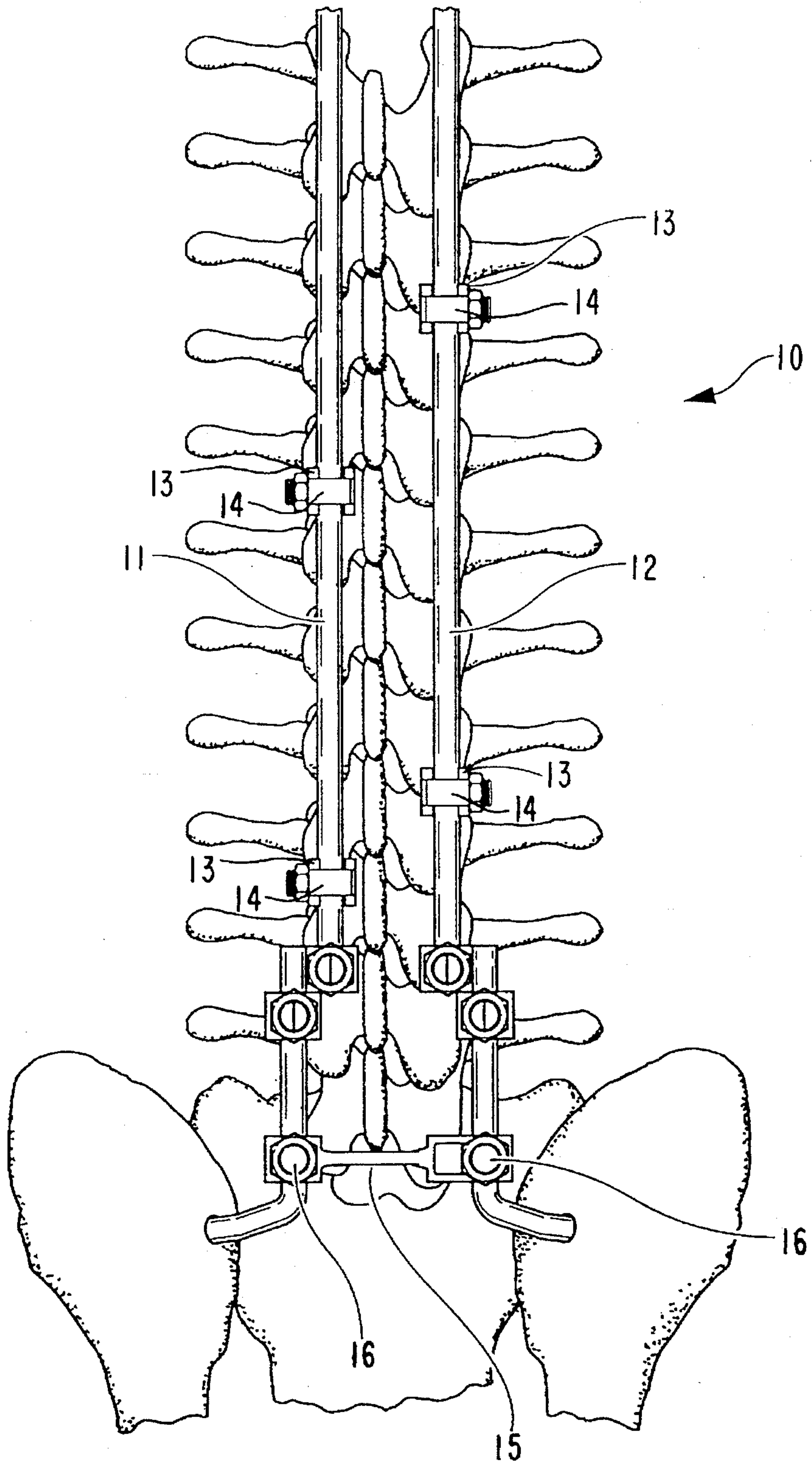
Fig. 1 (PRIOR ART)
