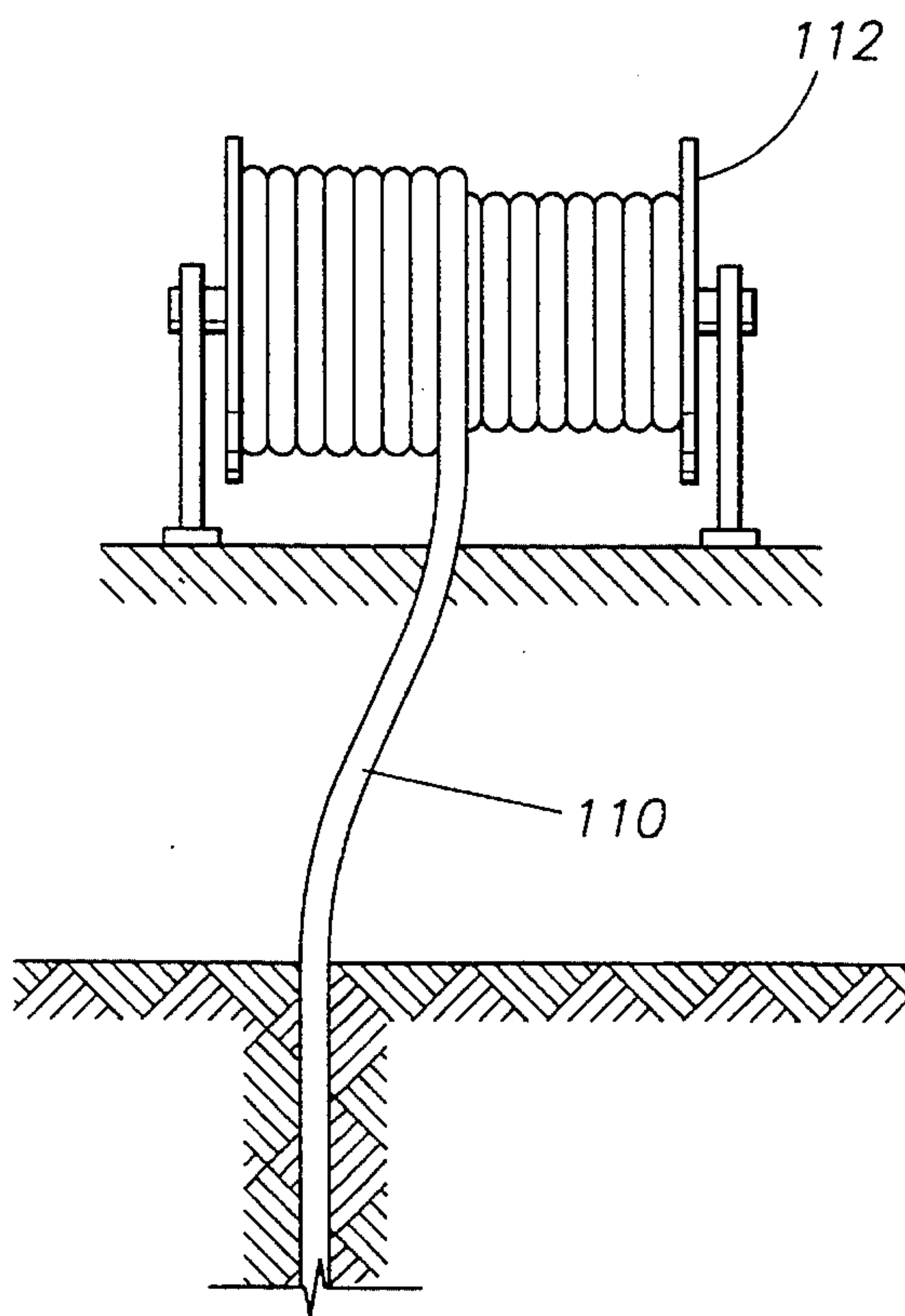
FIG. 8 (PRIOR ART)
