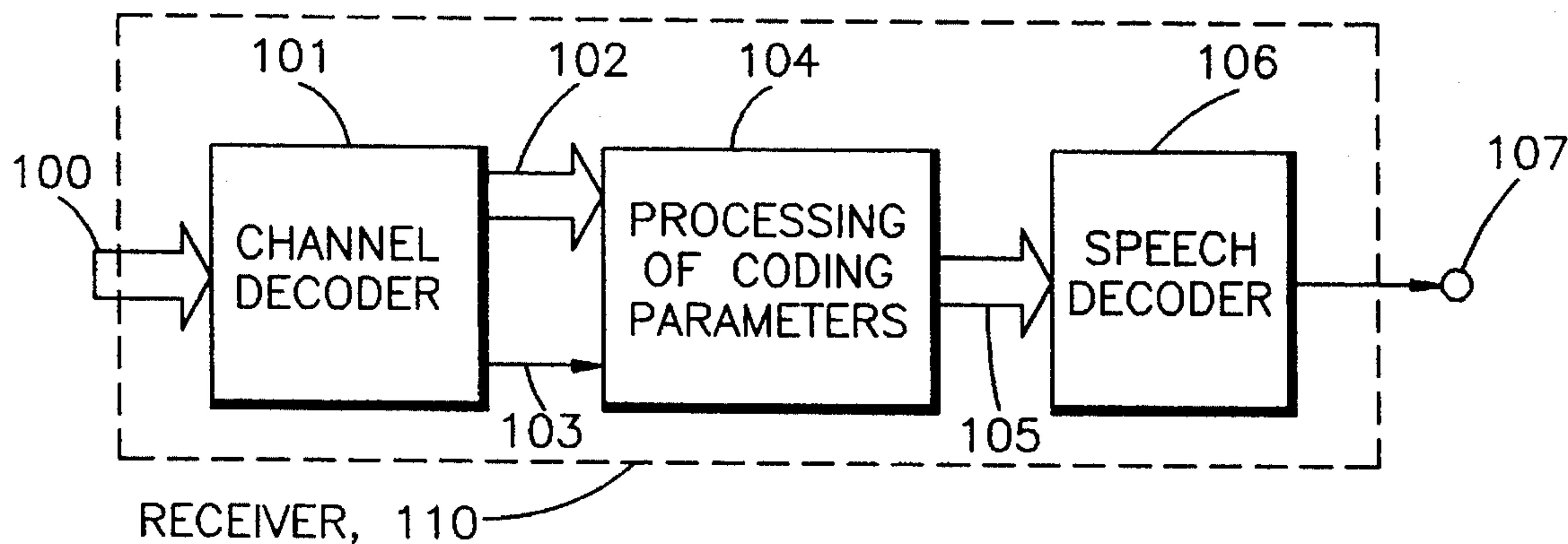
FIG. 1 PRIOR ART
