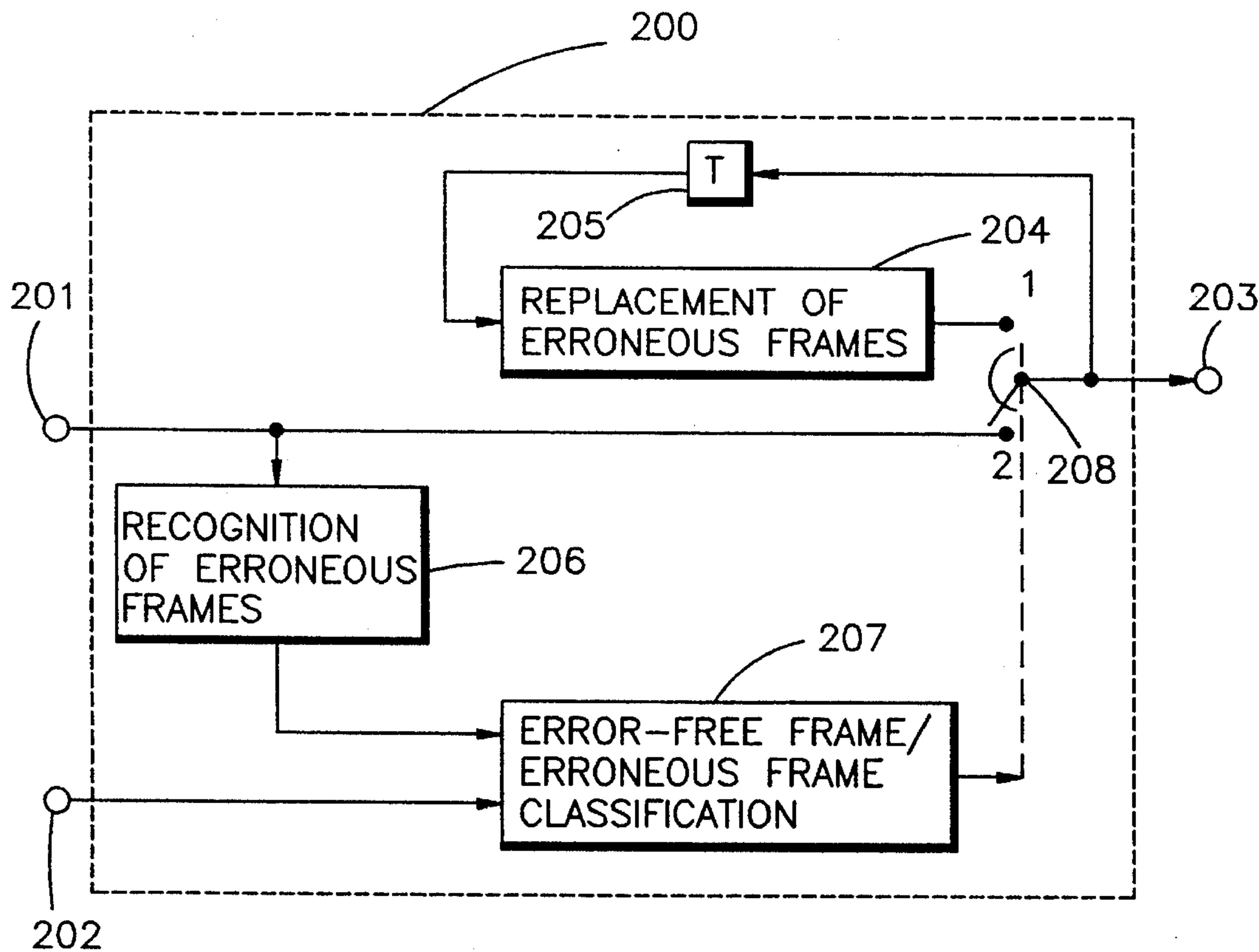
FIG. 2 PRIOR ART
