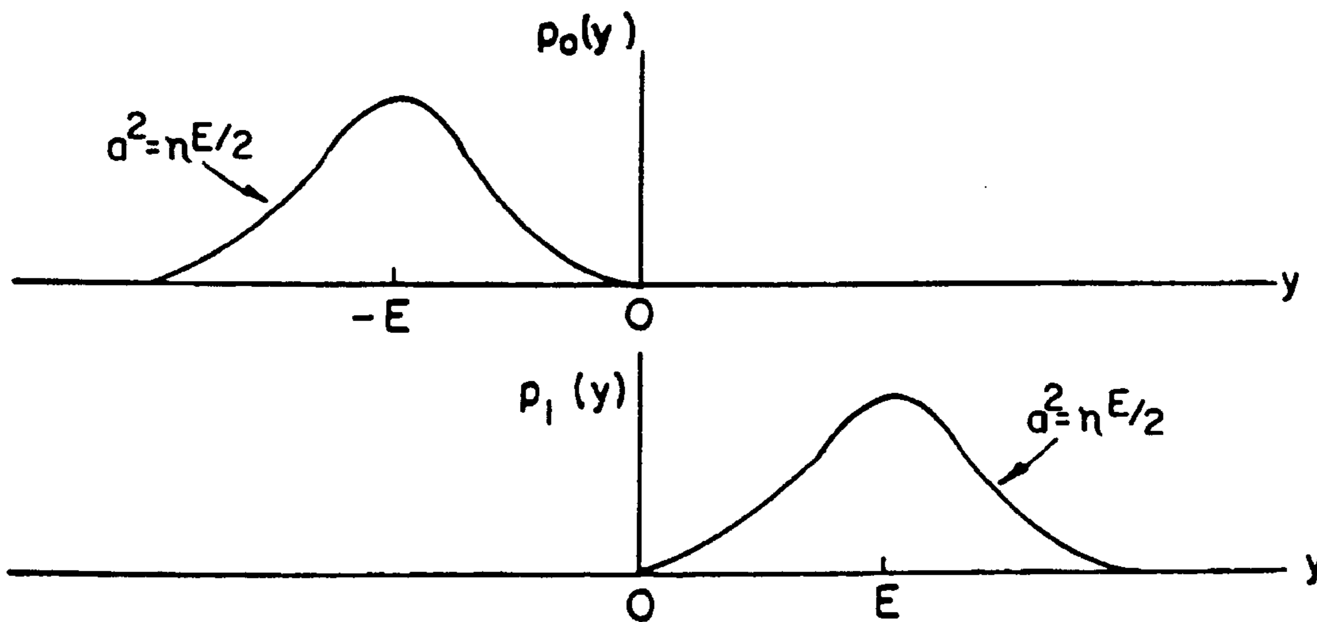
FIG. 4 PRIOR ART
