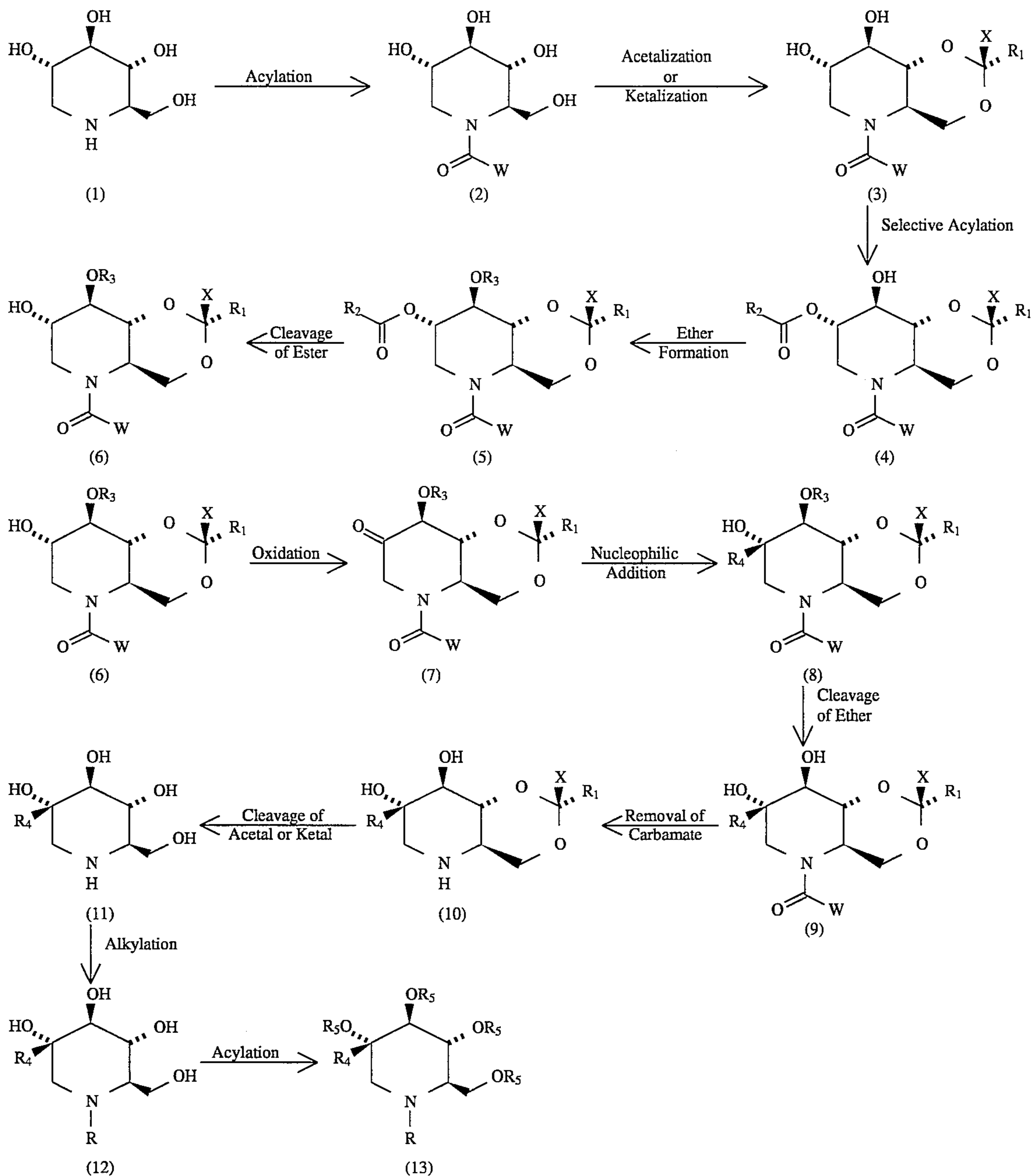
Scheme B: General Synthesis of 2-substituted tert-carbinol 1,5-iminosugars.
