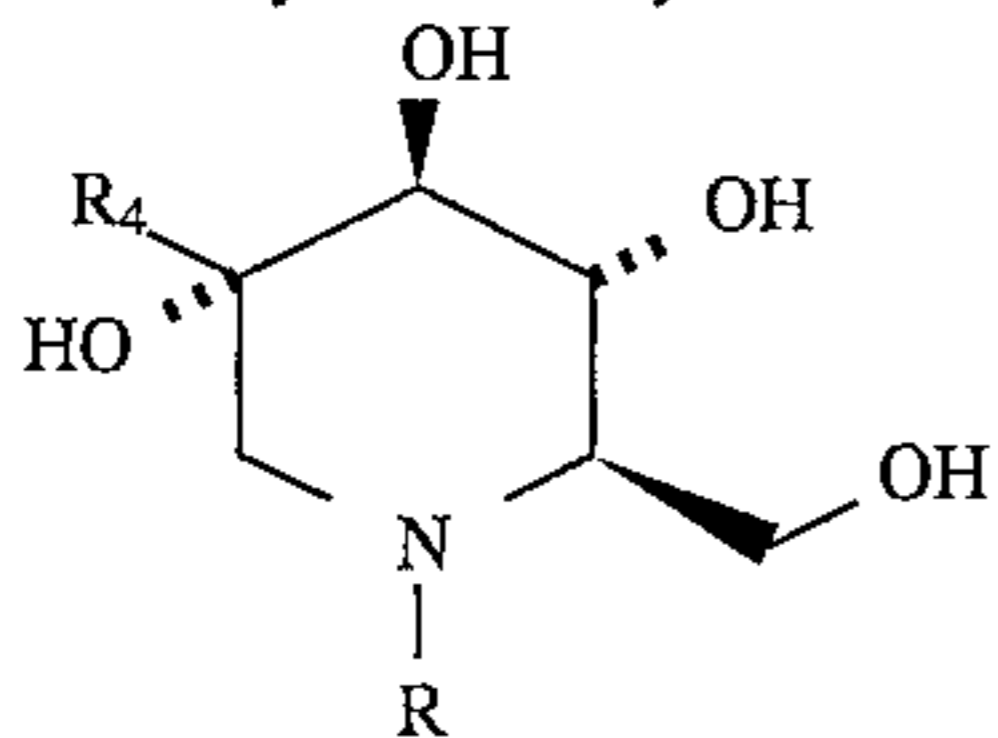
Anti HIV Activity of 2-Methyl Carbinol Analogs
