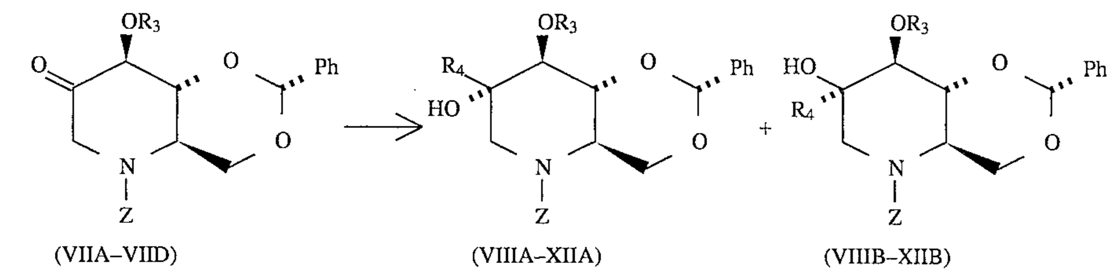
Scheme E: Nucleophilic Additions to 2-Ketone
