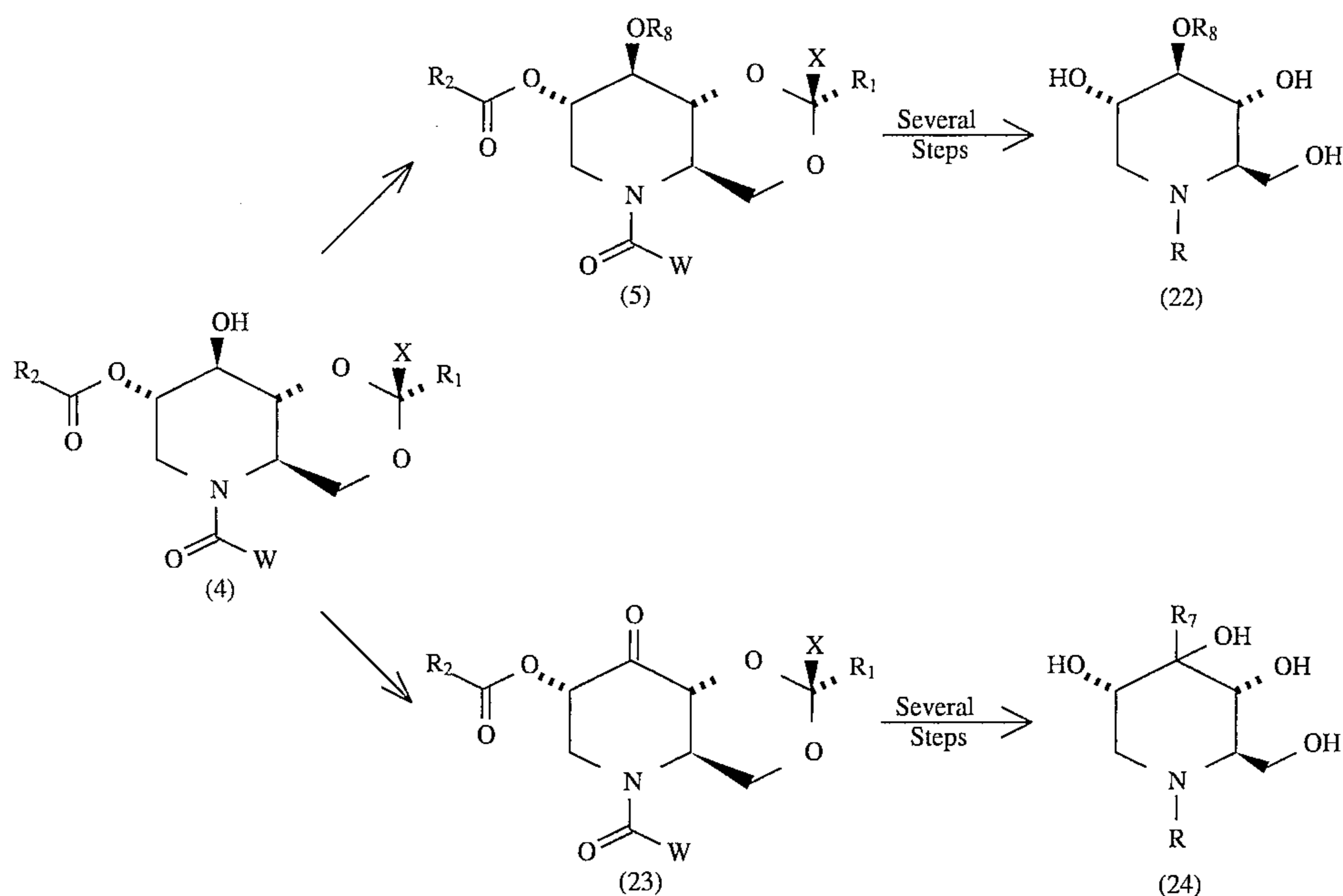
Scheme I: Generic Synthesis of 3-substituted 1,5-iminosugars
