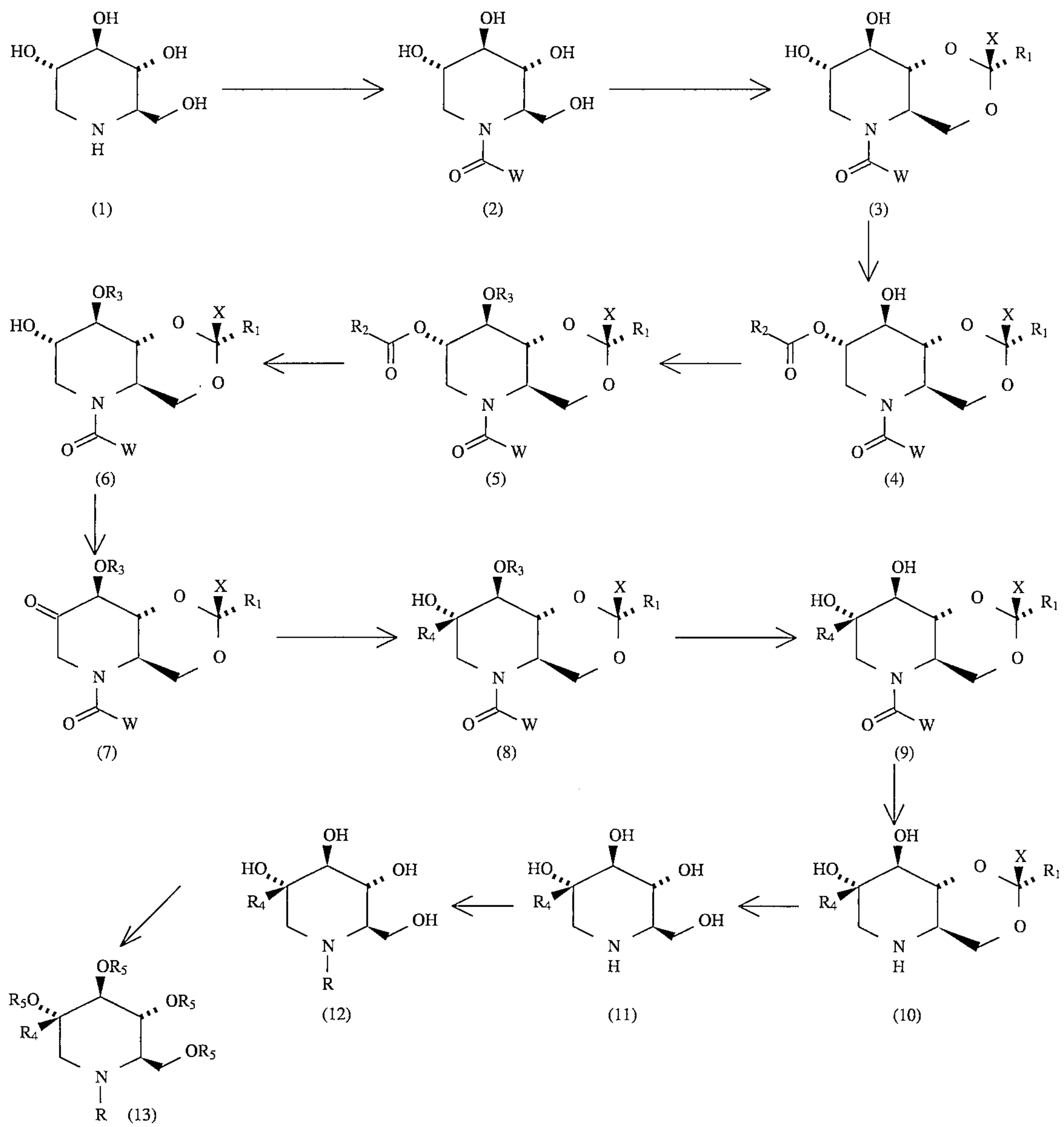
Scheme A: Generic Synthesis of 2-substituted tert-carbinol 1,5-iminosugars.
