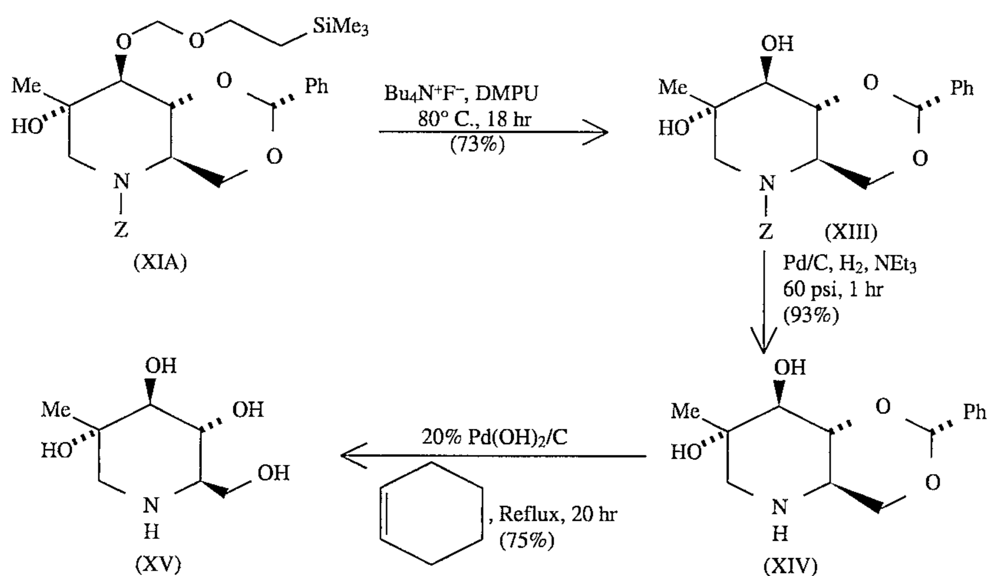
Scheme F: Synthesis of 2-Methyl Carbinols
