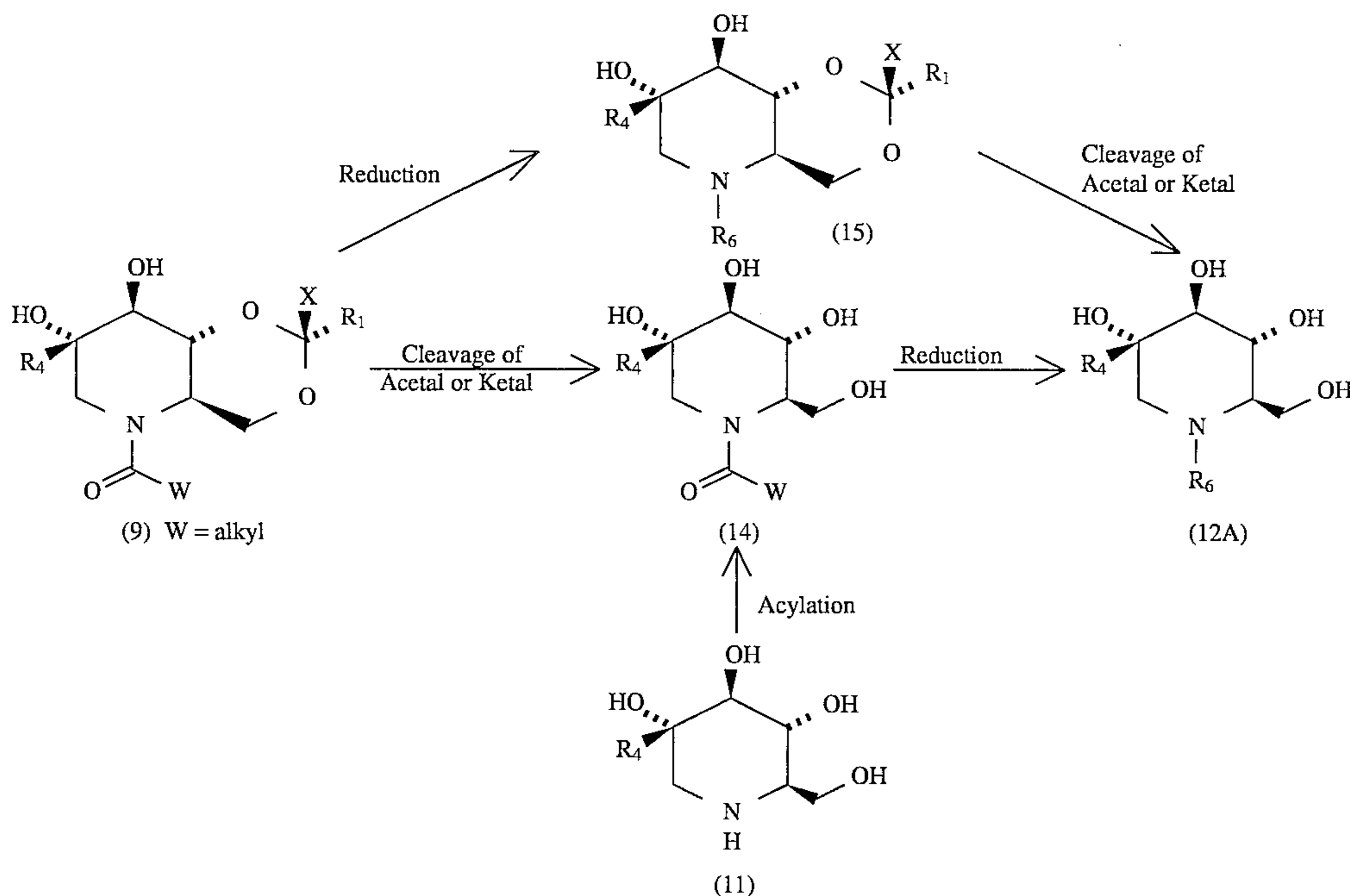
Scheme C: Additional Synthesis of 2-substituted tert-carbinol 1,5-imino sugars
