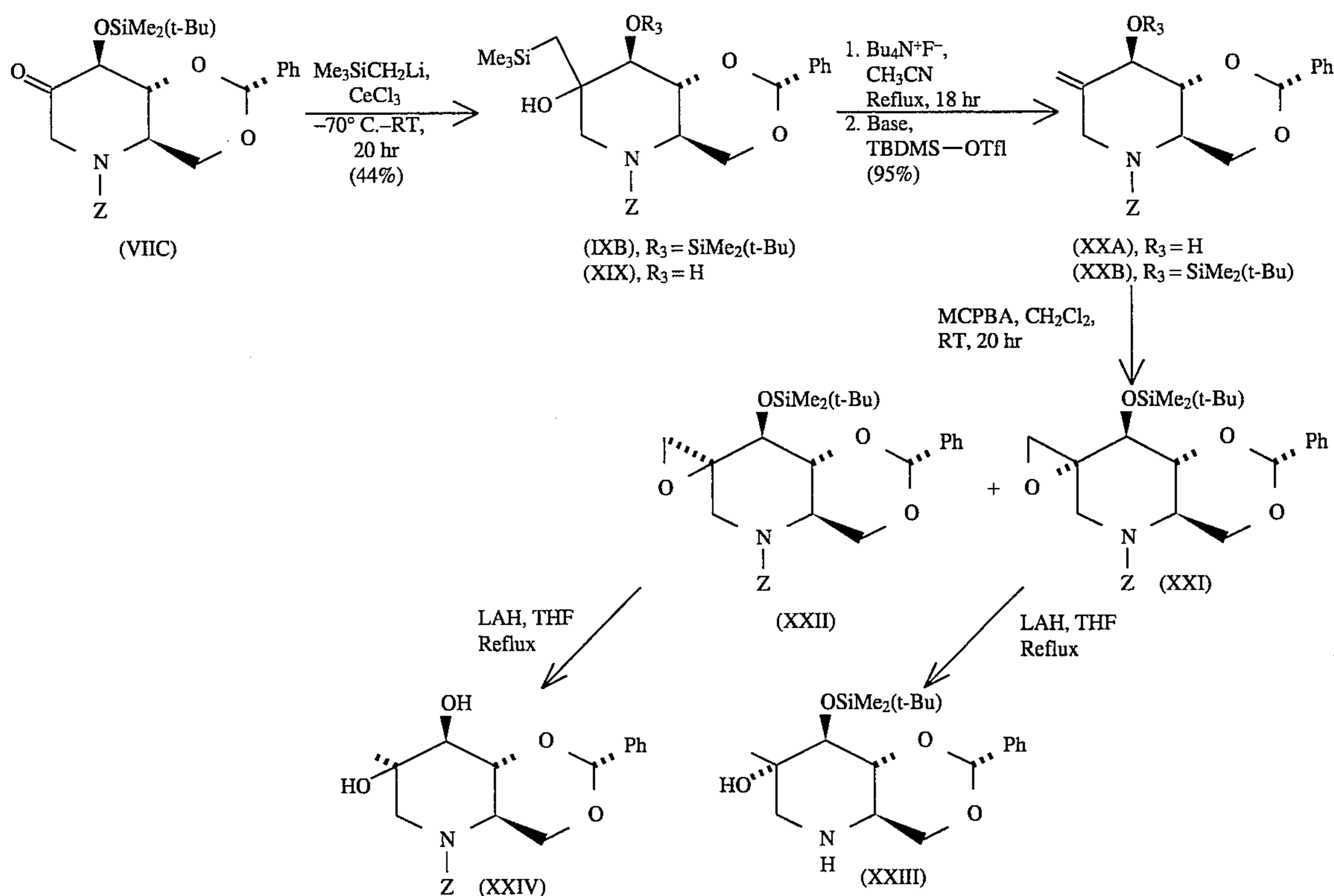
Scheme H: Synthesis of 2-Methyl Carbinol by Epoxide Opening
