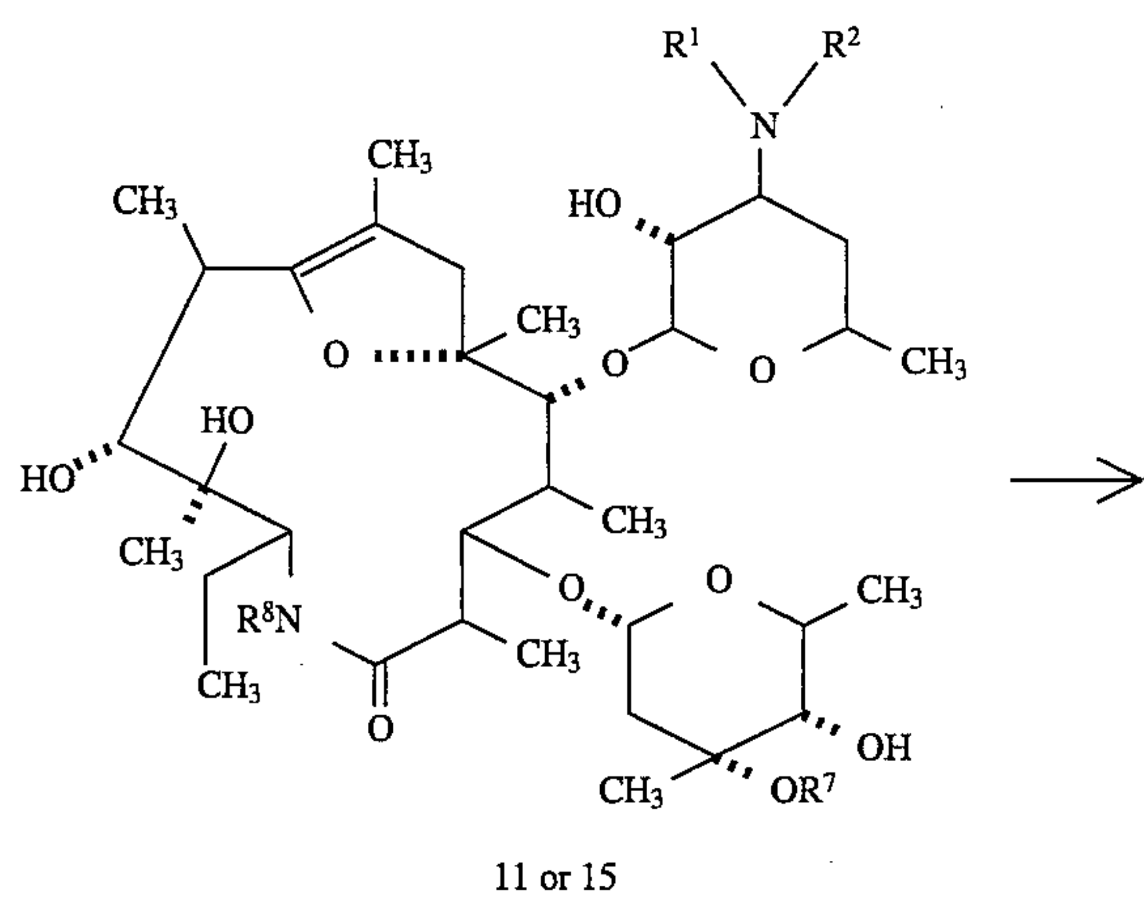
Scheme V
