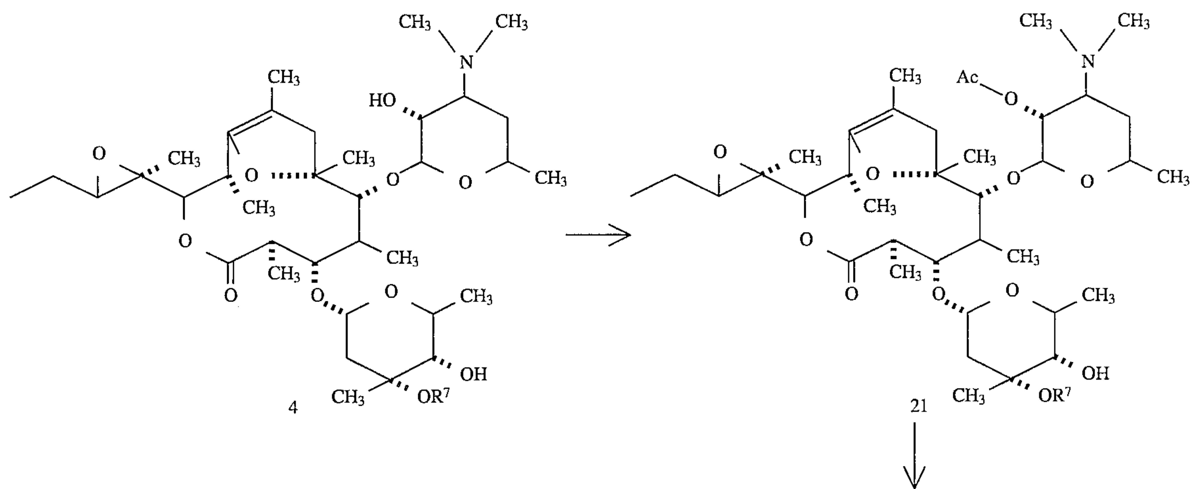
Scheme VIII
