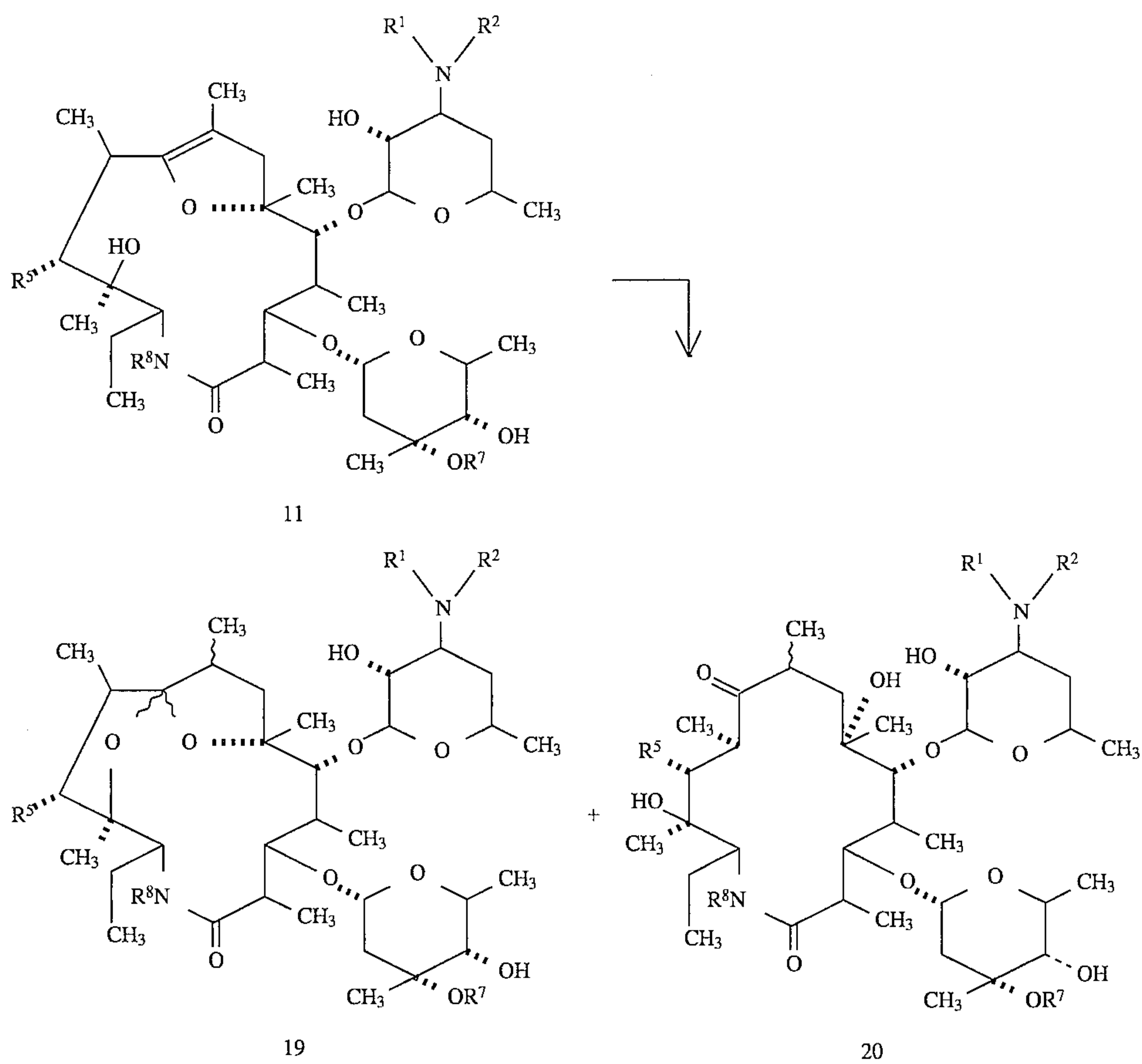
Scheme VII
