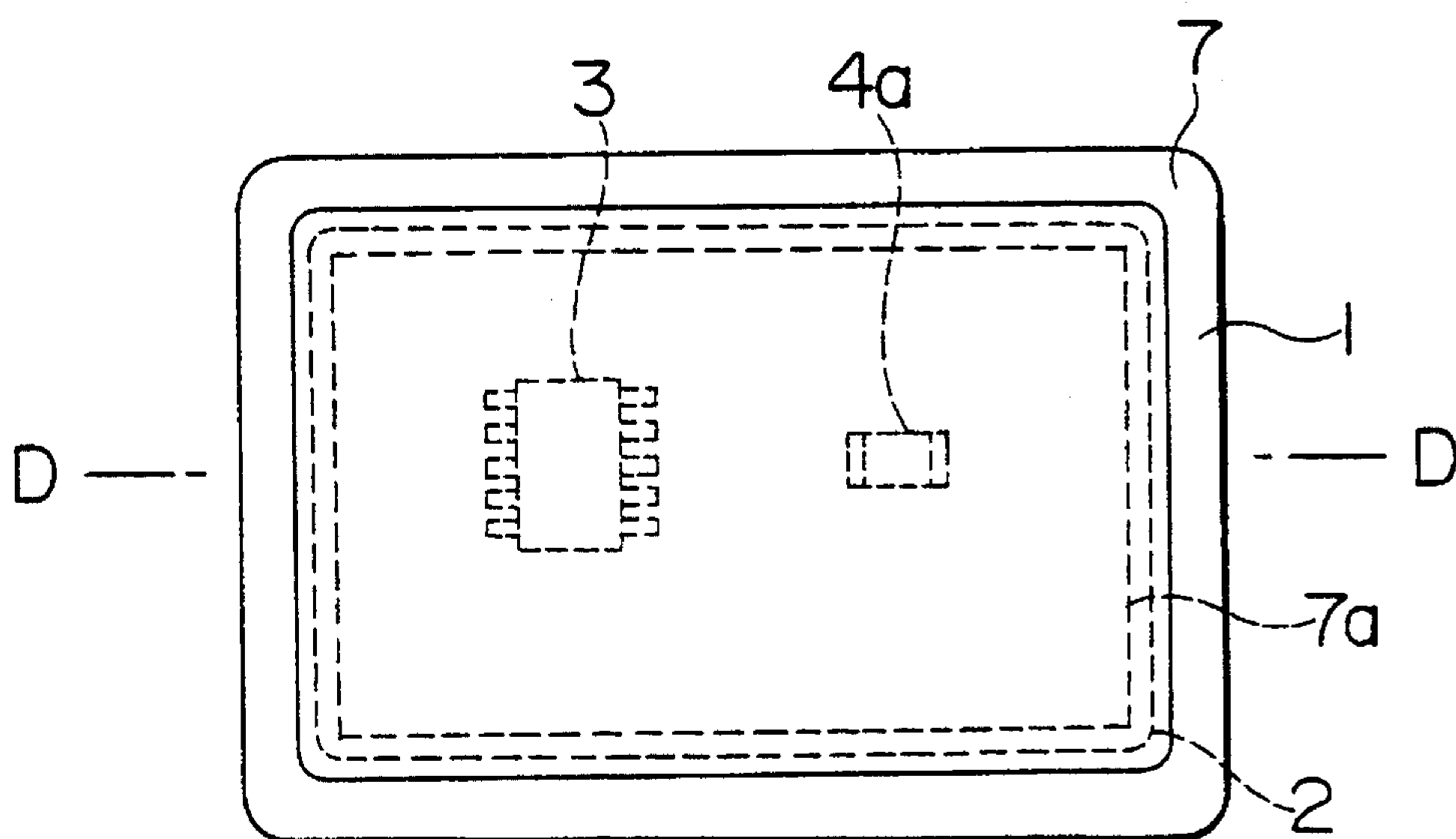
FIG. 51 PRIOR ART
