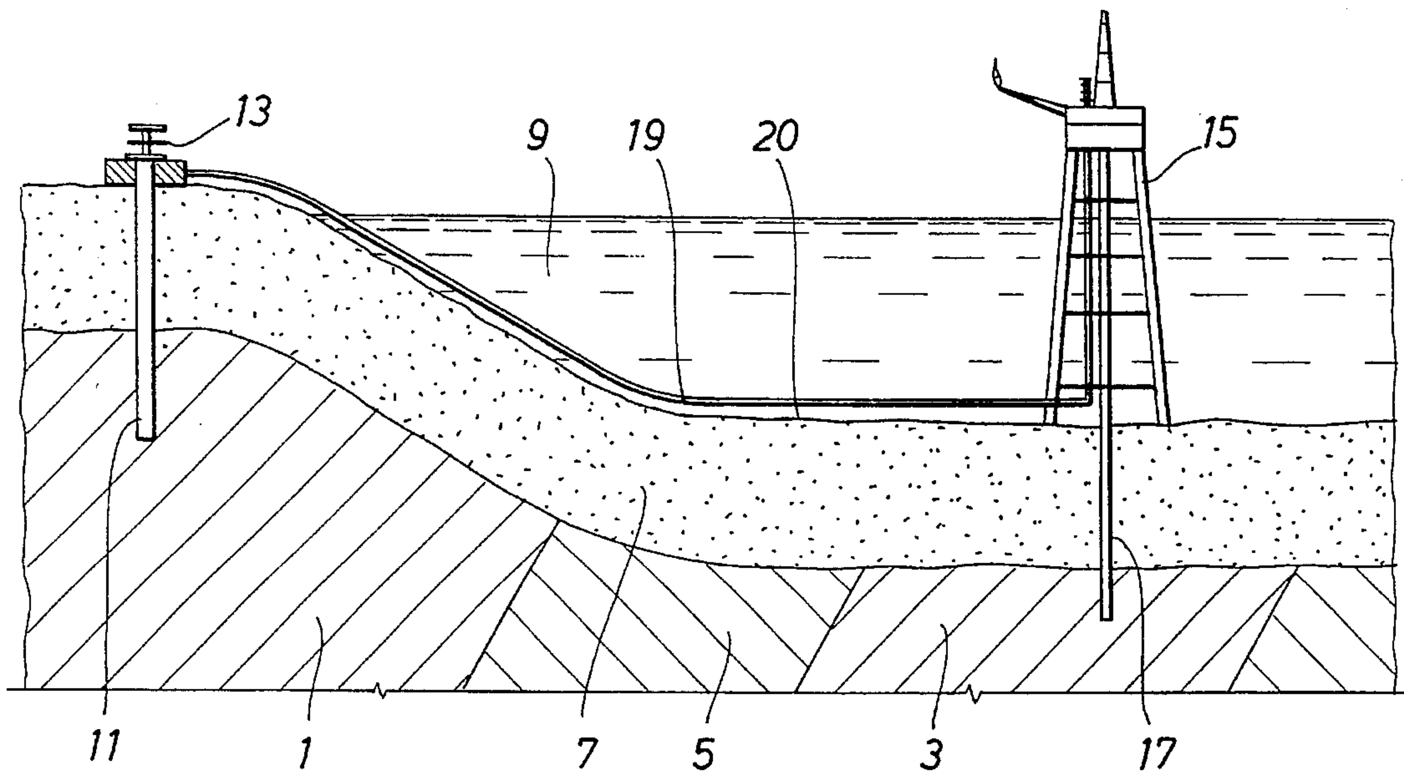
FIG. 1 (PRIOR ART)
