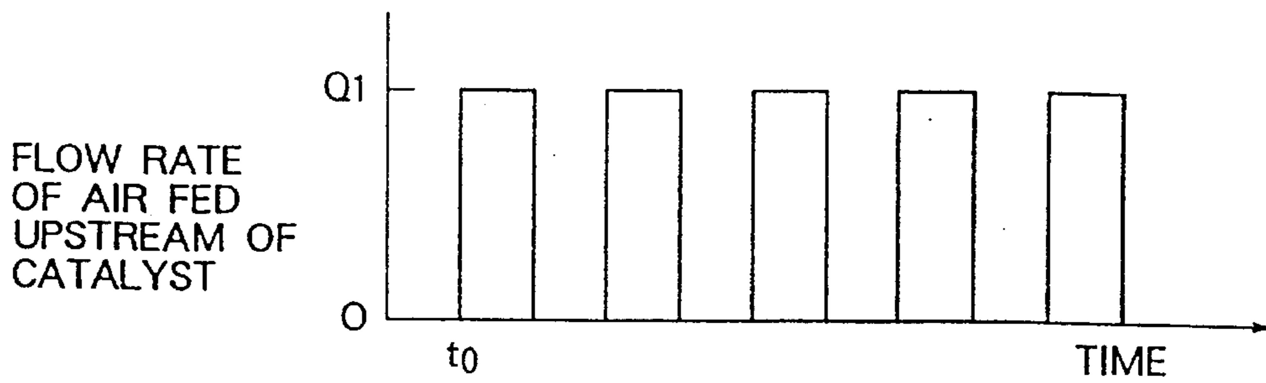
FIG. 18(A)
