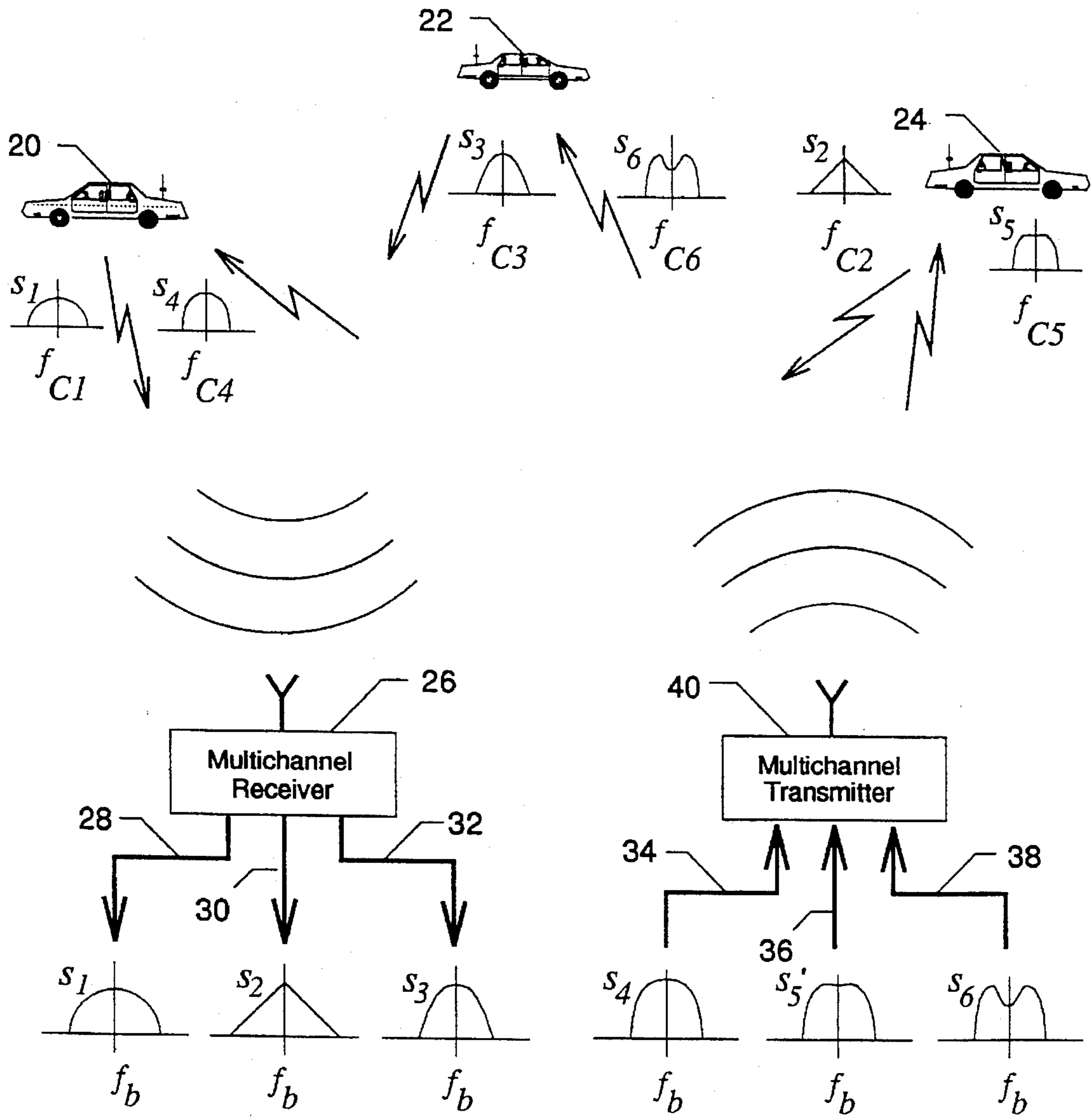
FIG. 1 PRIOR ART
