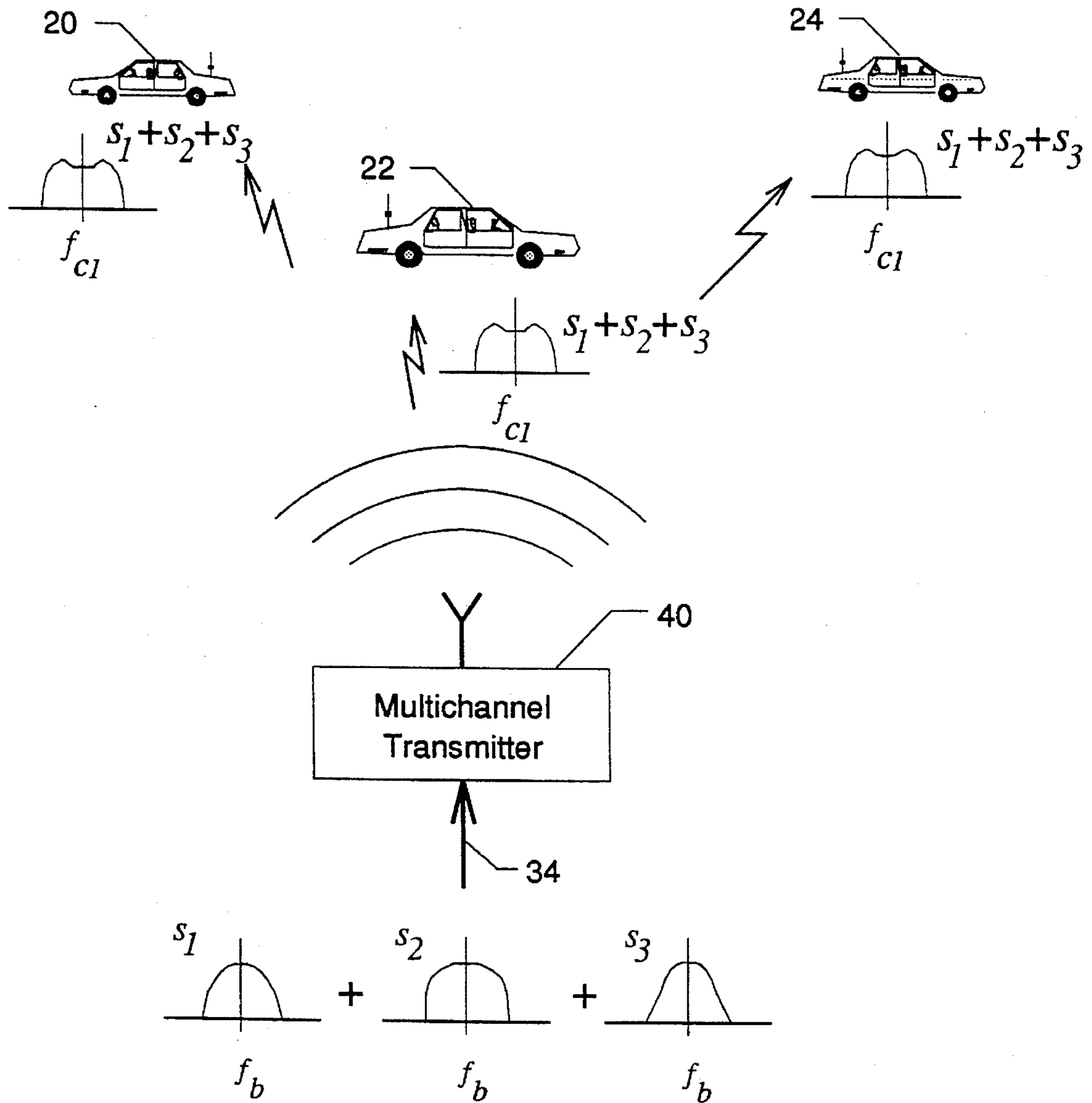
FIG. 3 PRIOR ART
