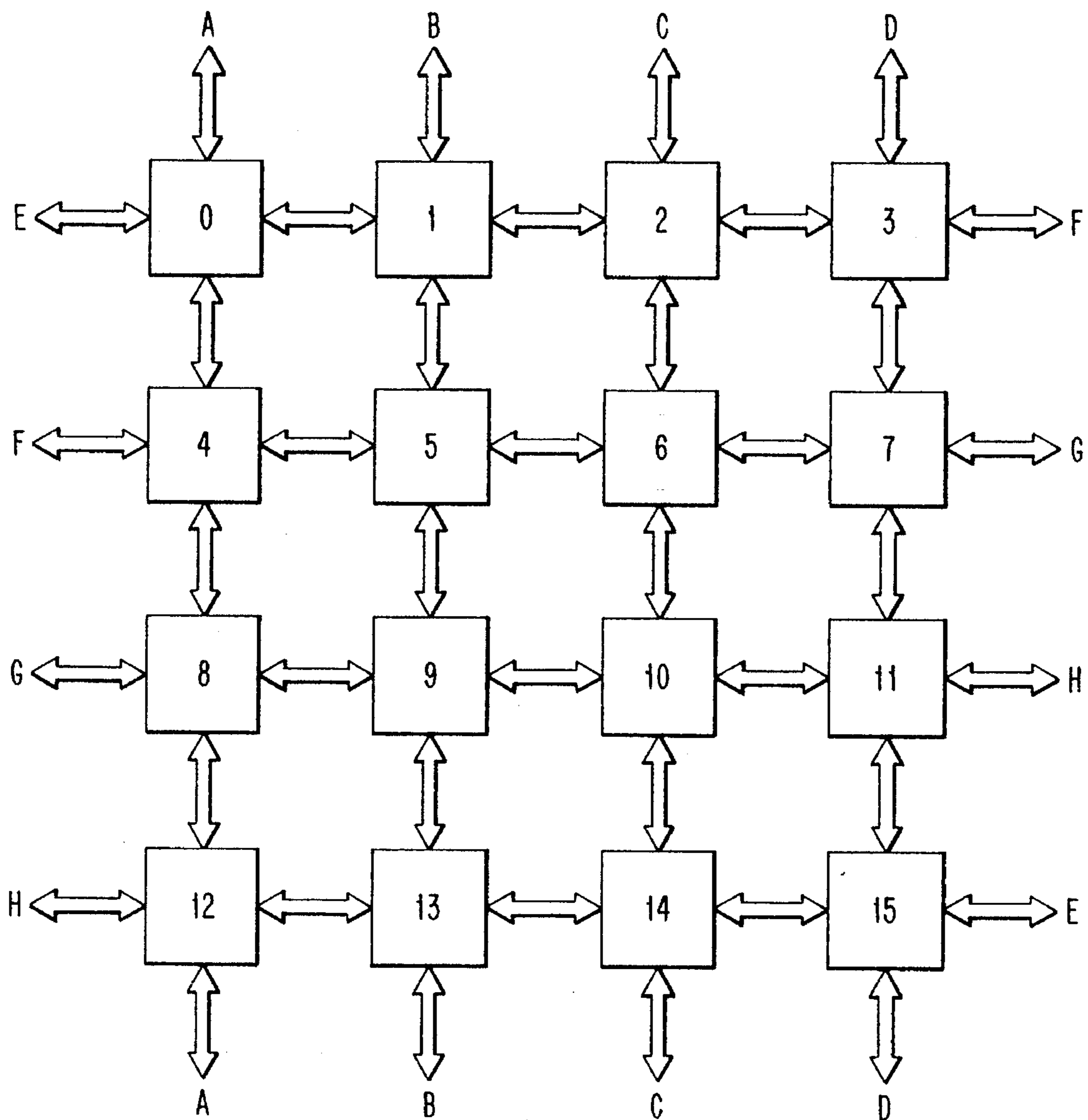
FIG. 2 (PRIOR ART)
