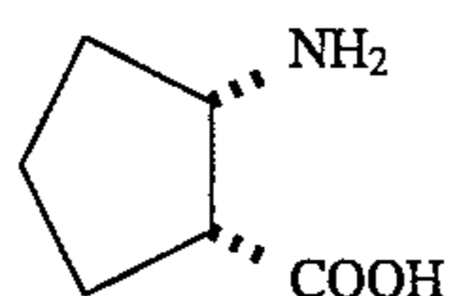
[(1R, 2S)-2-aminocyclopentanecarboxylic acid]
