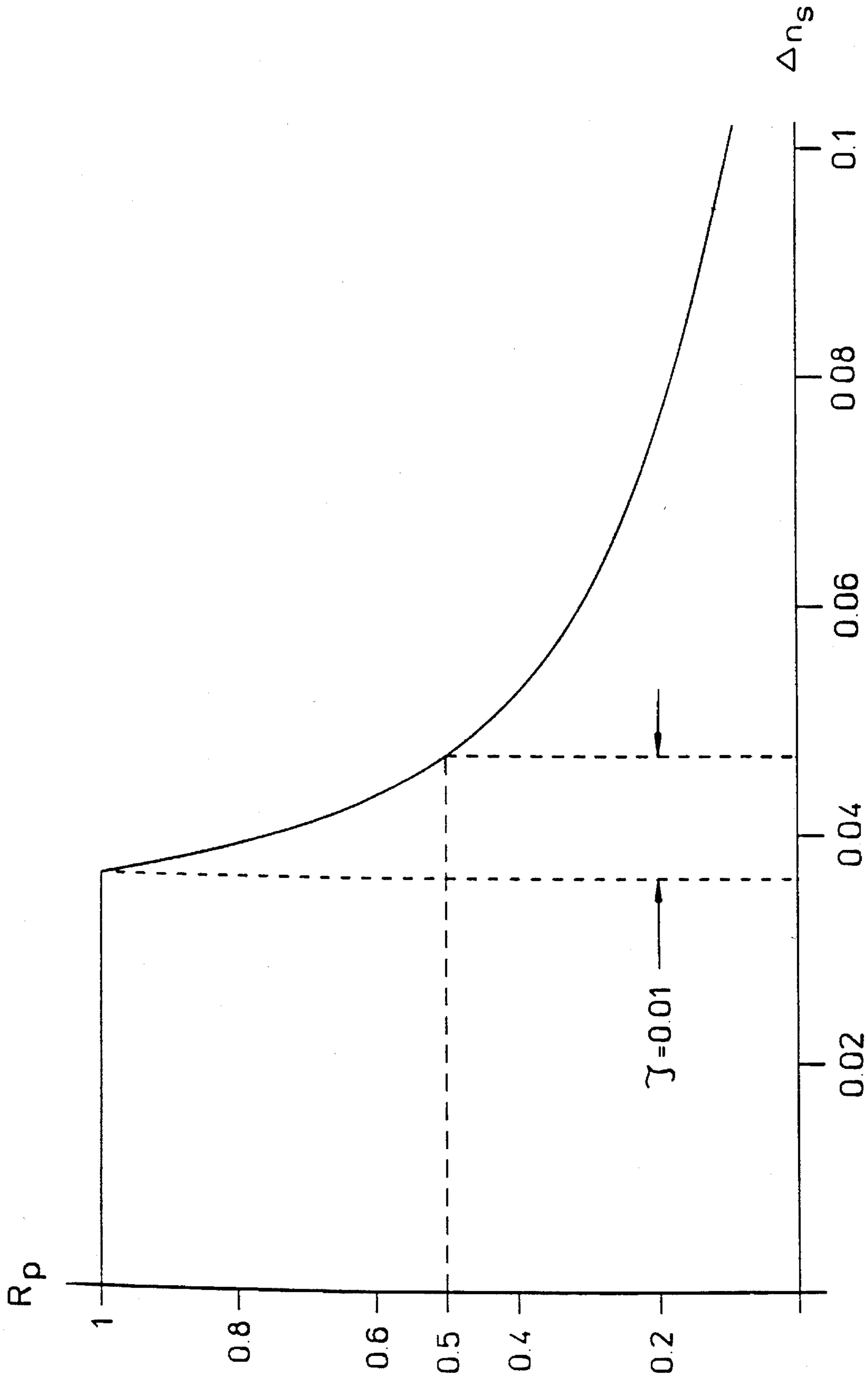
FIG. 6 (PRIOR ART)
