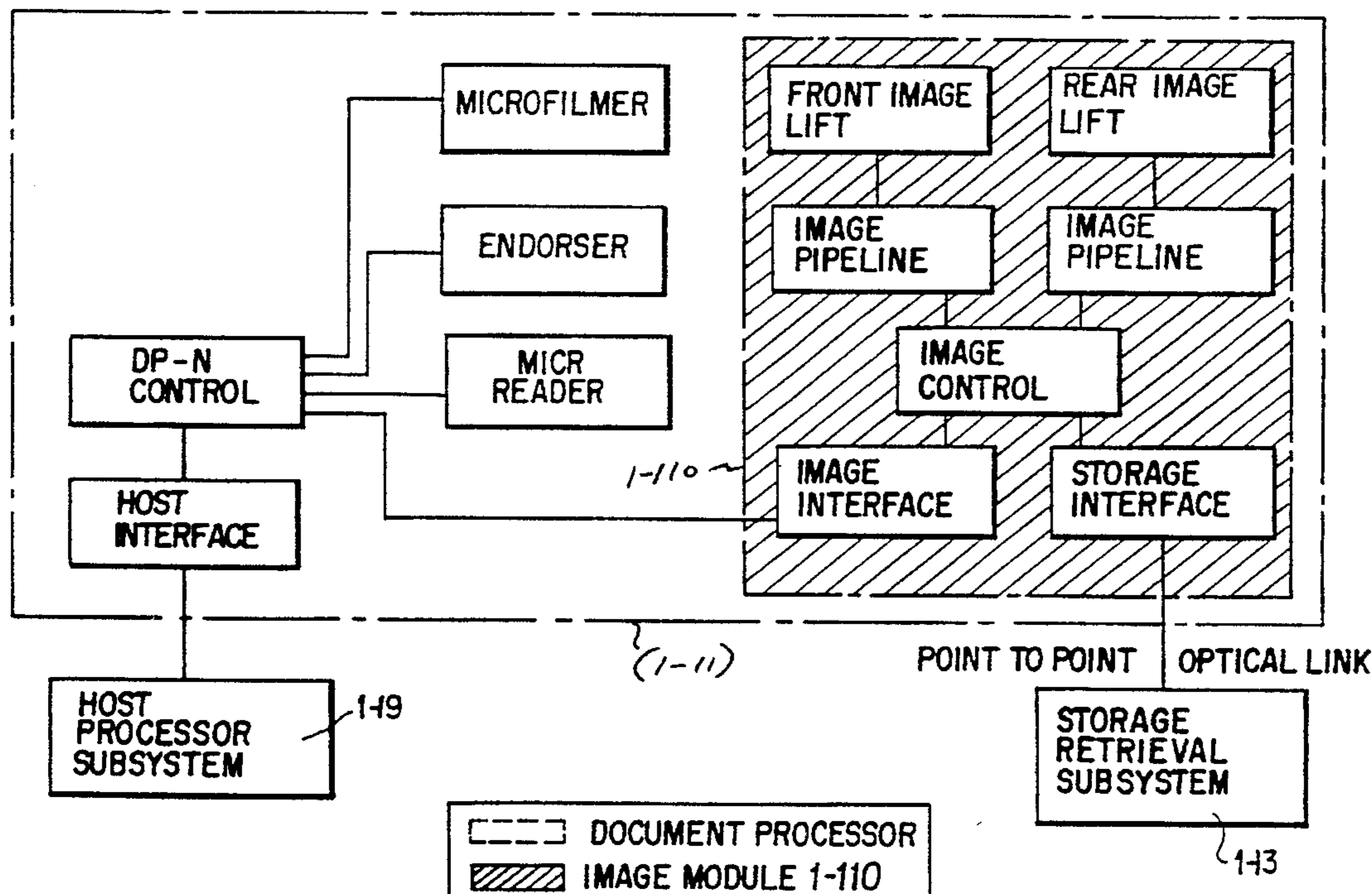
DOCUMENT PROCESSOR SUBSYSTEM FUNCTIONS
