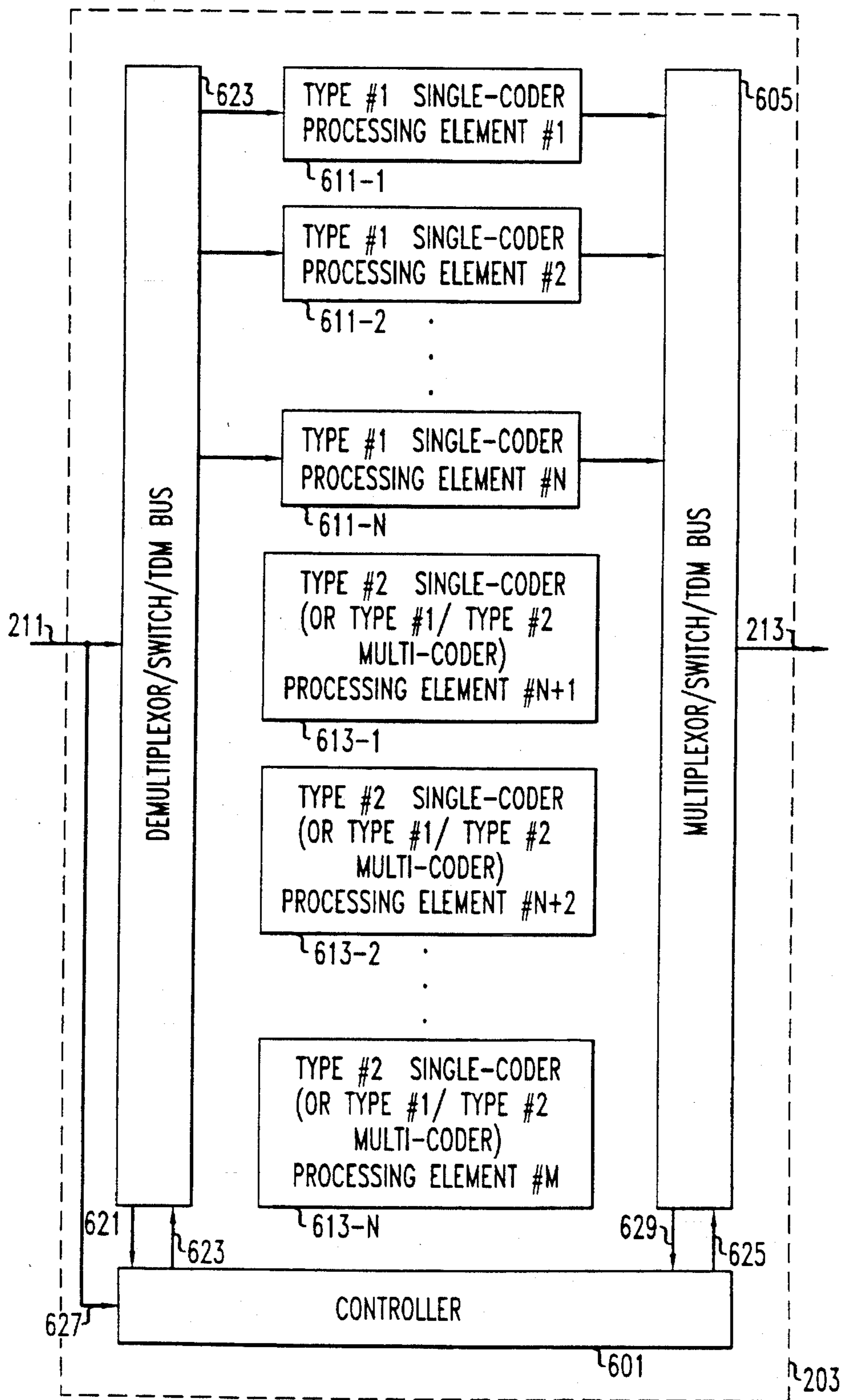
FIG. 6 (HALF-DUPLEX ARCHITECTURE)
