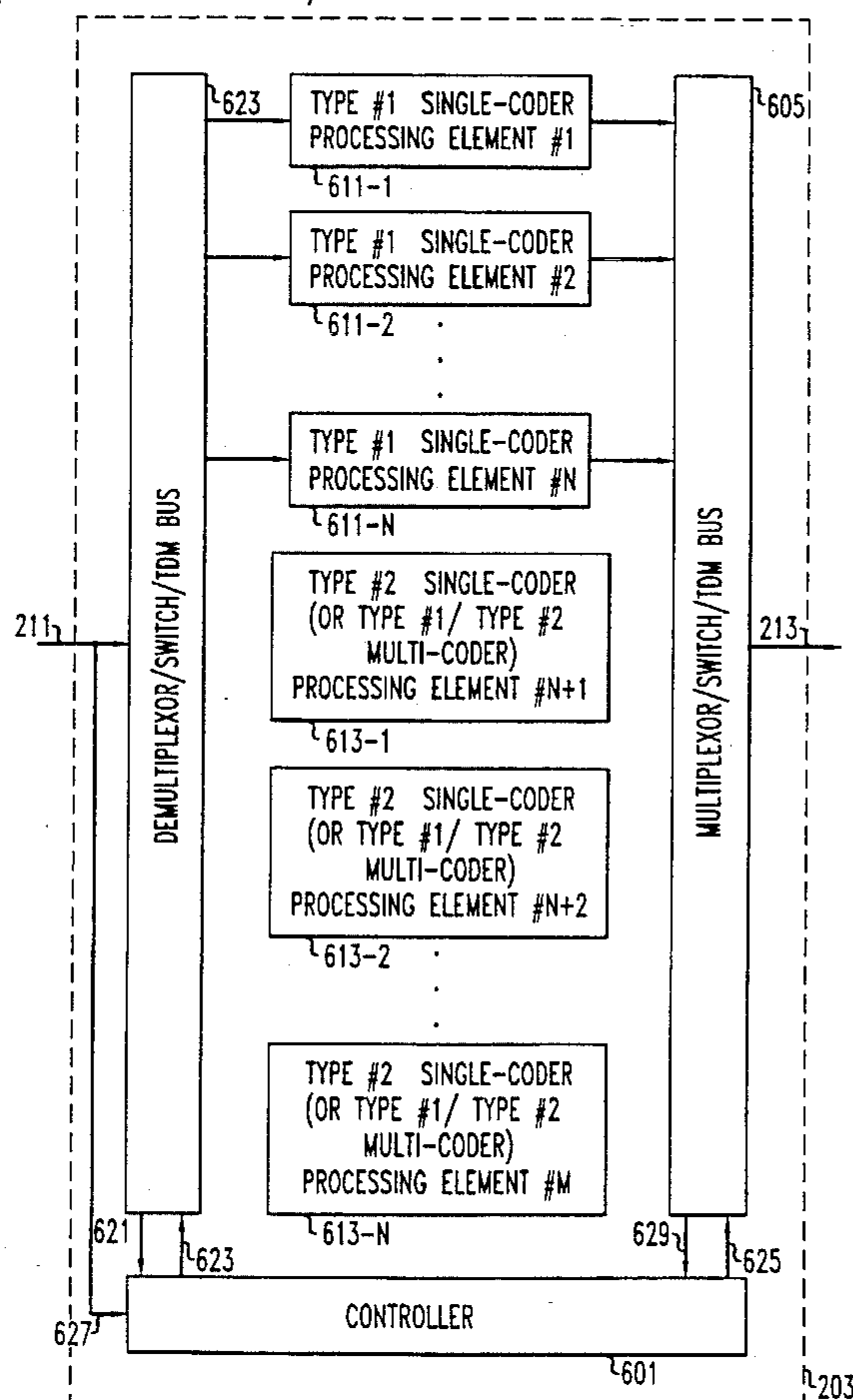
(HALF-DUPLEX ARCHITECTURE)
