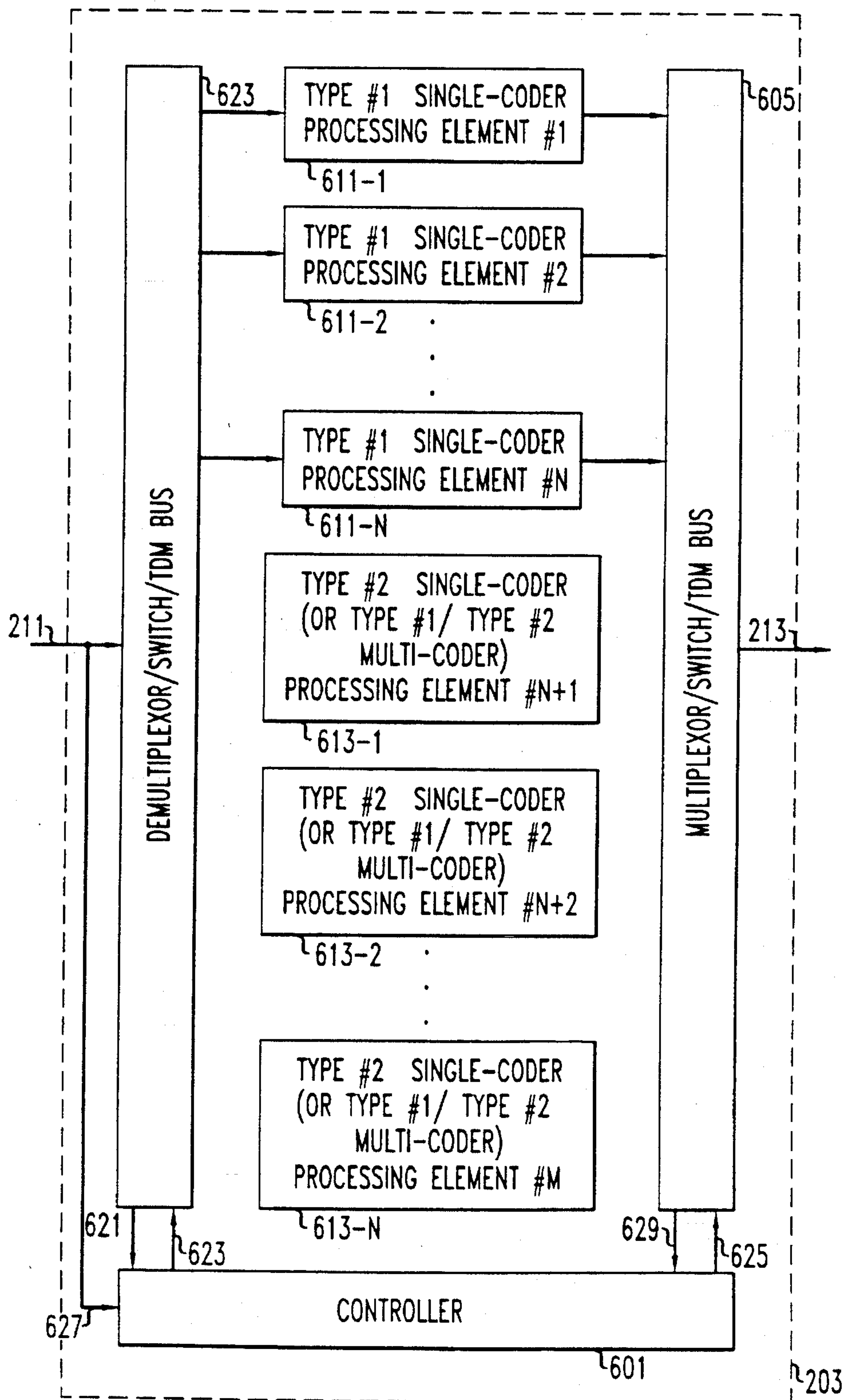
FIG. 6 (HALF-DUPLEX ARCHITECTURE)
