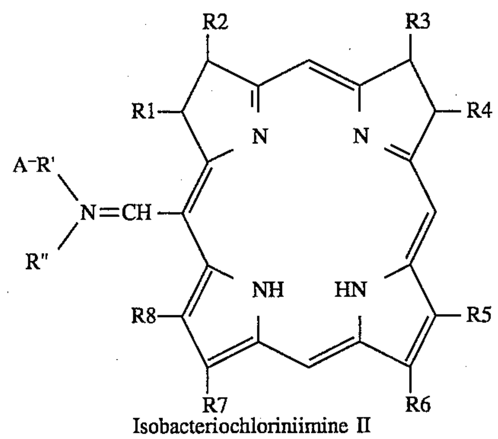
Isobacteriochlorinimine I
