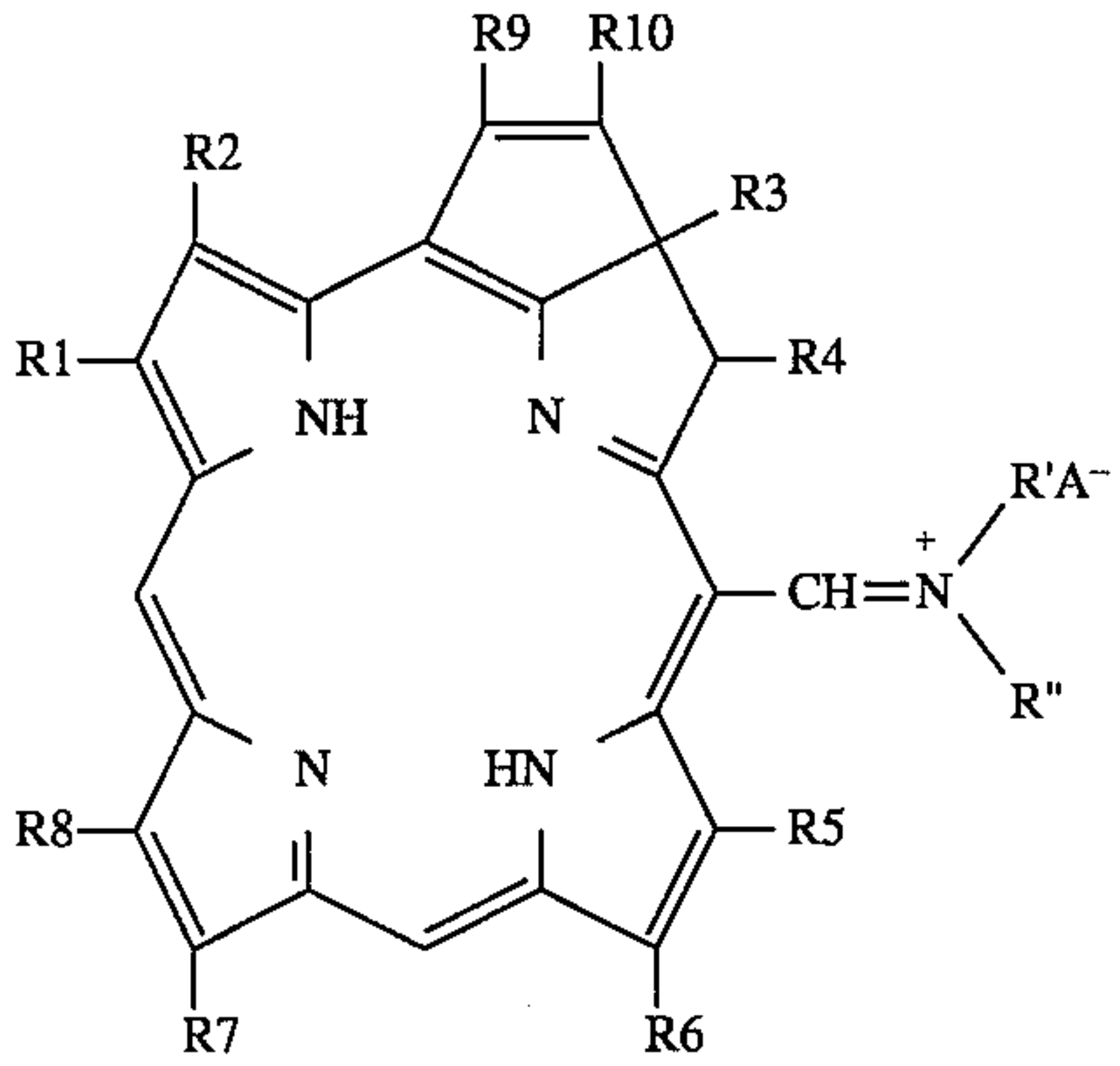
Bacteriochlorophyllimine III
