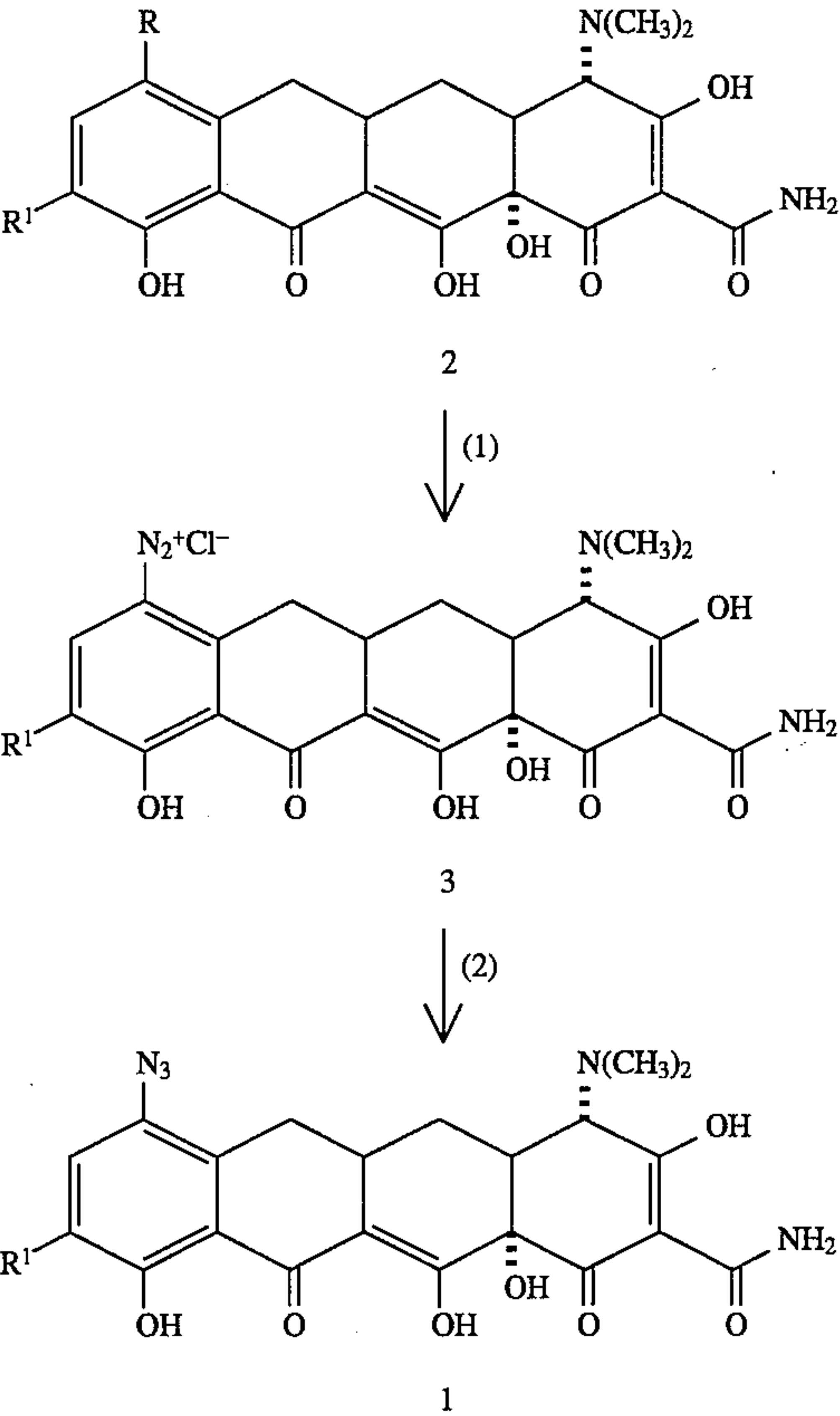
Scheme 1
