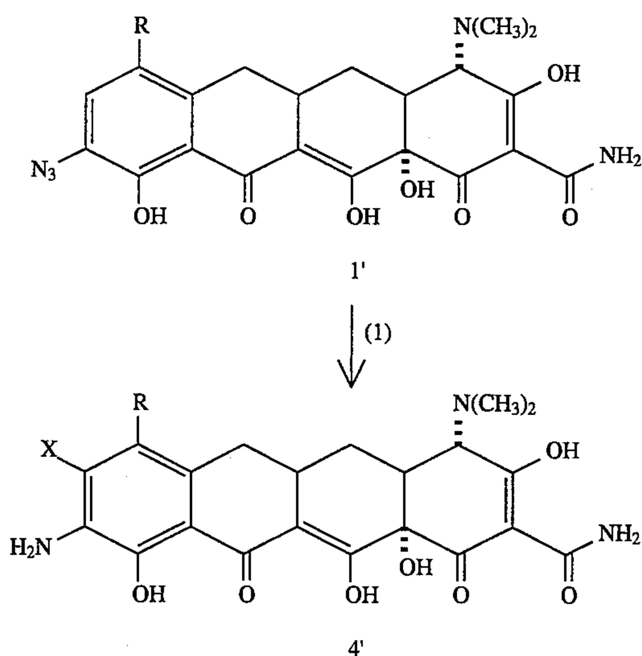
Scheme 4
