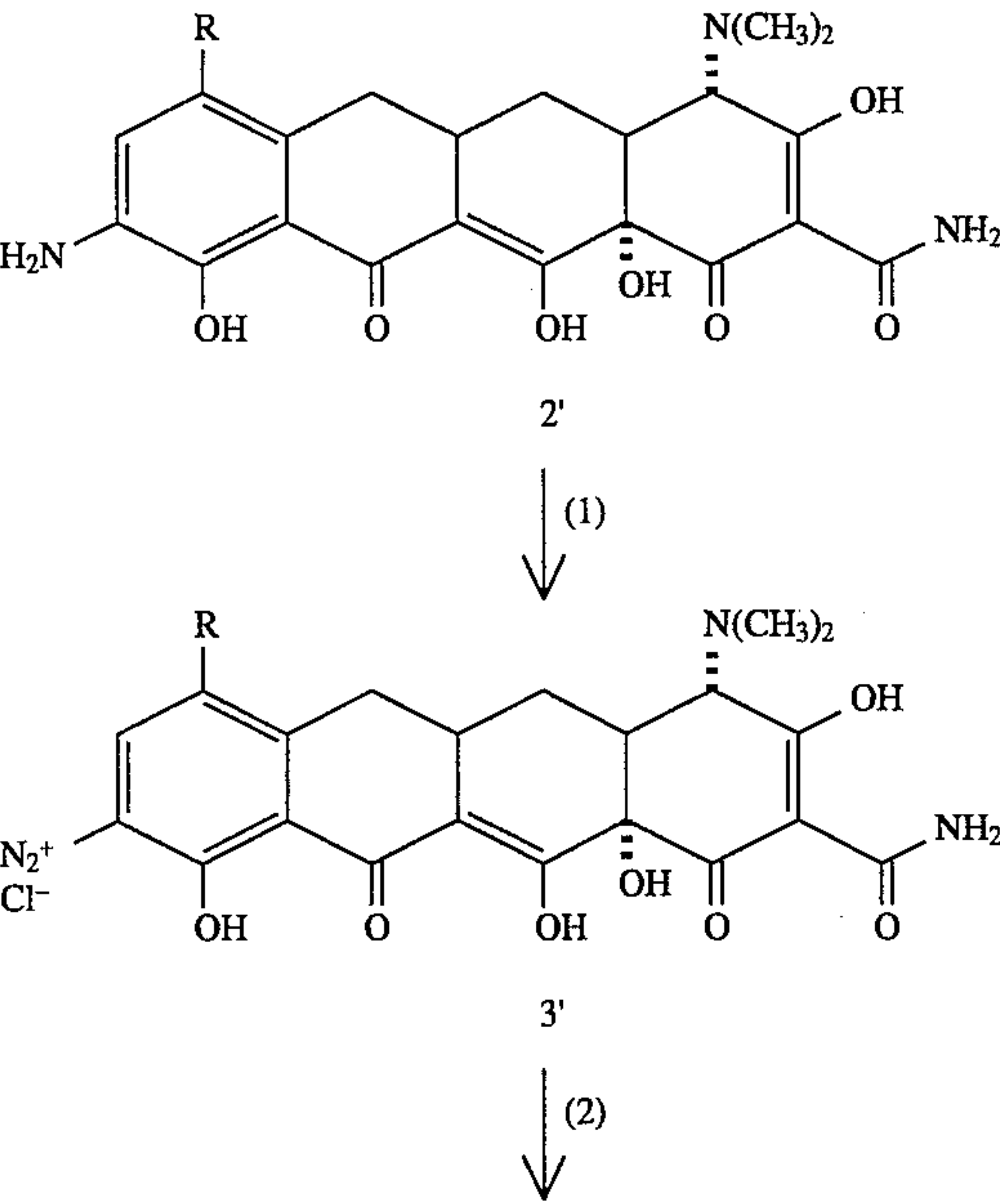
Scheme 2
