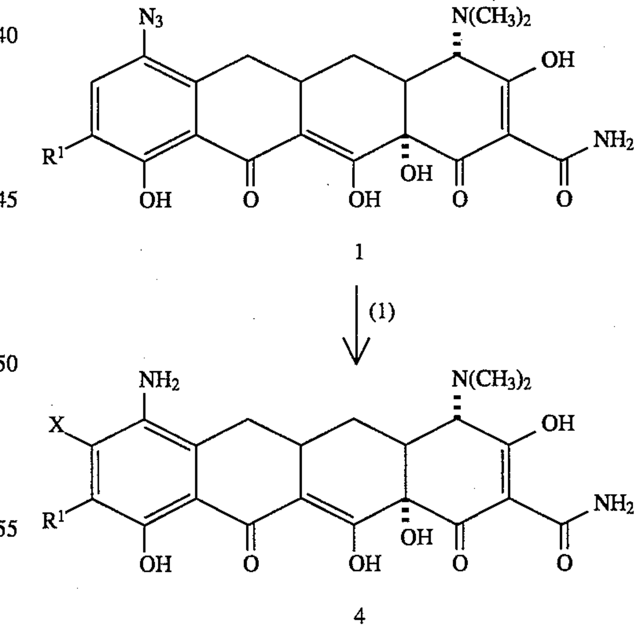
Scheme 3
