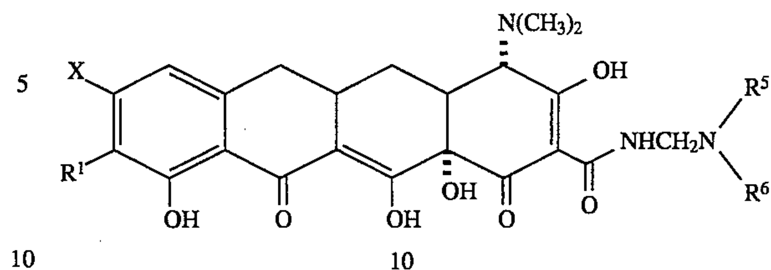
-continued Scheme 13
