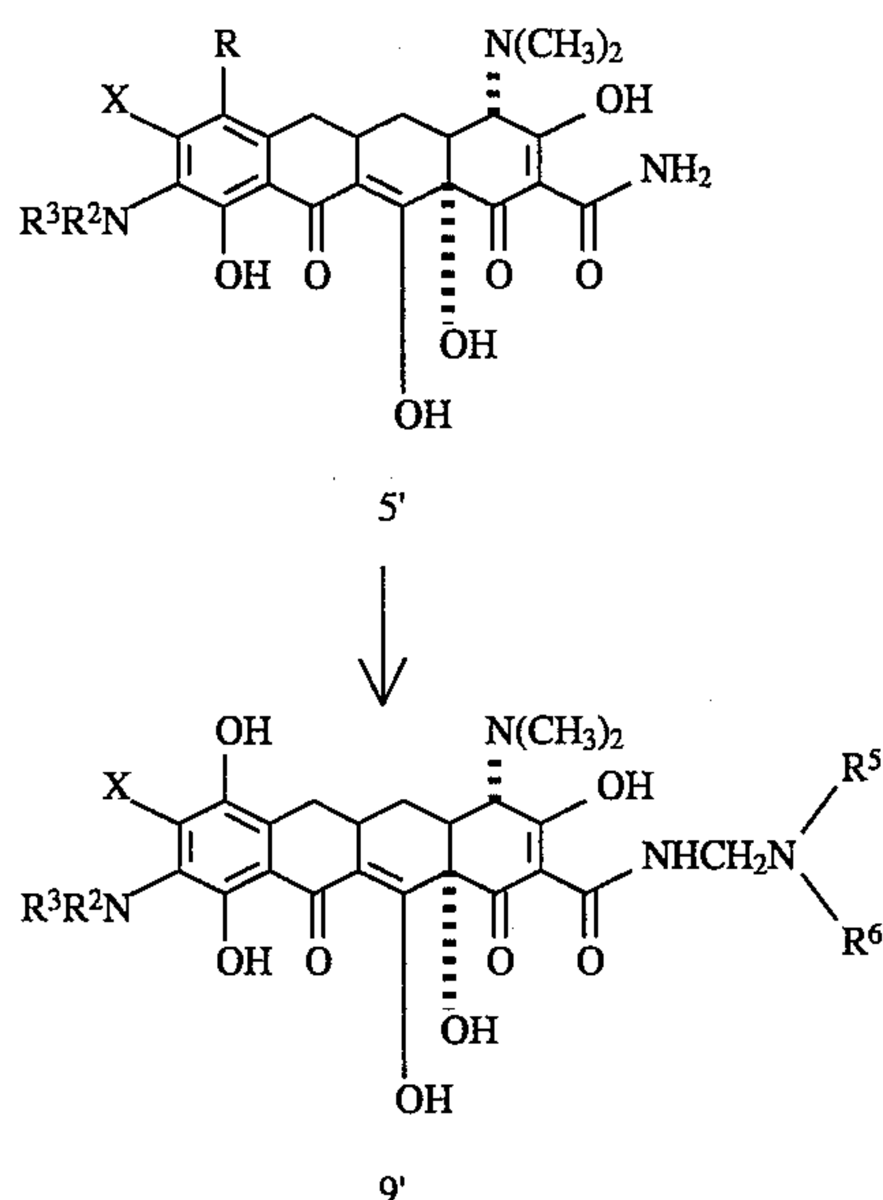
Scheme 12
