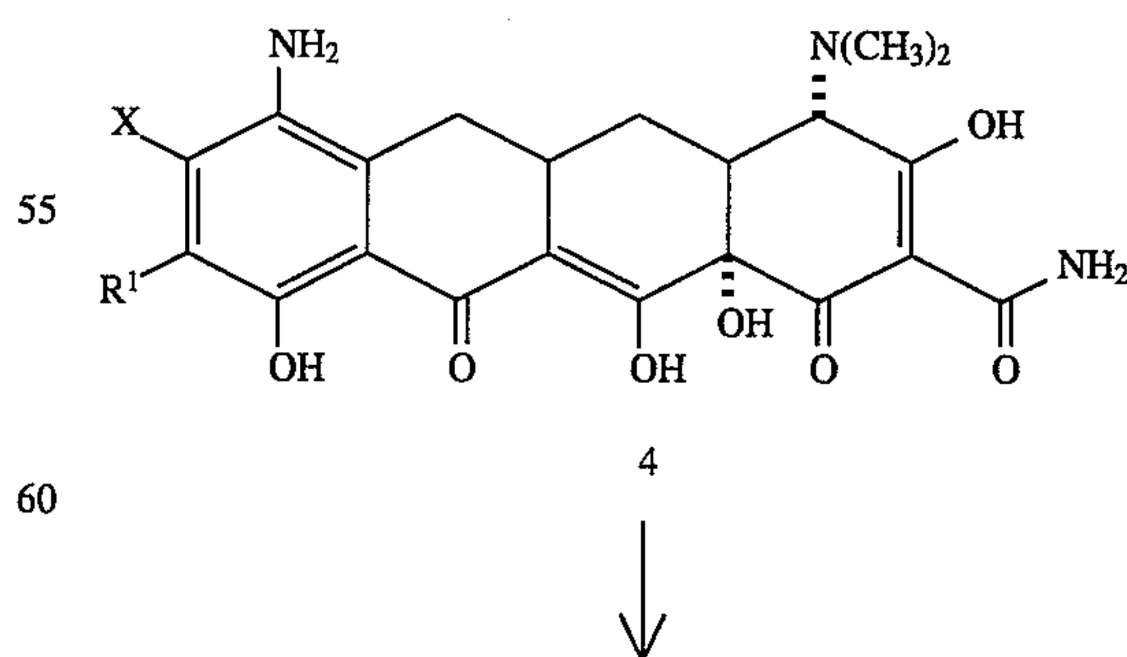
Scheme 7
