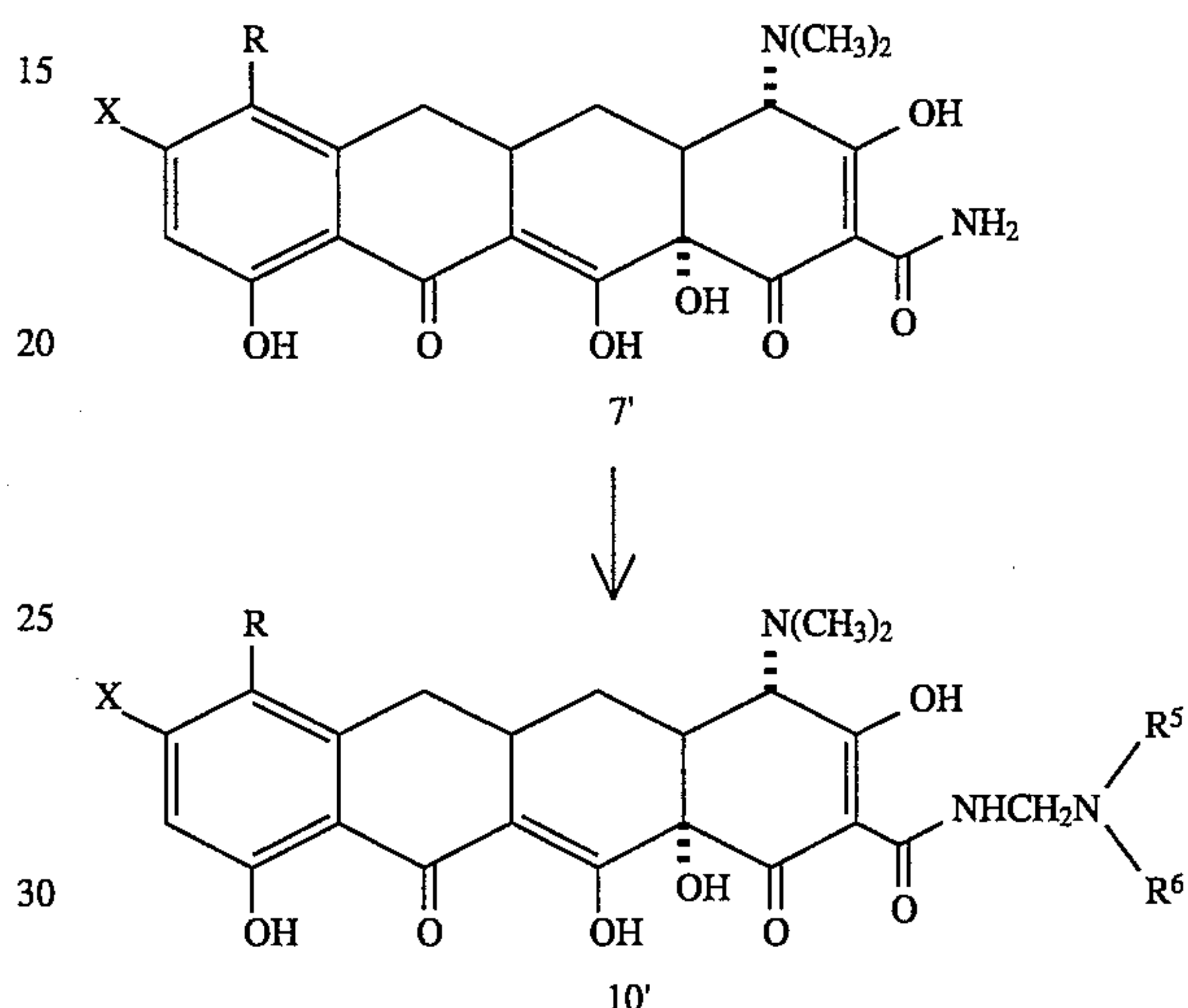
Scheme 14
