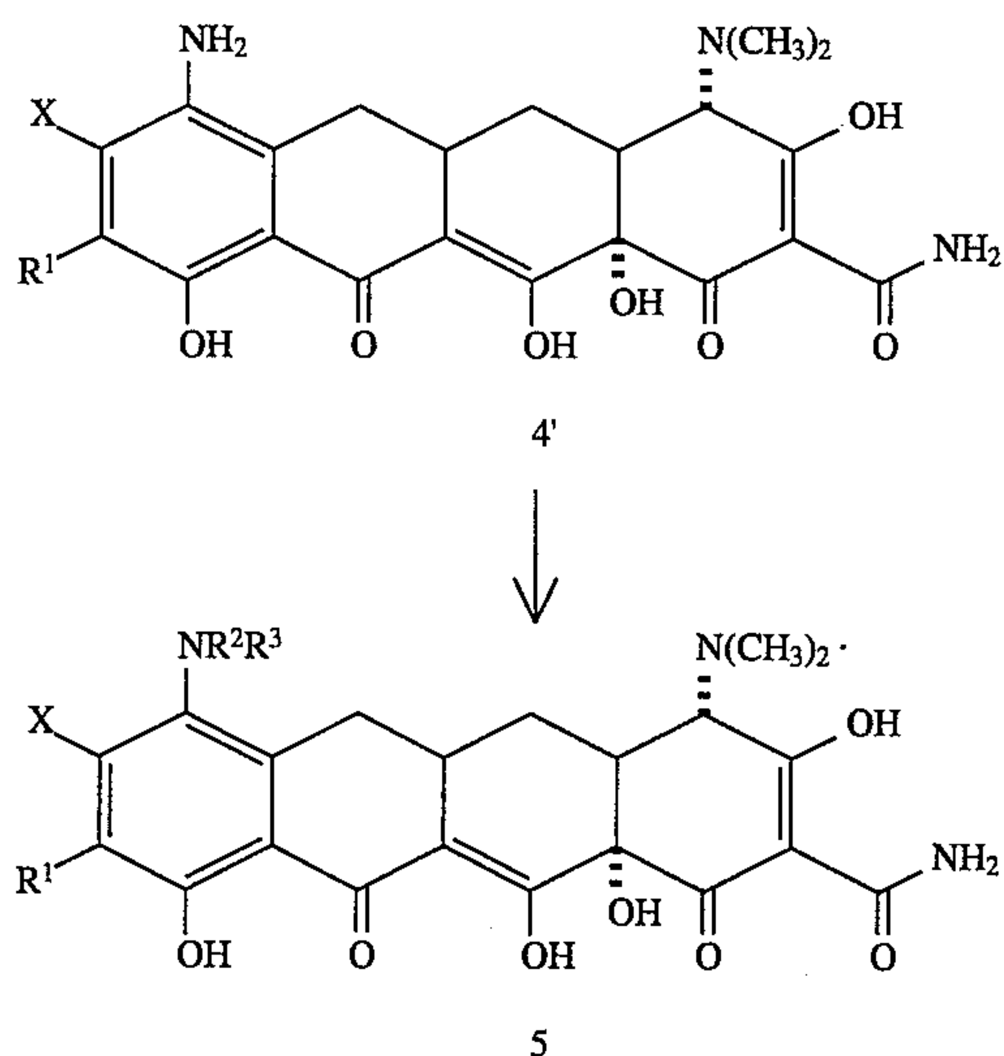
Scheme 5
