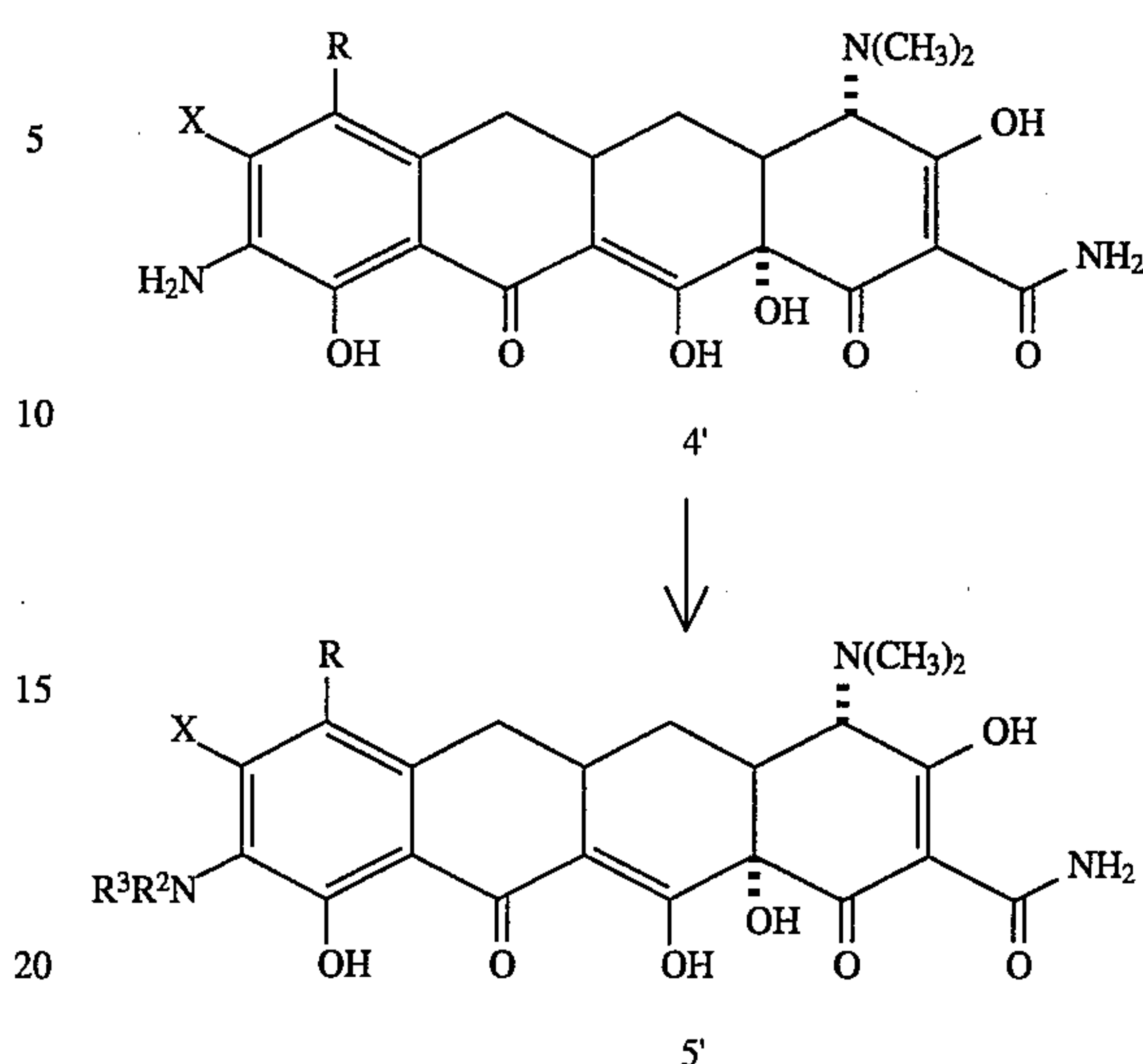
Scheme 6
