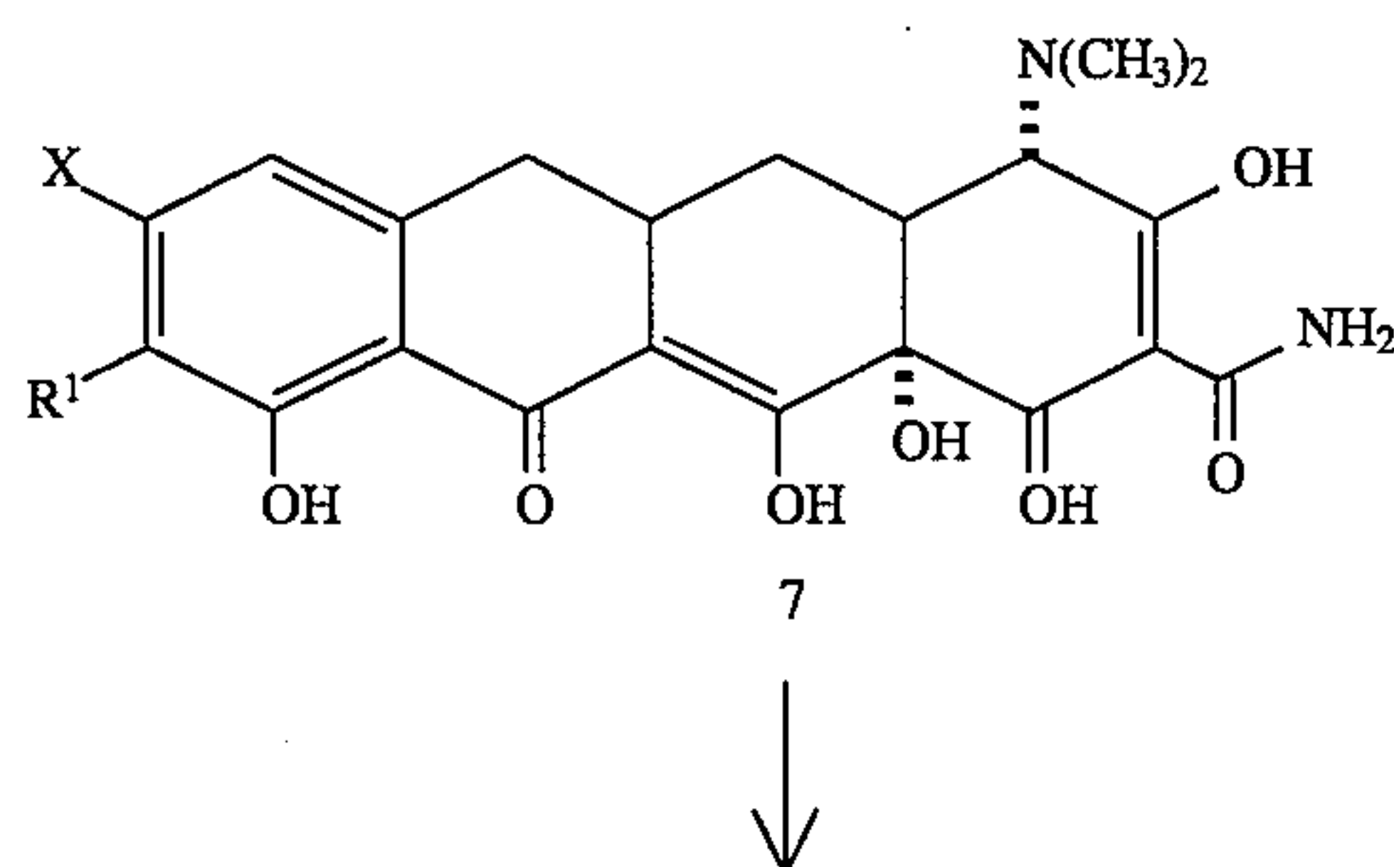
Scheme 13
