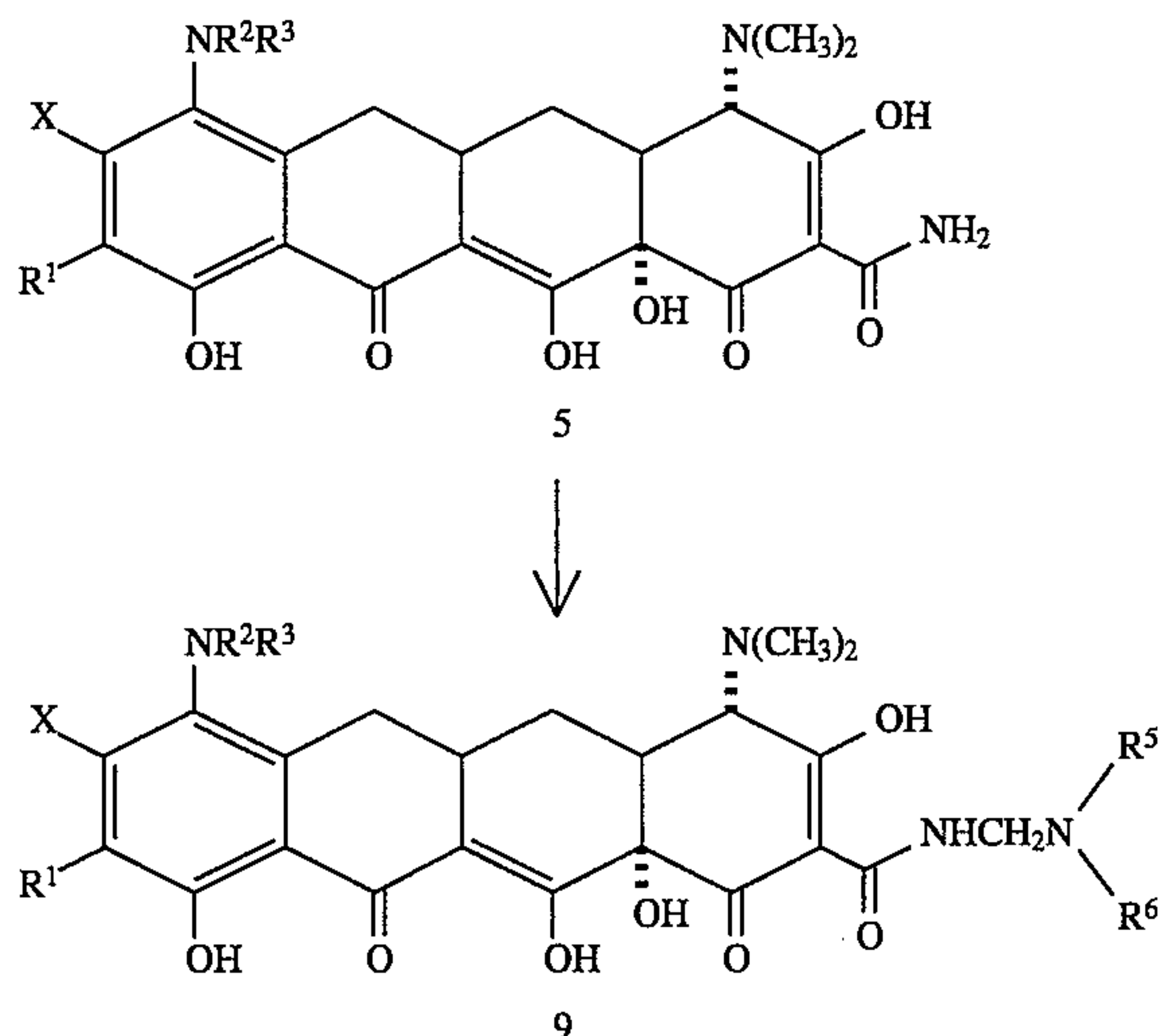
Scheme 11
