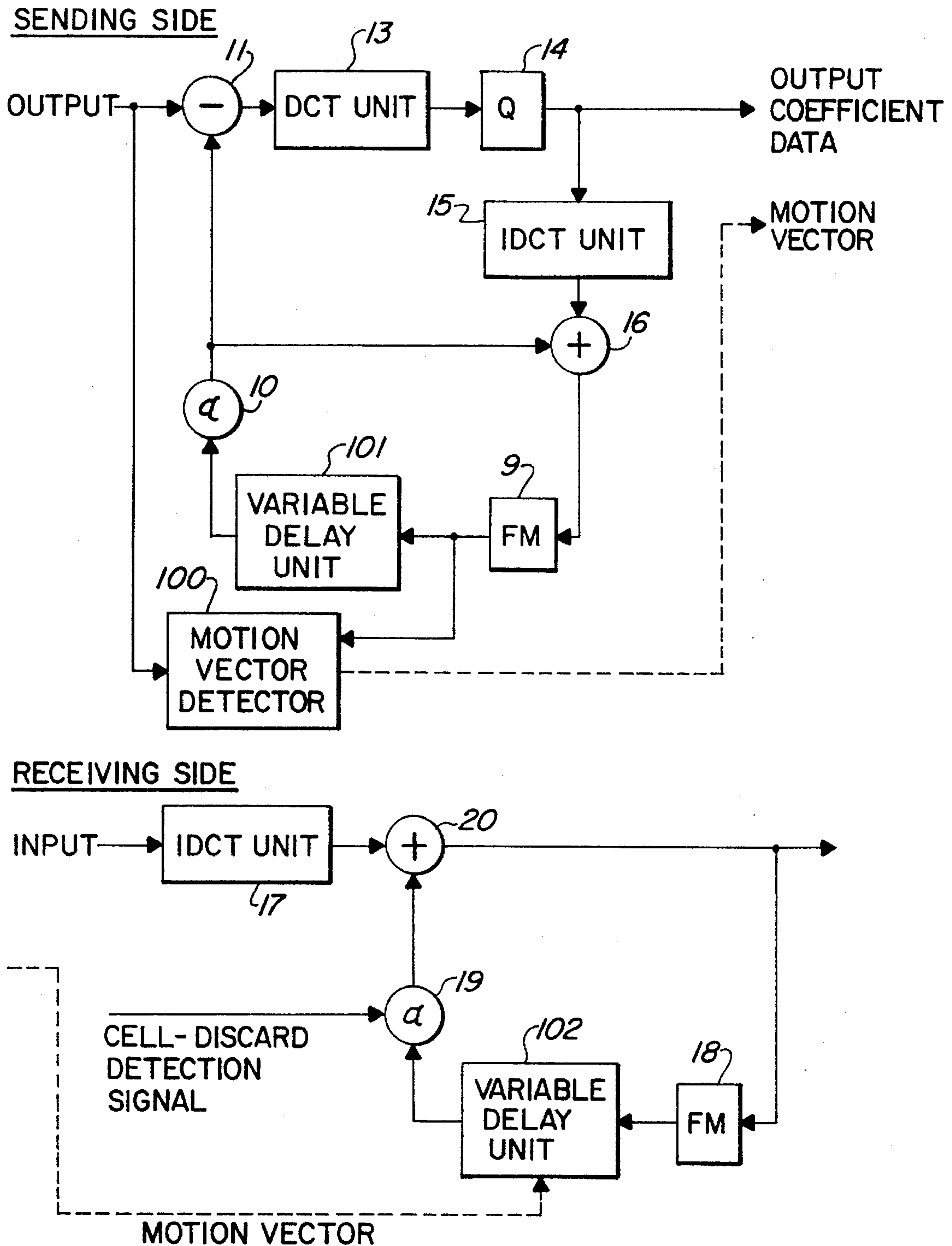
Fig. 4 (PRIOR ART)
