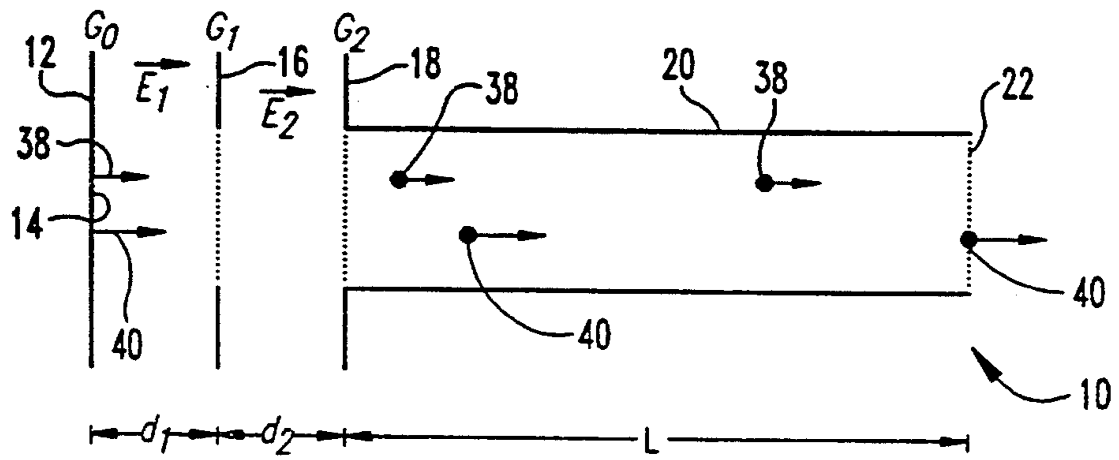
Fig. 4 (Prior Art)
