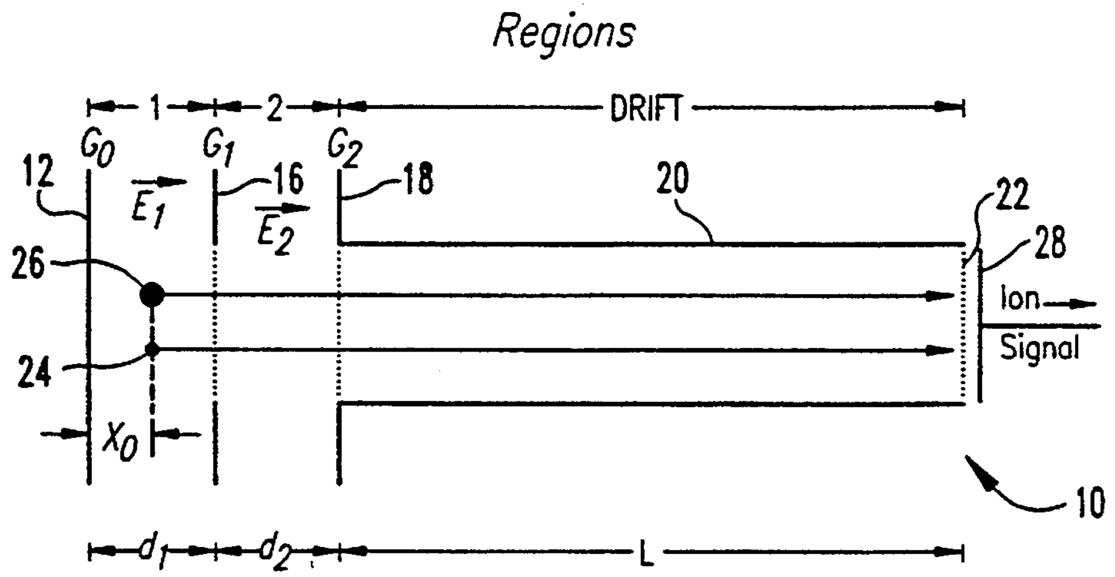
Fig. 1 (Prior Art)
