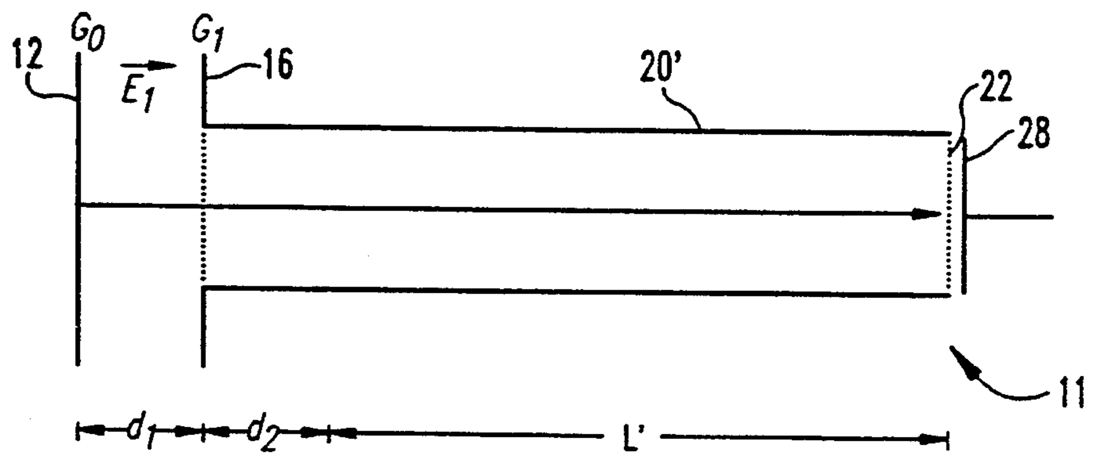
Fig. 5 (Prior Art)
