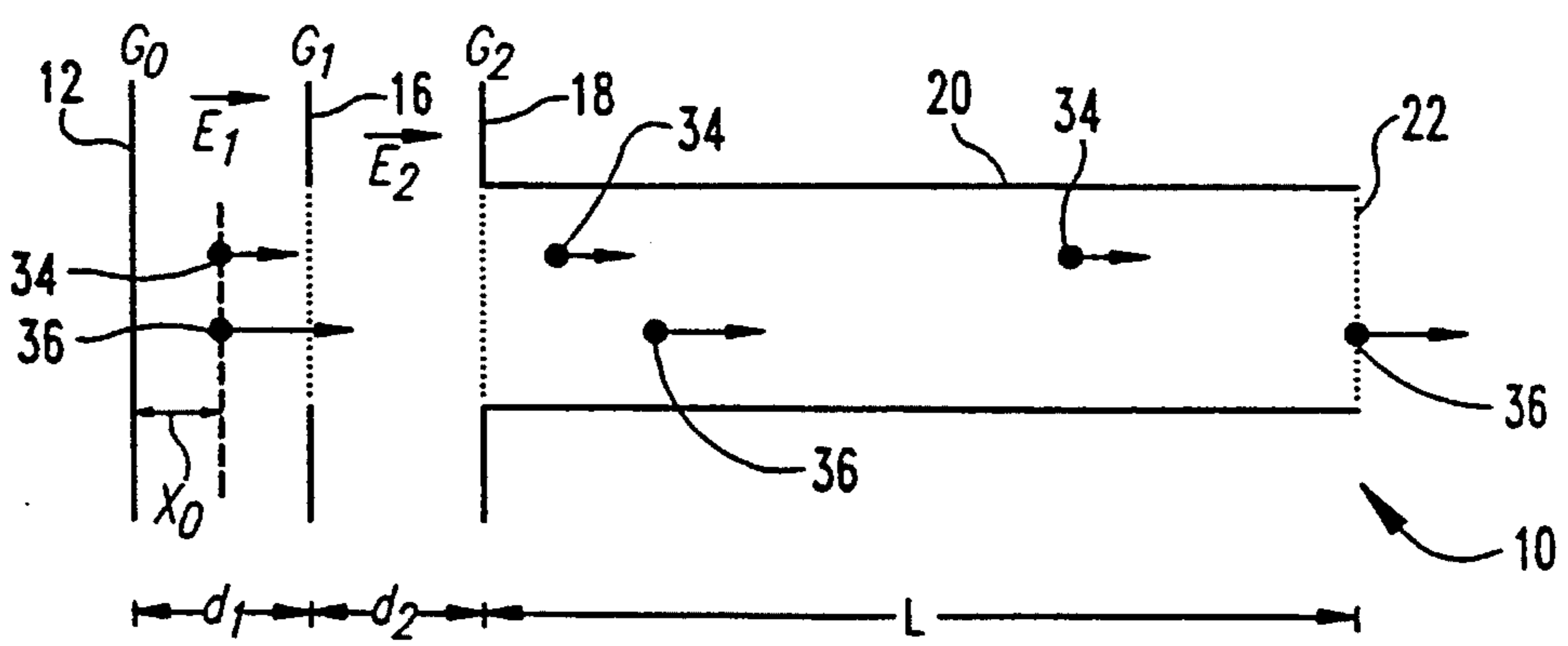
Fig. 3 (Prior Art)
