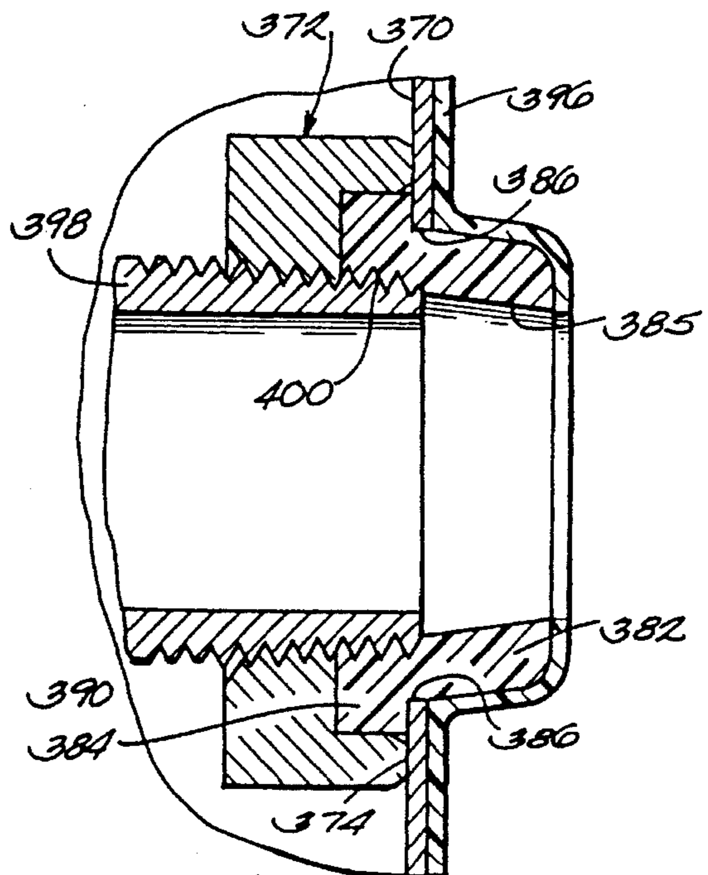
Fig. 8 PRIOR ART
