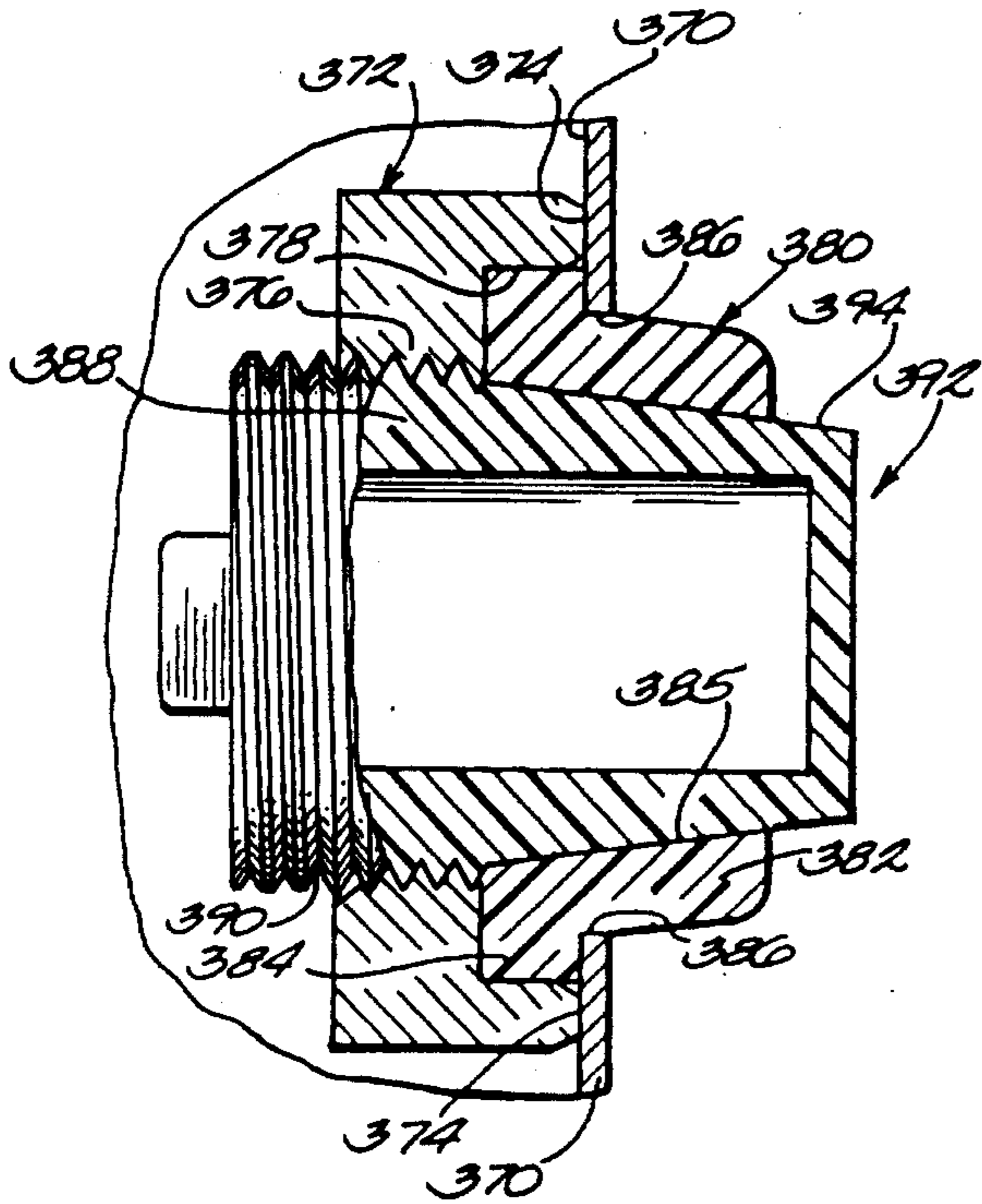
Fig. 5 PRIOR ART
