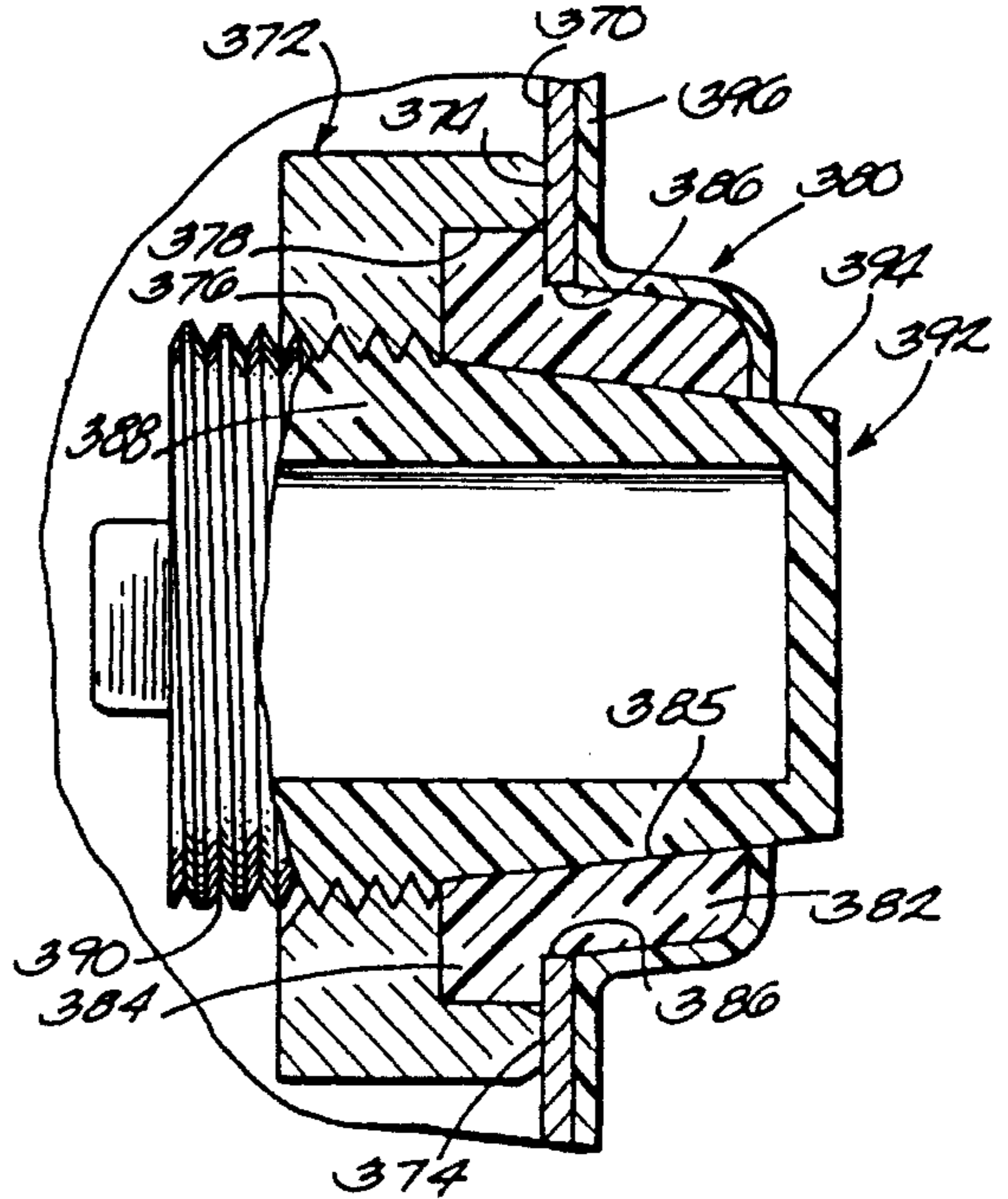
Fig. 6 PRIOR ART
