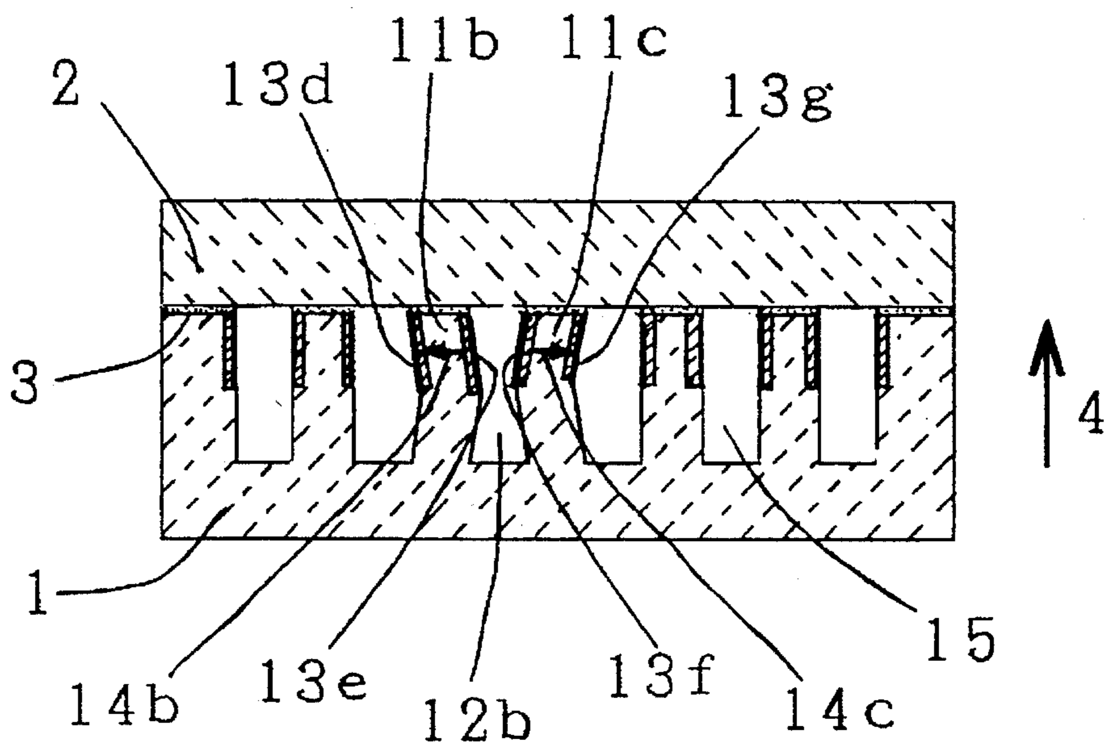
Fig.16 PRIOR ART
