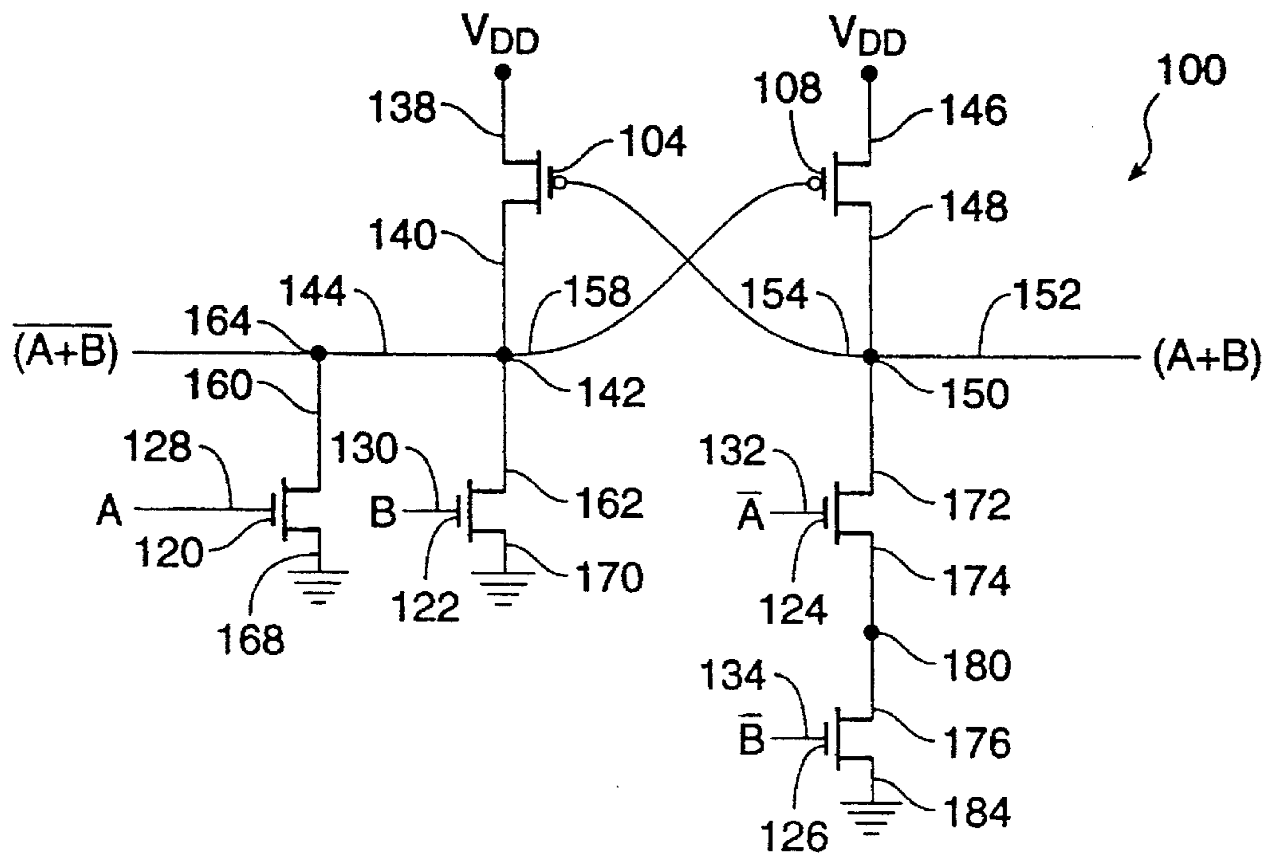
FIG. 2 (PRIOR ART)
