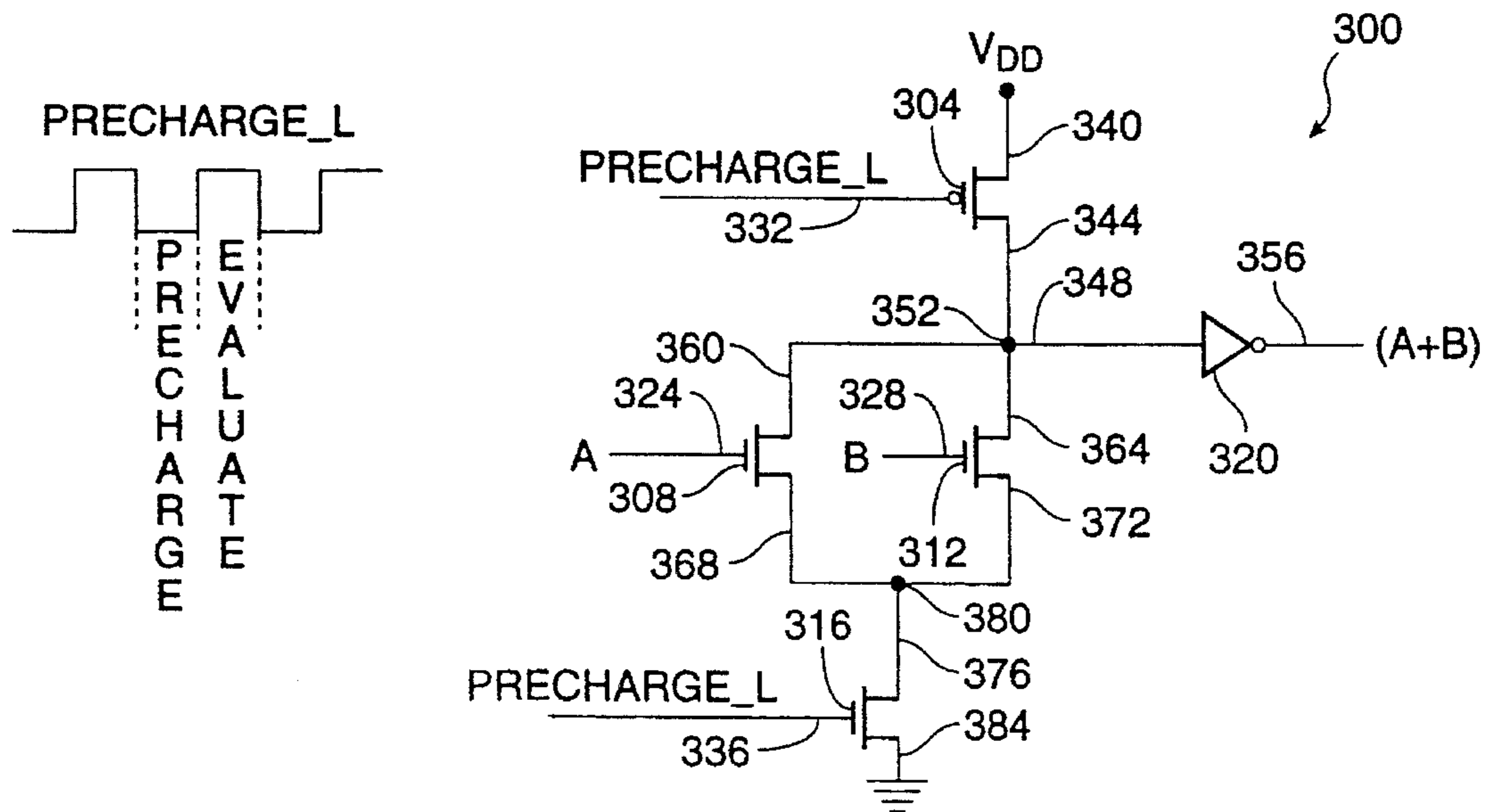
FIG. 4 (PRIOR ART)
