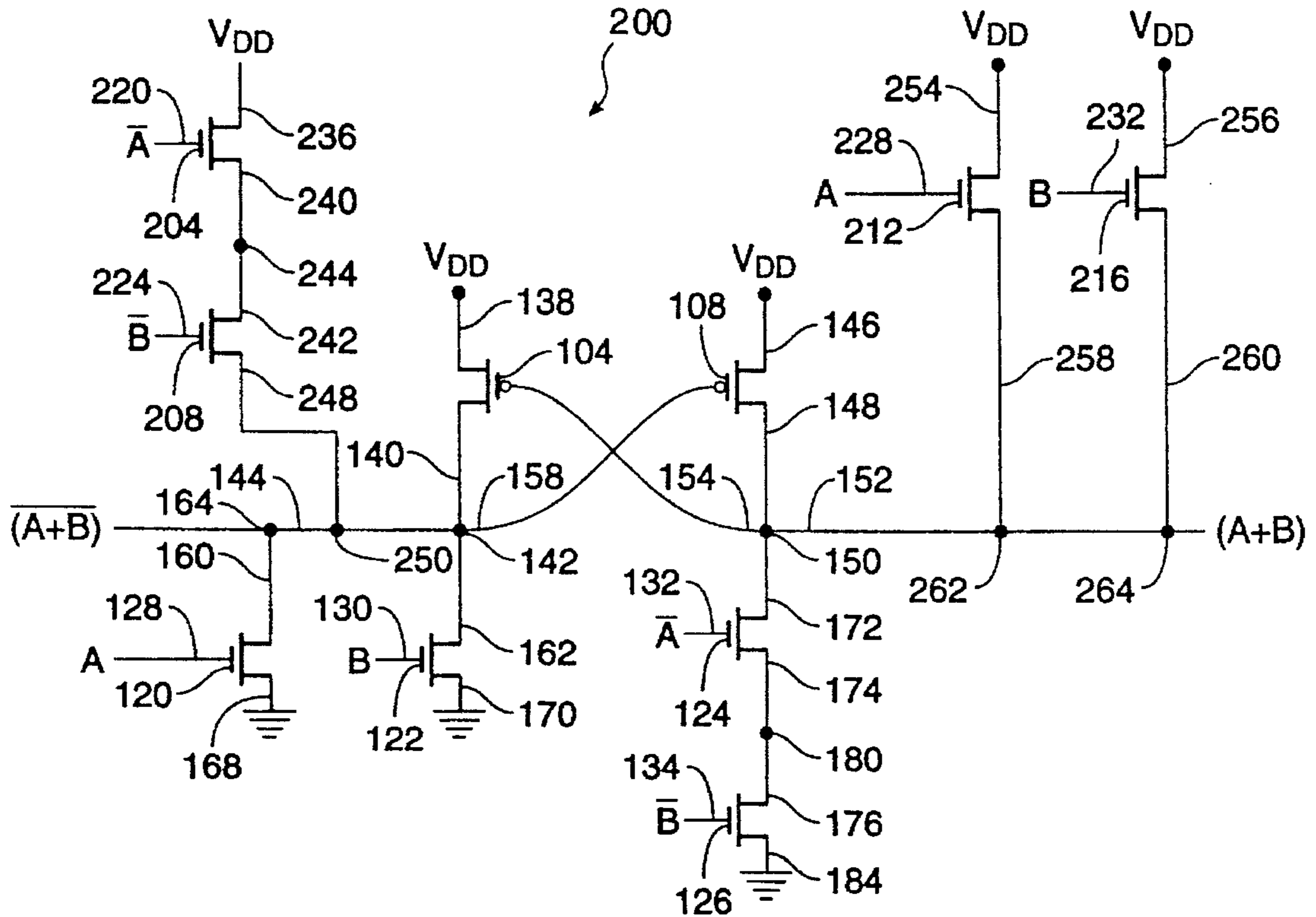
FIG. 3 (PRIOR ART)
