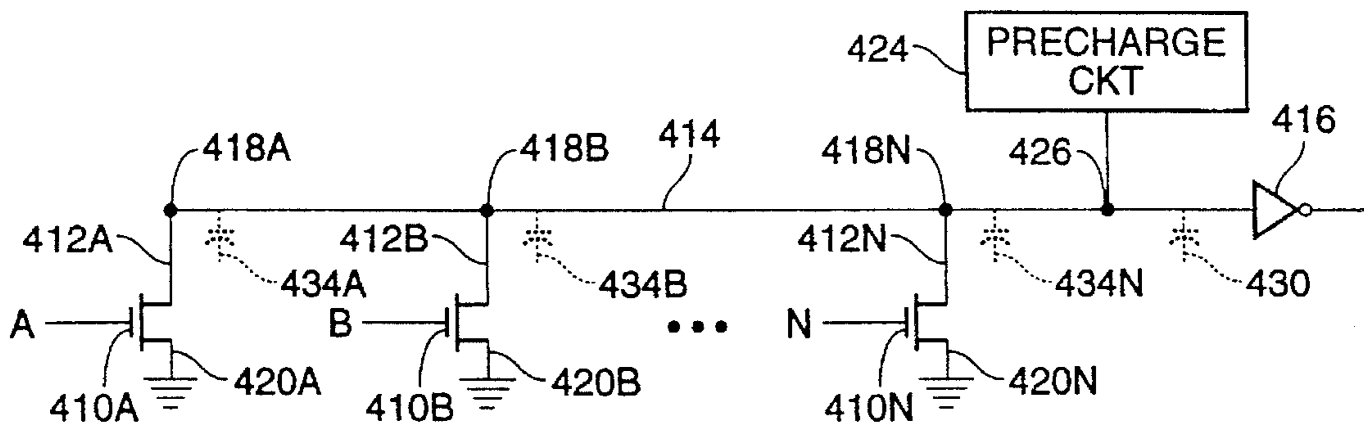
FIG. 5 (PRIOR ART)
