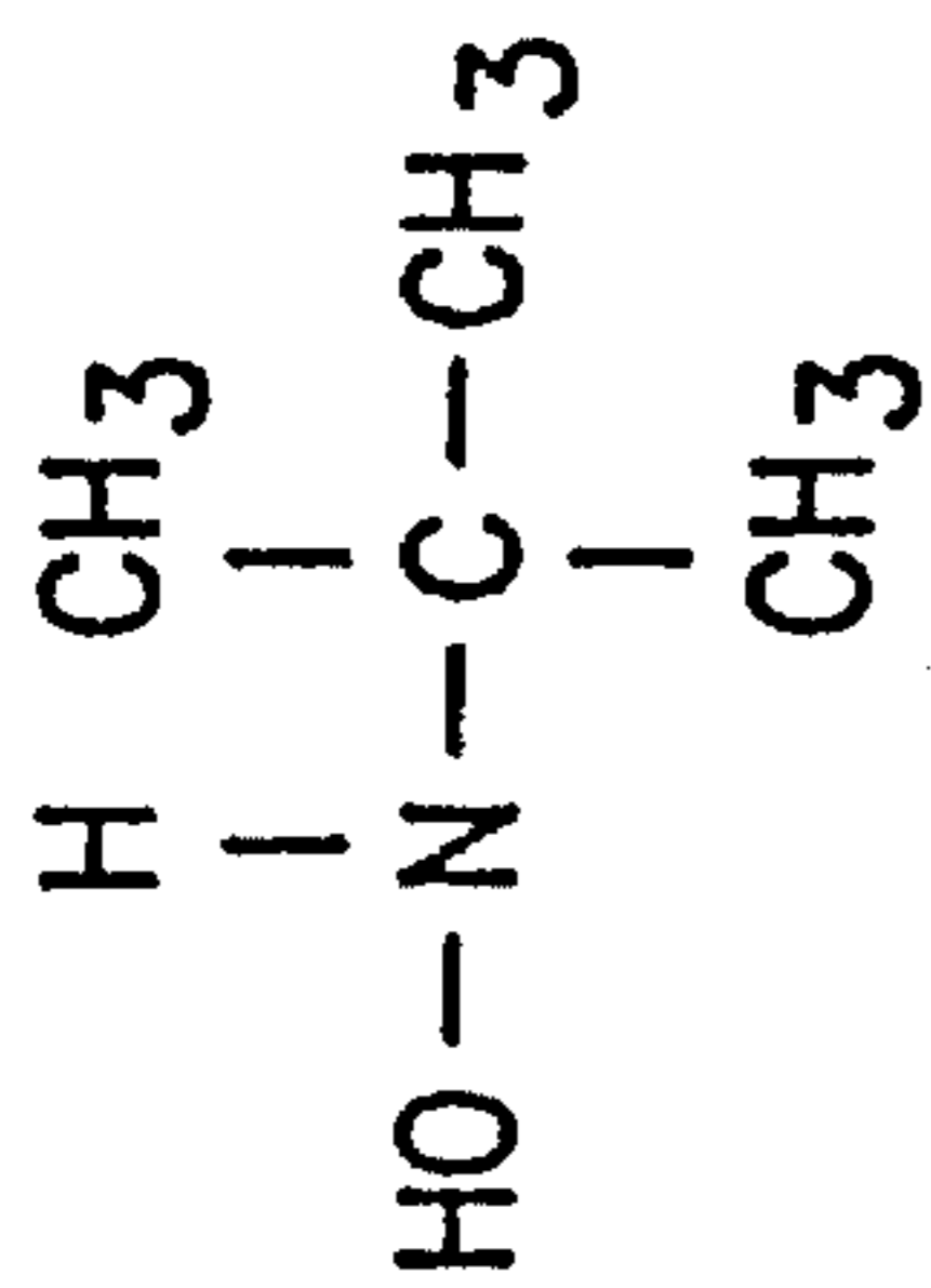
t -Butylhydroxylamine
