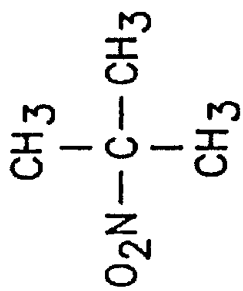
2-Methyl-2-nitropropane
