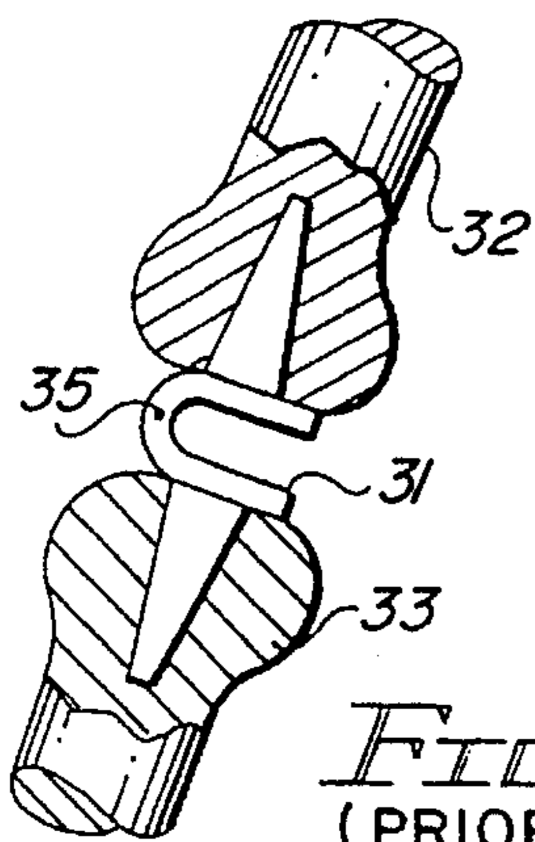
FIG. 1 (PRIOR ART)
