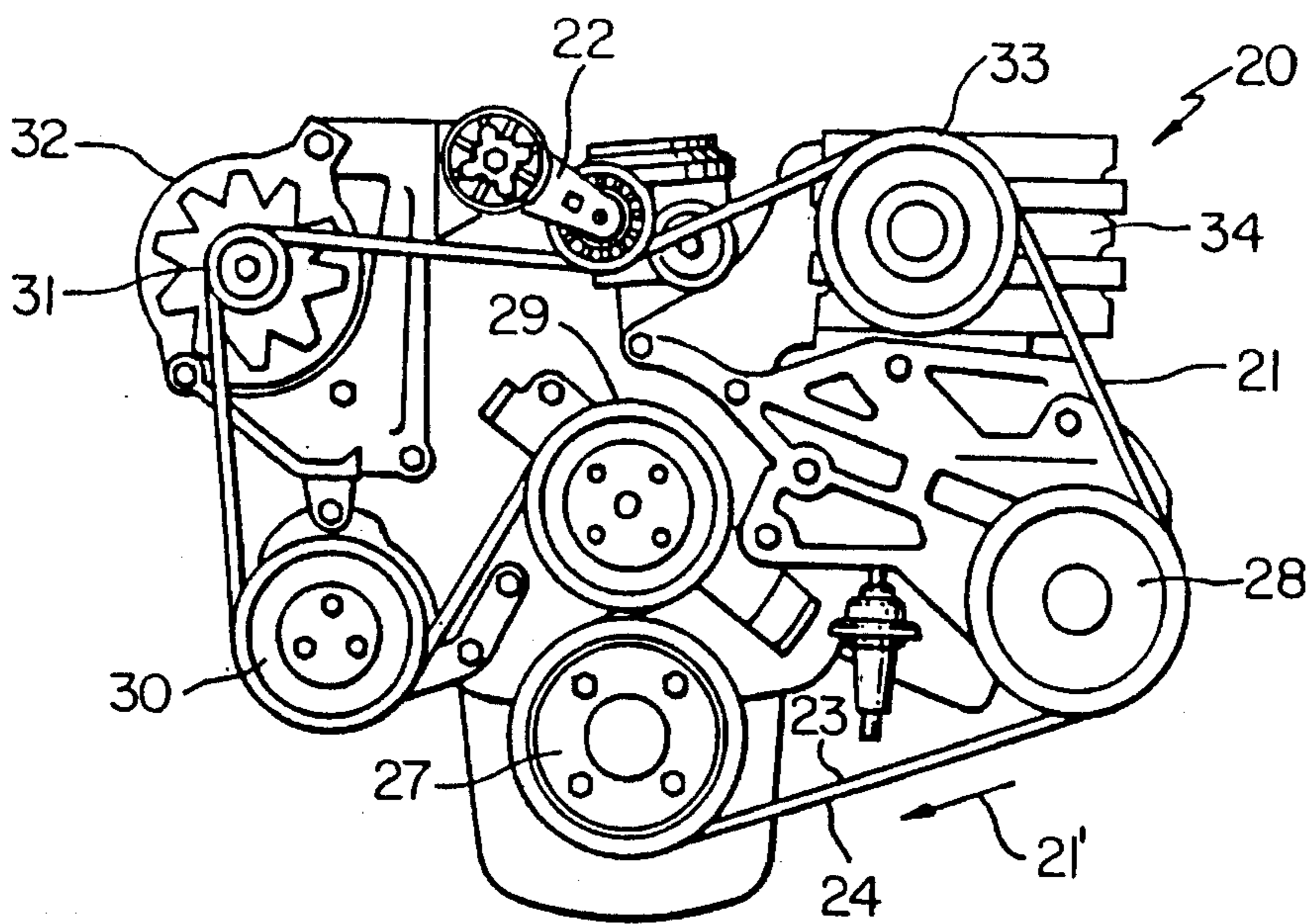
FIG. 2 PRIOR ART
