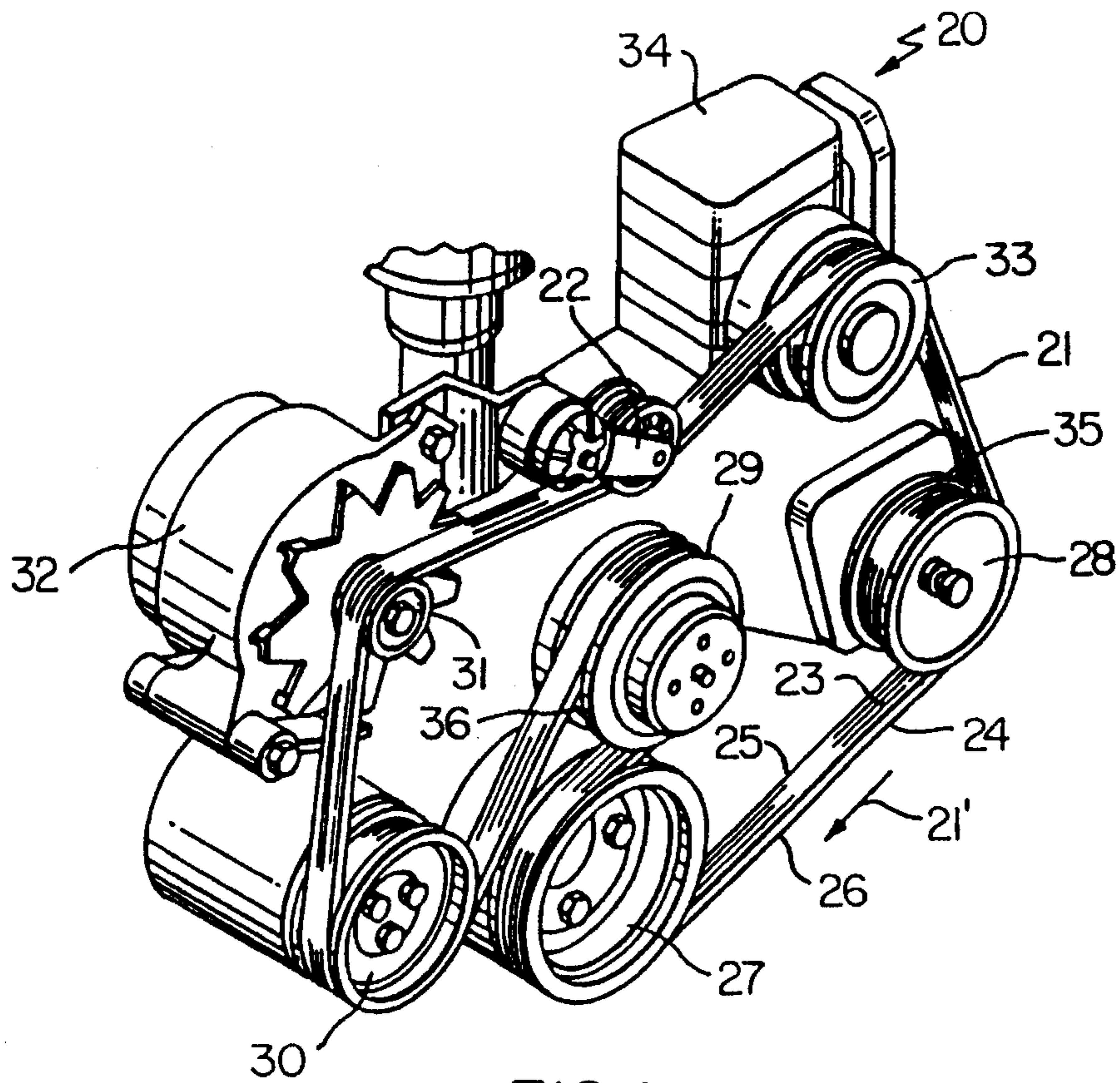
FIG. 1 PRIOR ART
