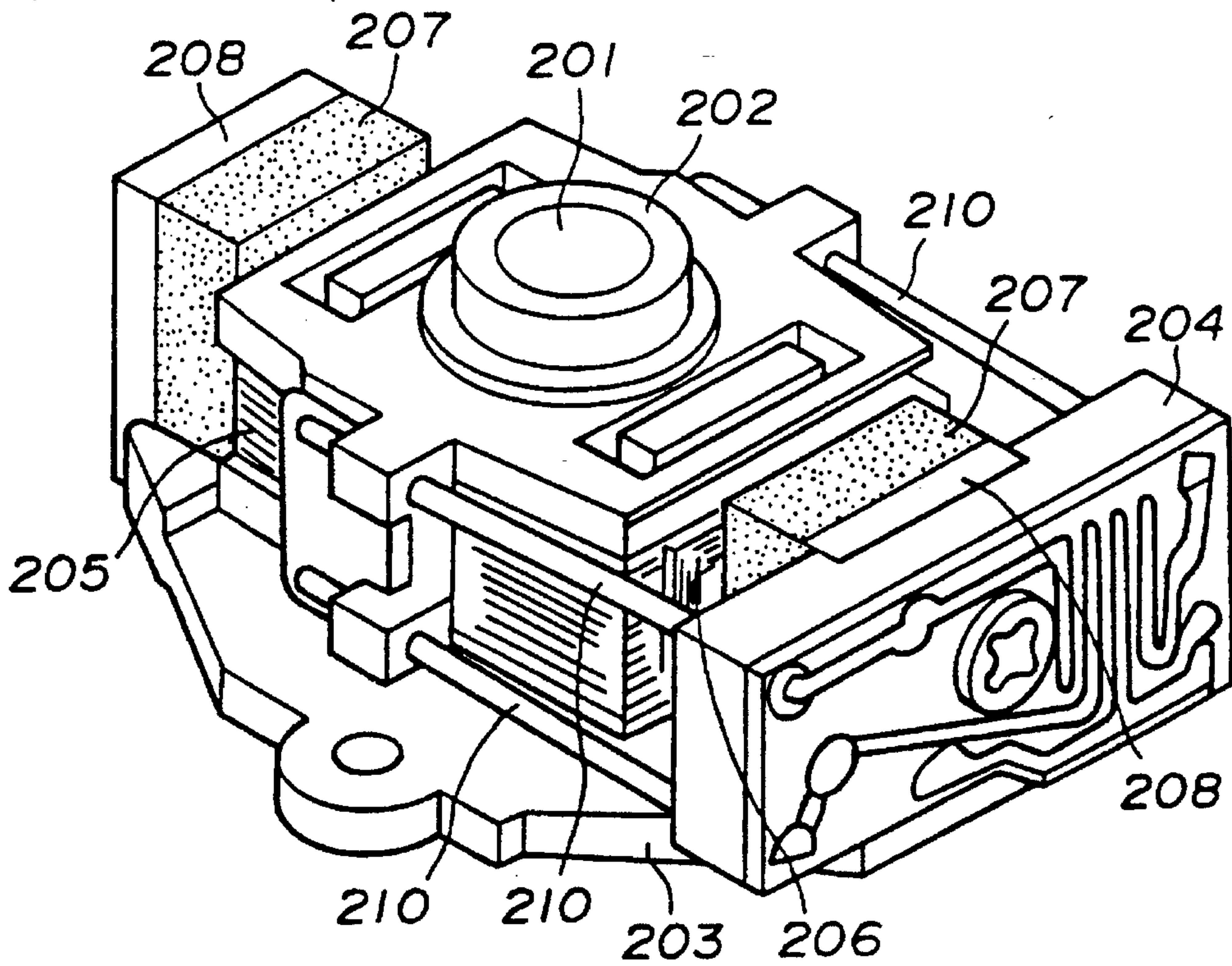
FIG. 2 (PRIOR ART)
