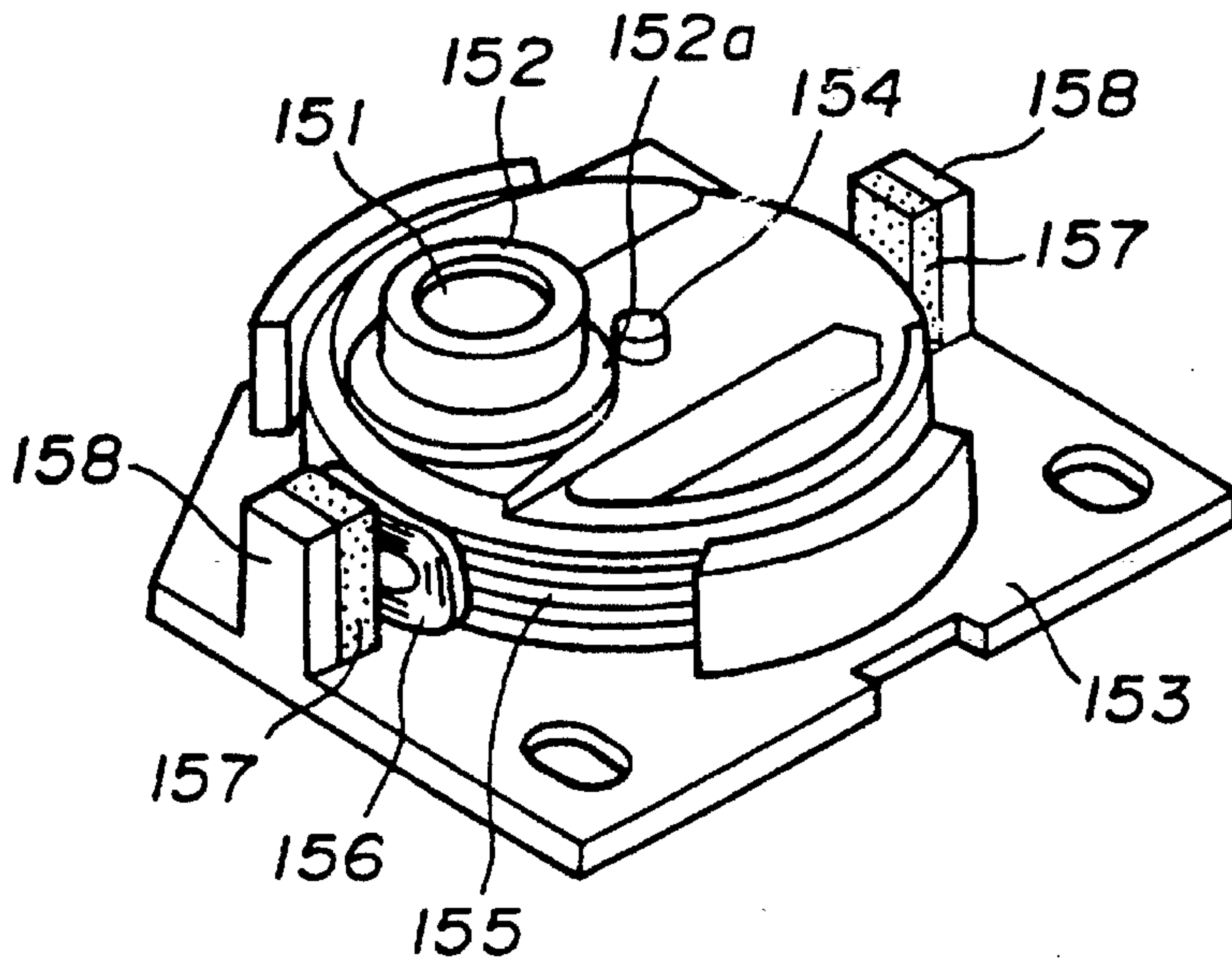
FIG. 1 (PRIOR ART)
