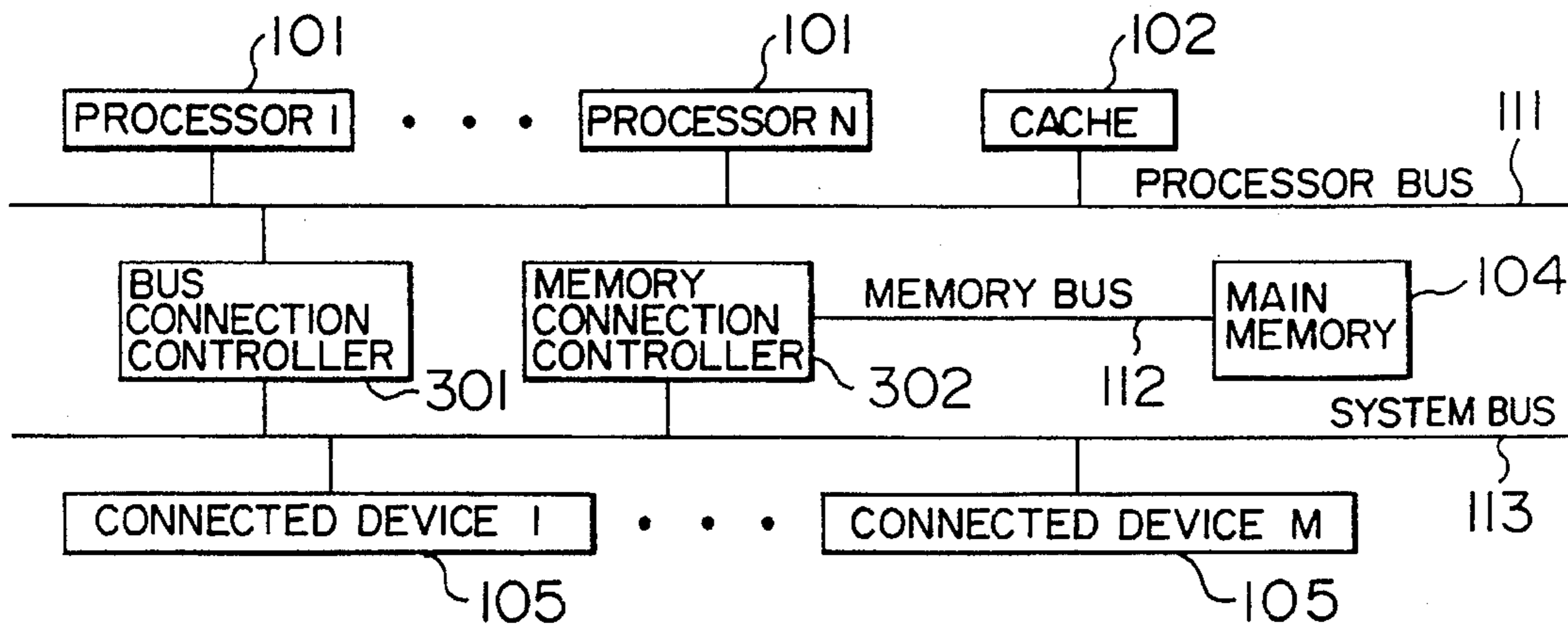
FIG. 3 PRIOR ART
