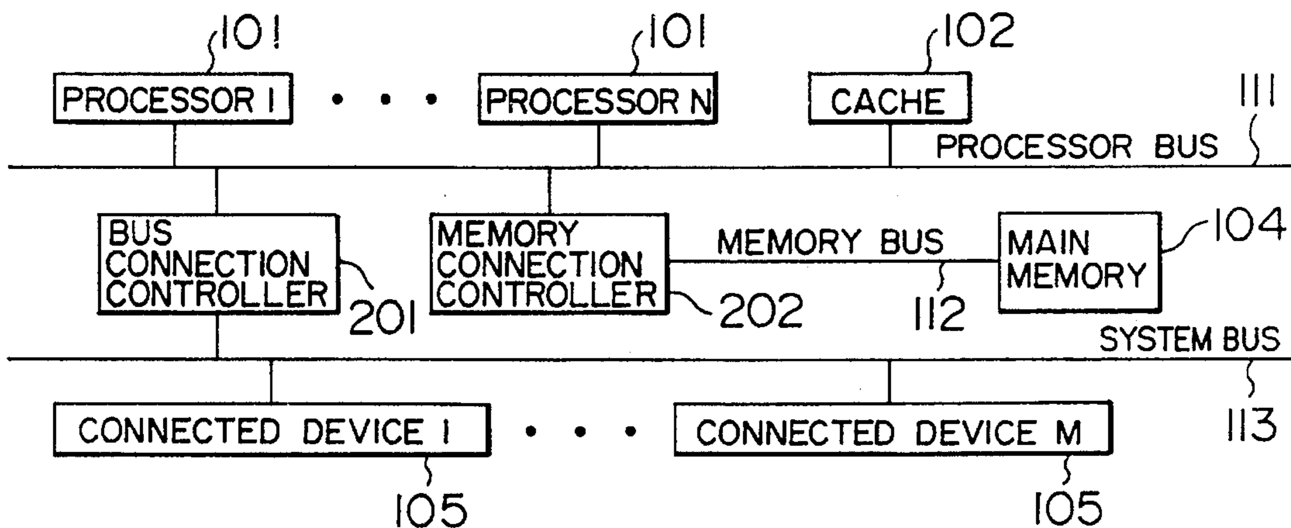
FIG. 3 PRIOR ART
