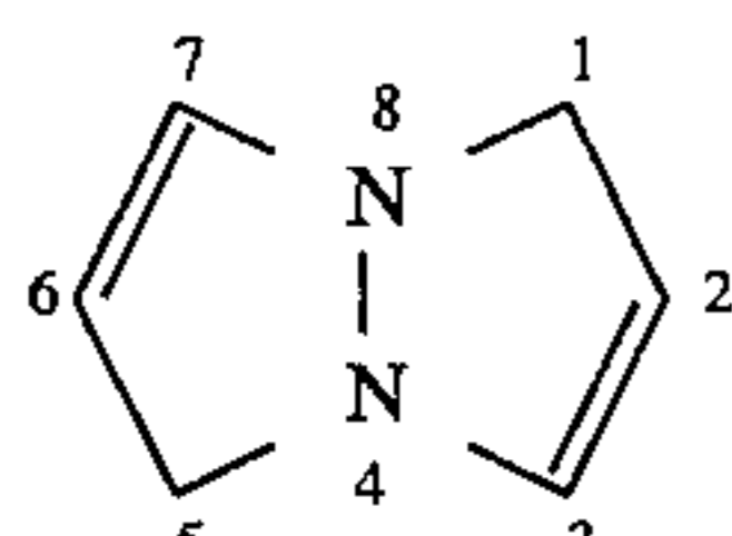
1H,5H-pyrazolo[1,2-a]pyrazole.
