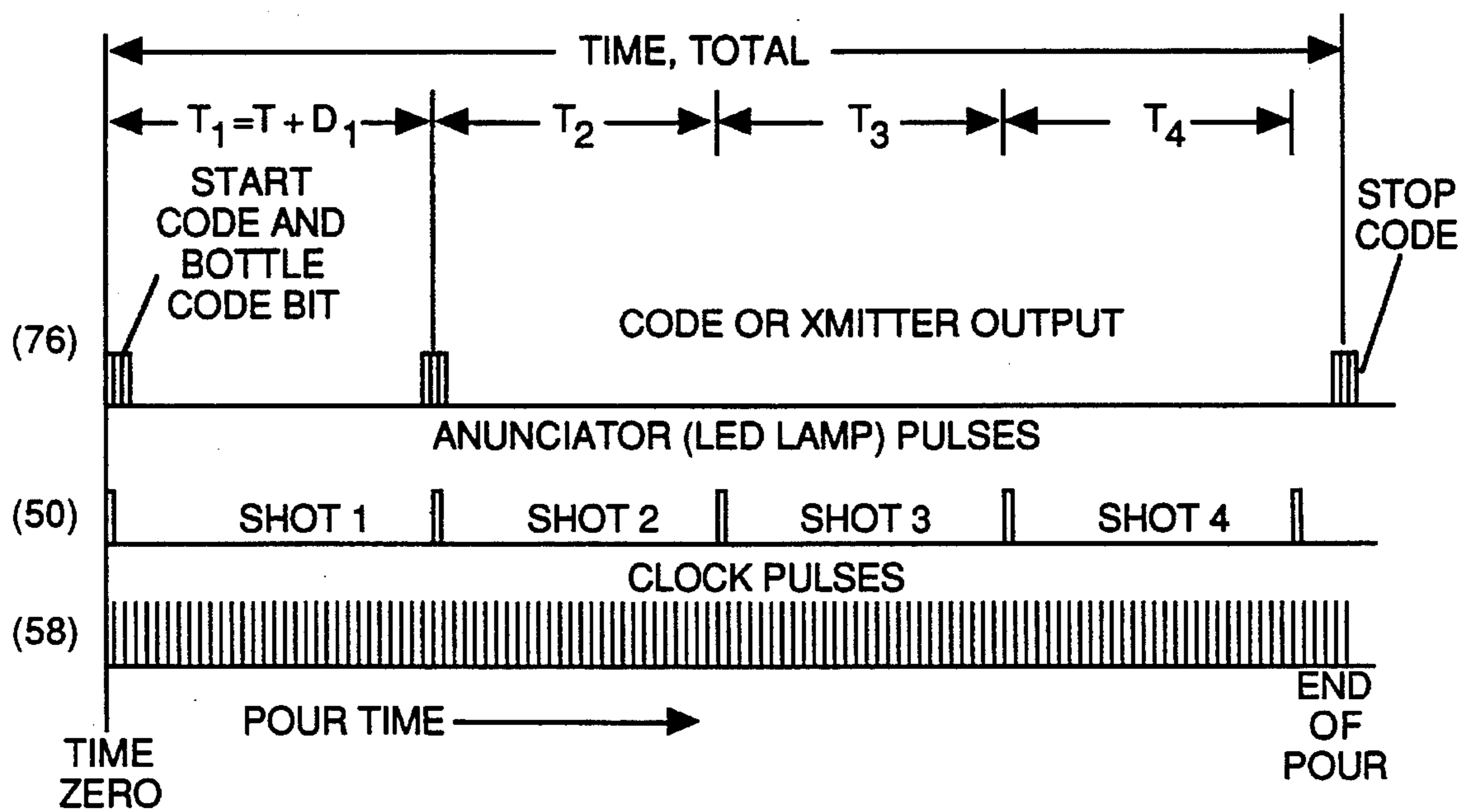
TIMING CYCLE FOR "SHOT" TIMER-CODER-XMITTER
