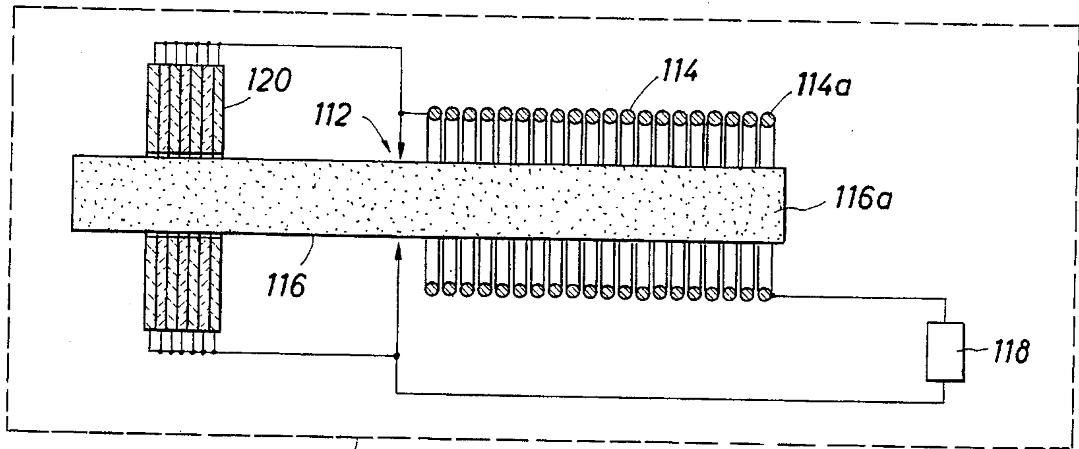
FIG. 22 (PRIOR ART)
