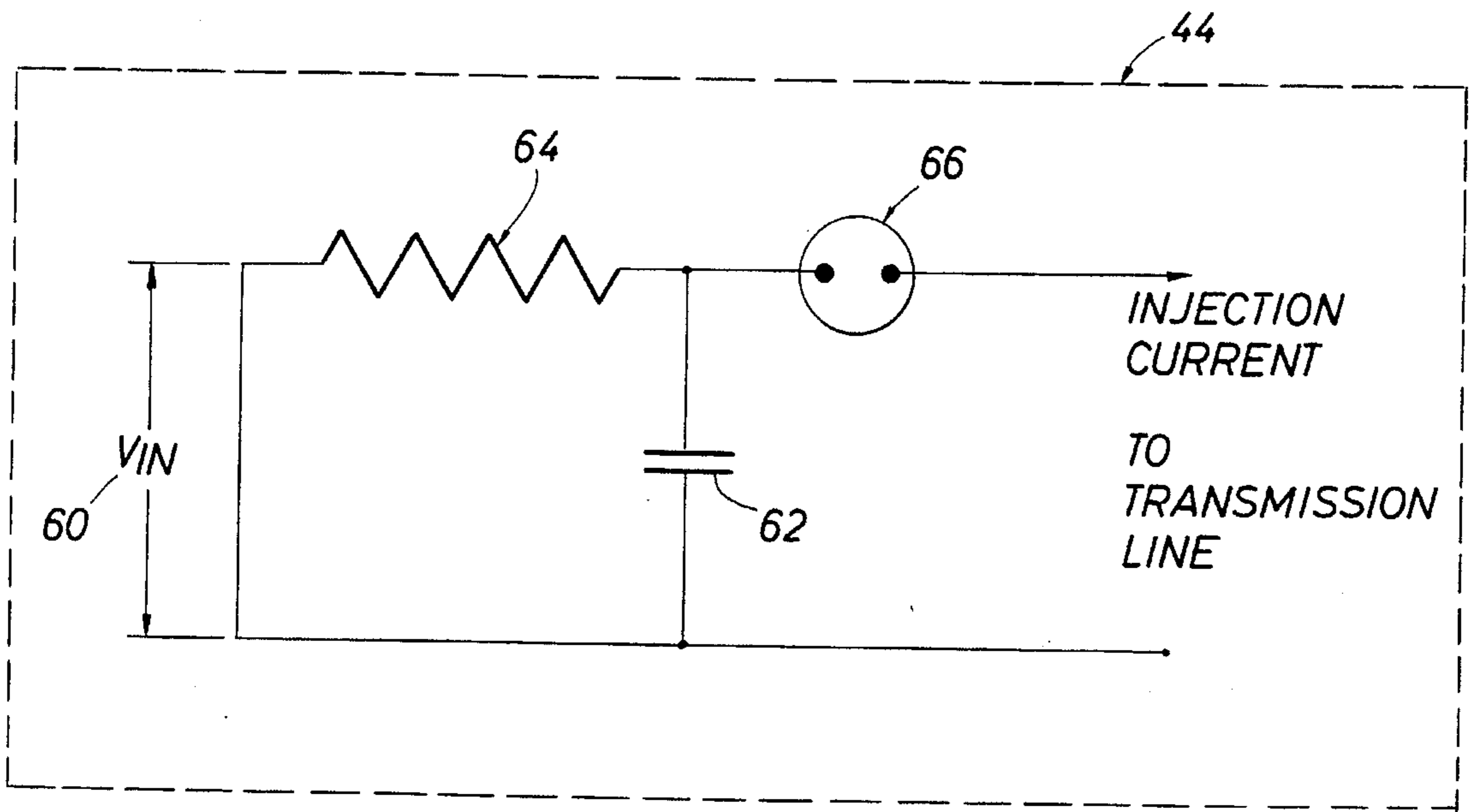
FIG.18 (PRIOR ART)
