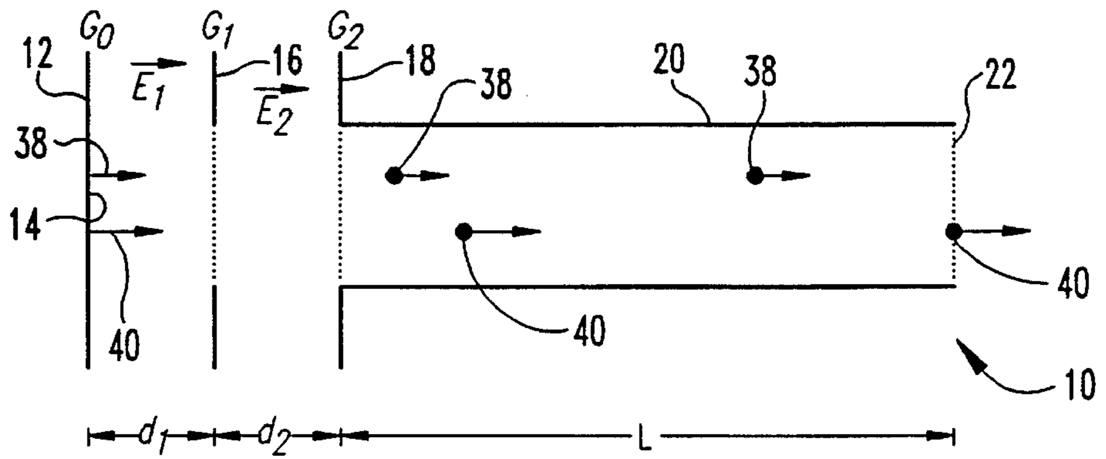
Fig. 4 (Prior Art)
