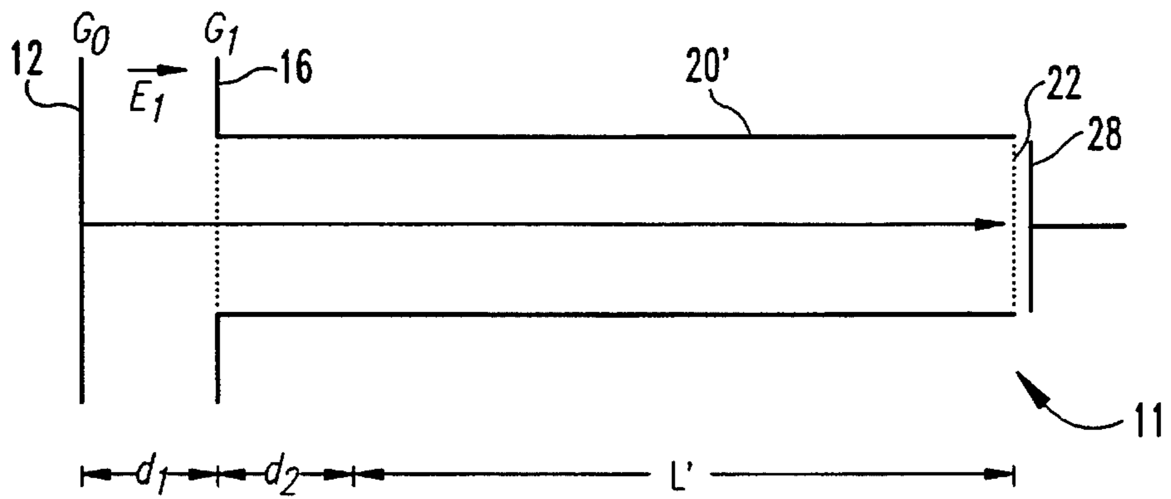
Fig. 5 (Prior Art)
