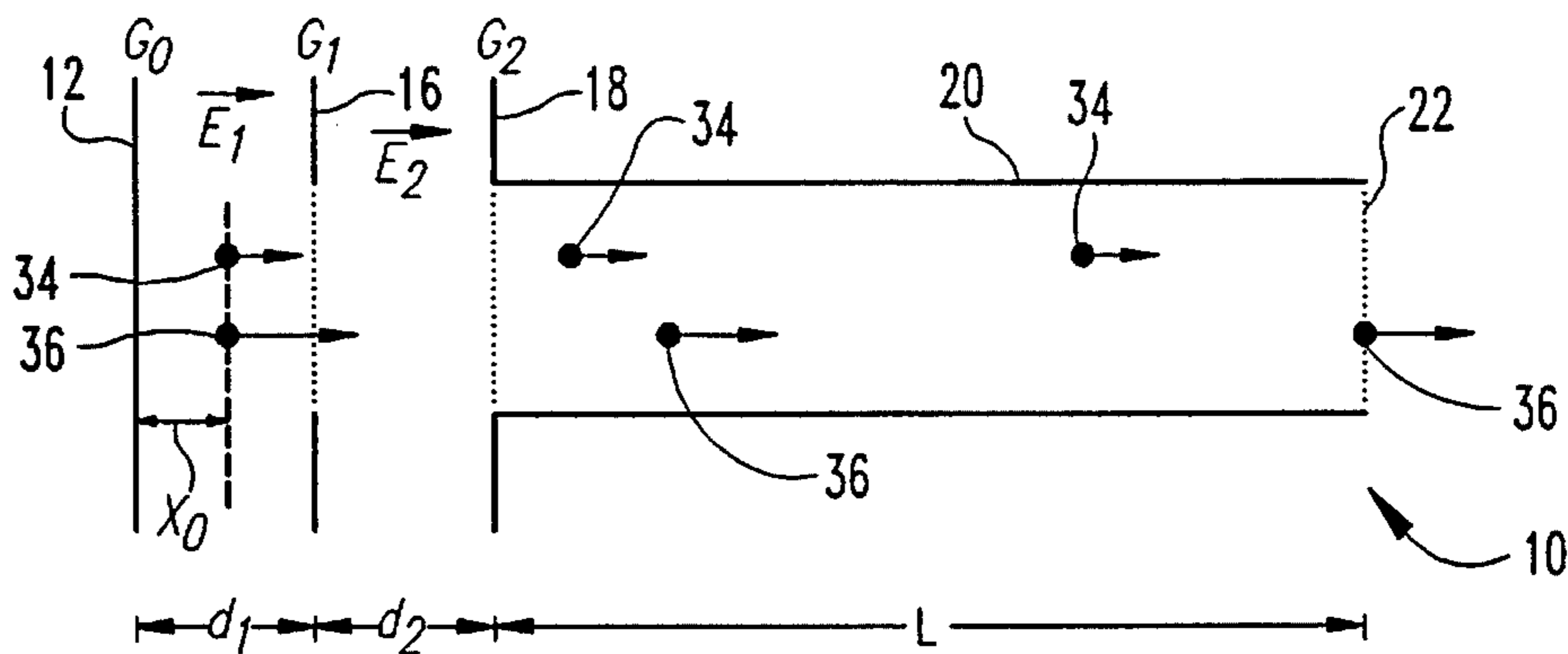
Fig. 3 (Prior Art)
