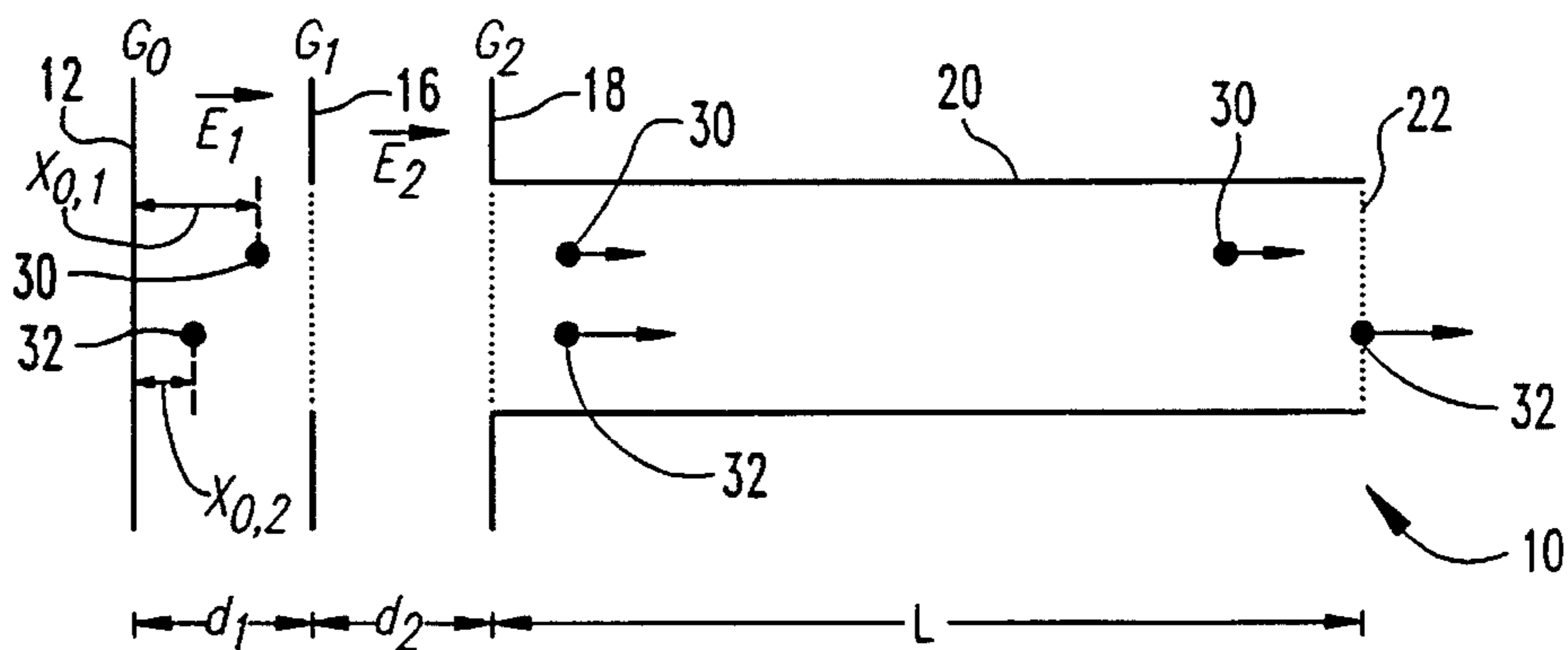
Fig. 2 (Prior Art)
