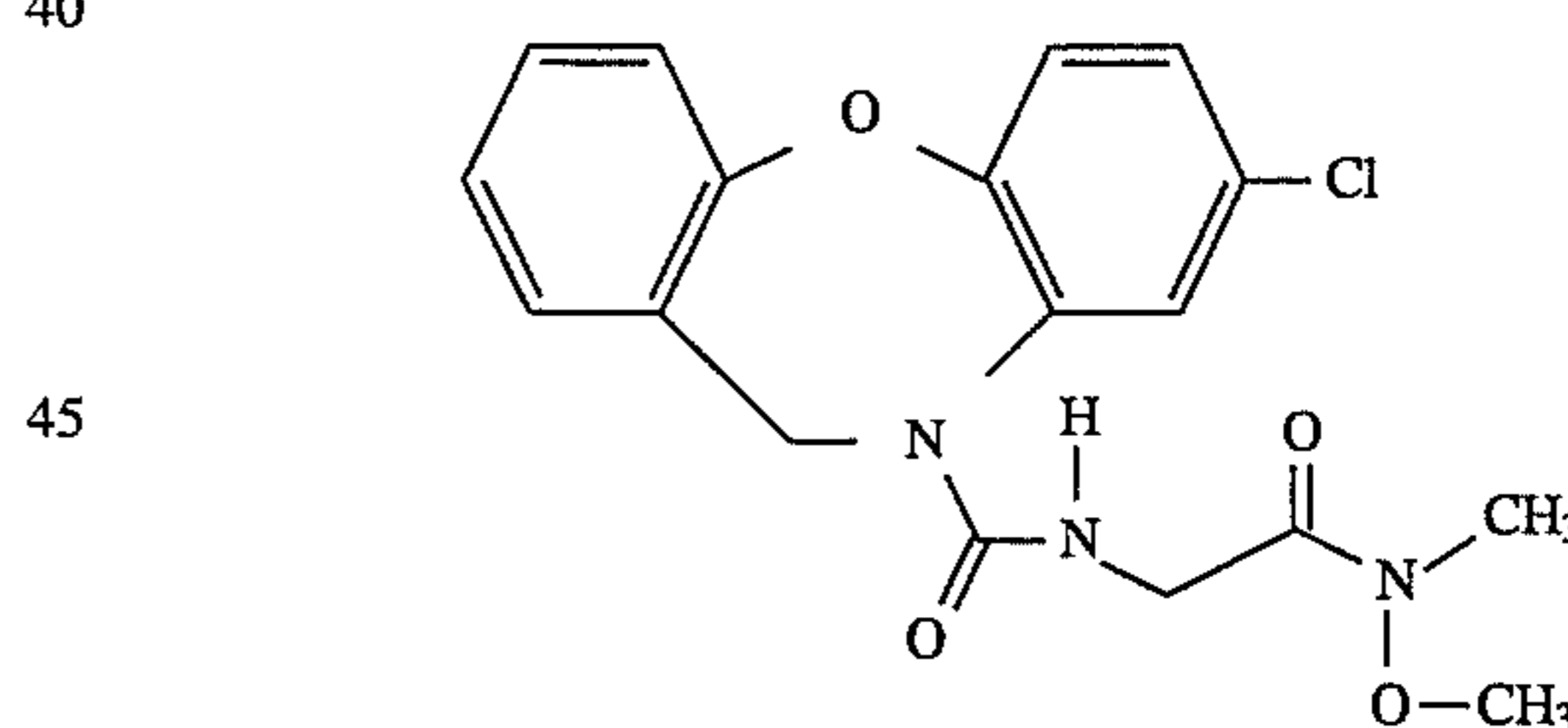
8-chloro-N-[[[(methoxy)methylamino]carbonyl]-methyl]dibenz[b,f][1,4]oxazepine-10(11H)-carboxamide (42)
