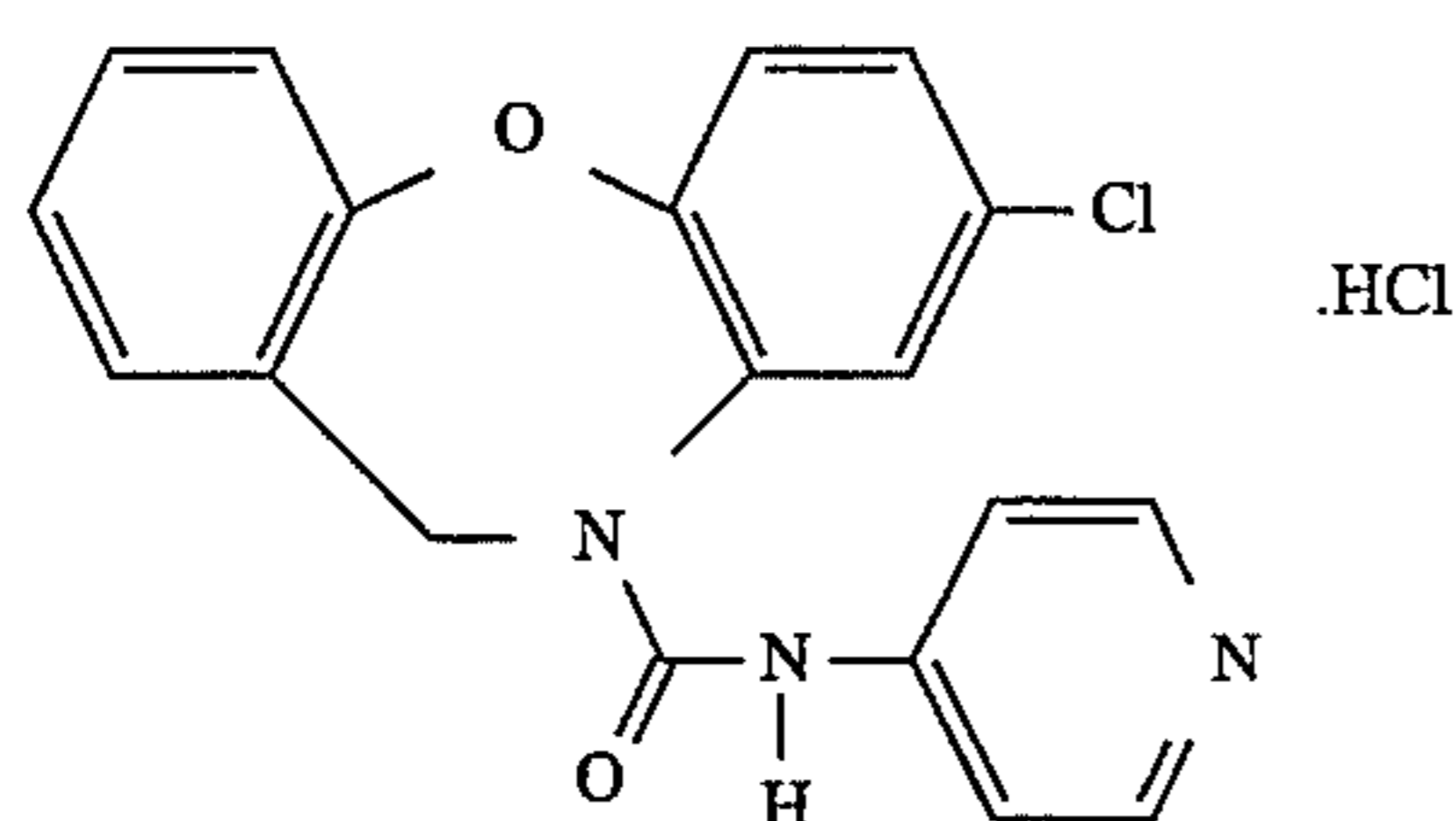
8-chloro-N-(4-pyridinyl)dibenz[b,f][1,4]oxazepine-10(11H)-carboxamide, monohydrochloride (40)
