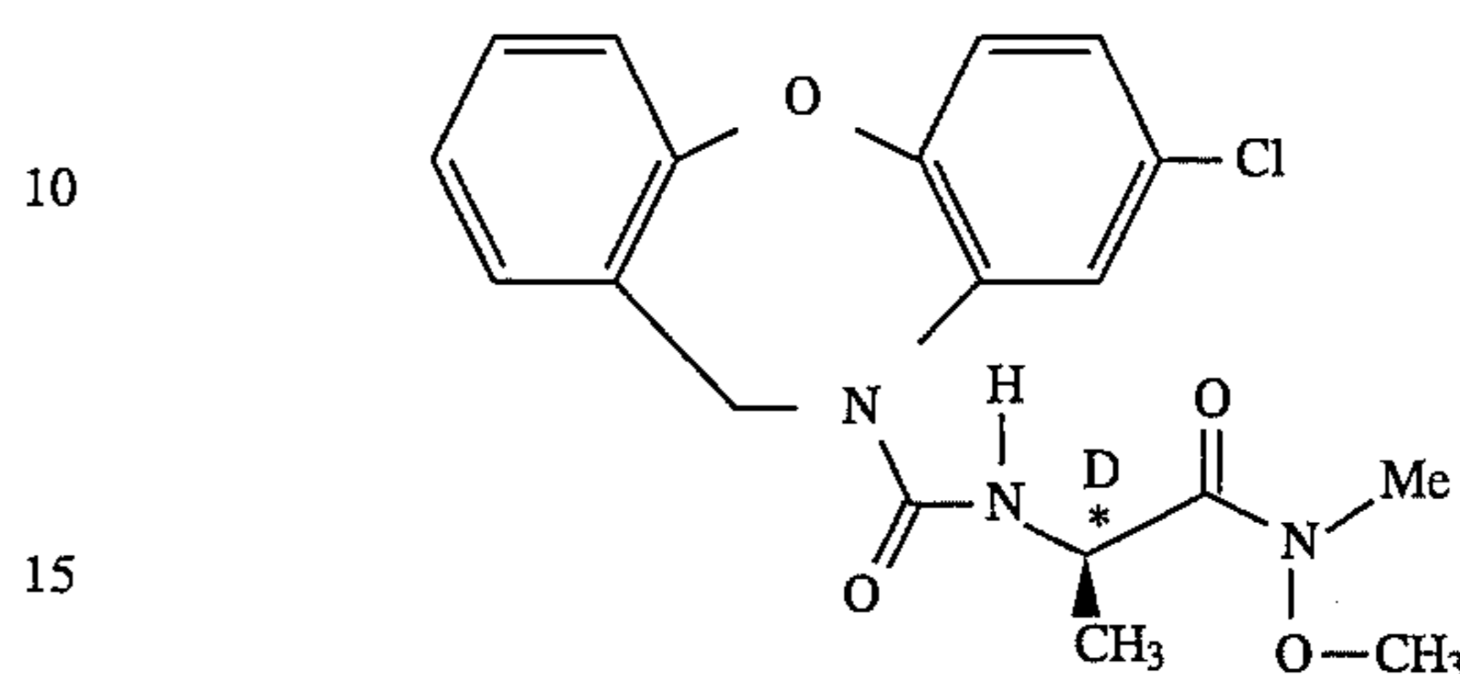
8-chloro-N-[1R-[[[(methoxy)methylamino]-carbonyl]-ethyl]dibenz[b,f][1,4]oxazepine-10(11H)-carboxamide (41)
