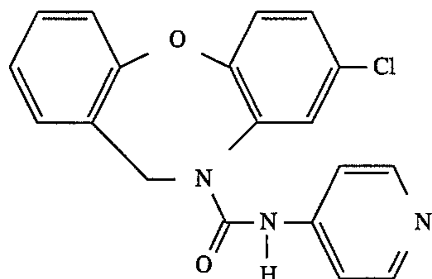
8-chloro-N-(4-pyridinyl)dibenz[b,f][1,4]oxazepine-10(11H)-carboxamide (39)
