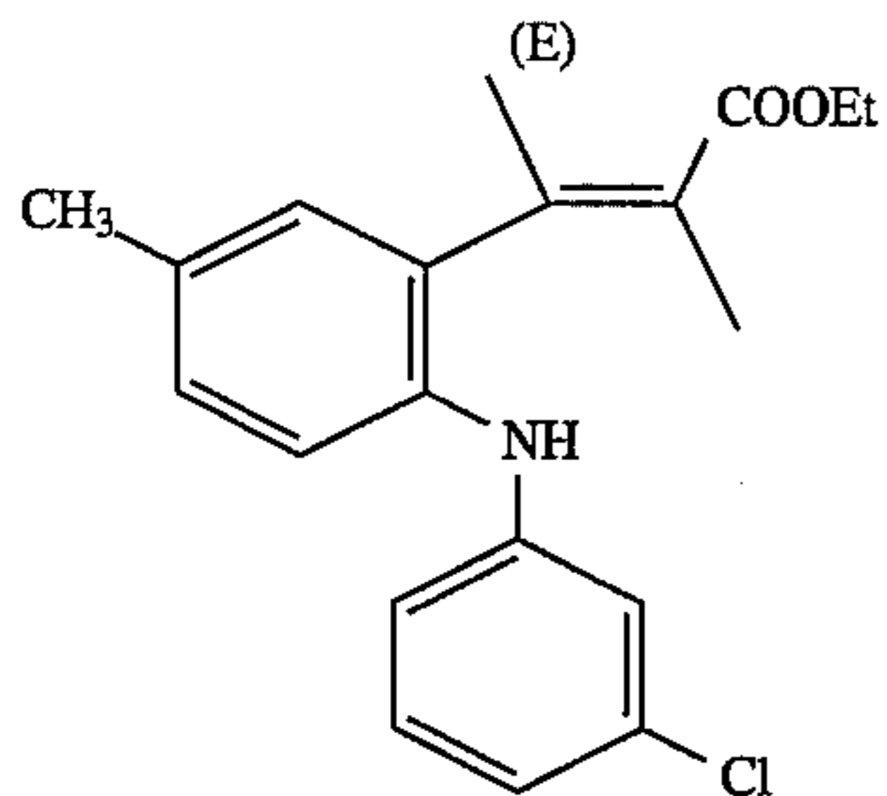
(F) C 16 H 14 ClNO 2 (287.74)
