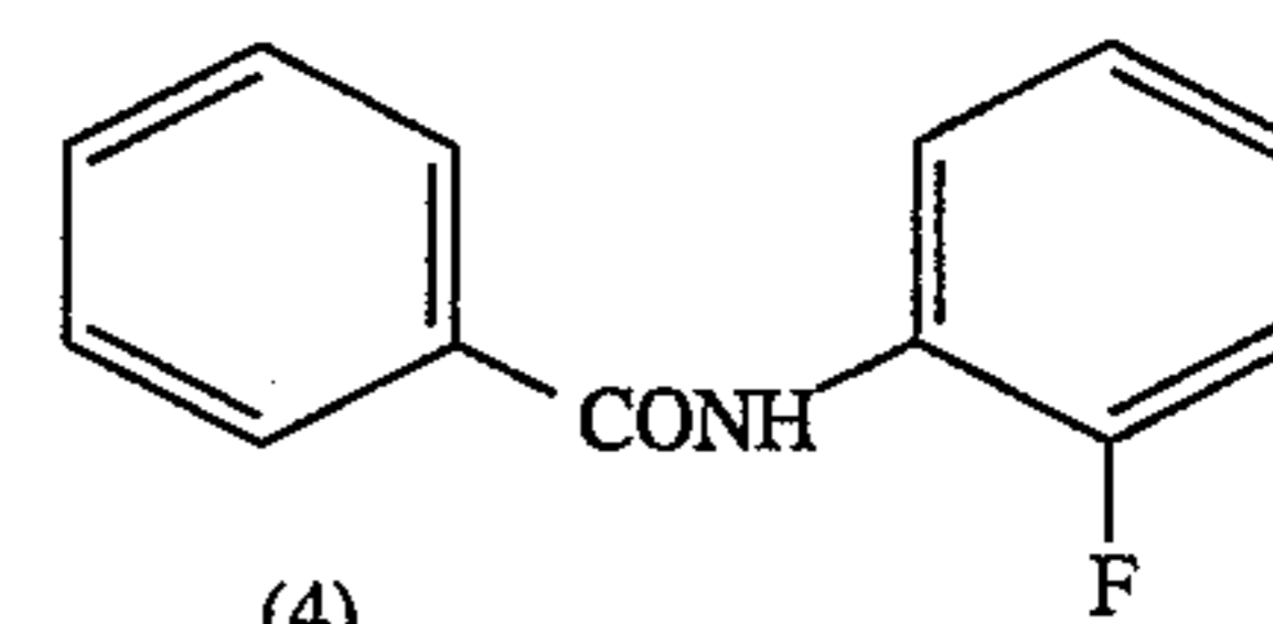
(4) C 13 H 10 FNO (215.22)
