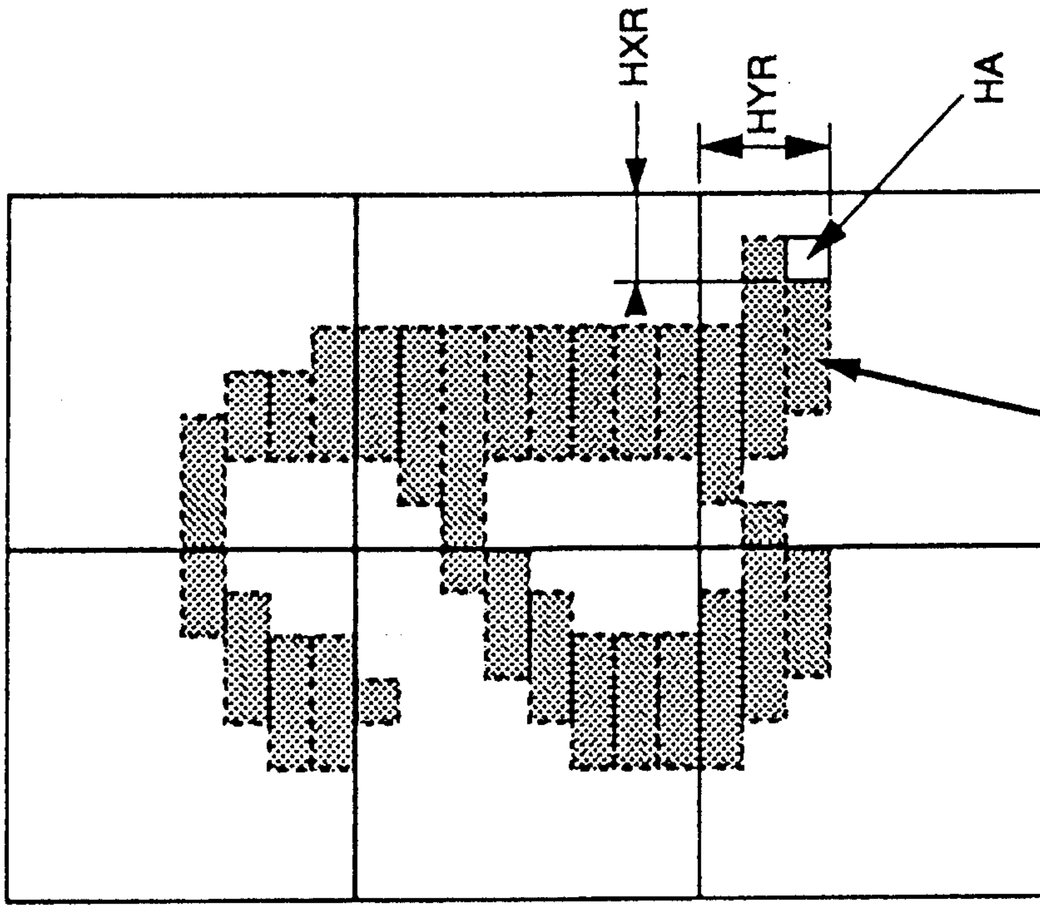
Bottom to Top FIG. 22B
