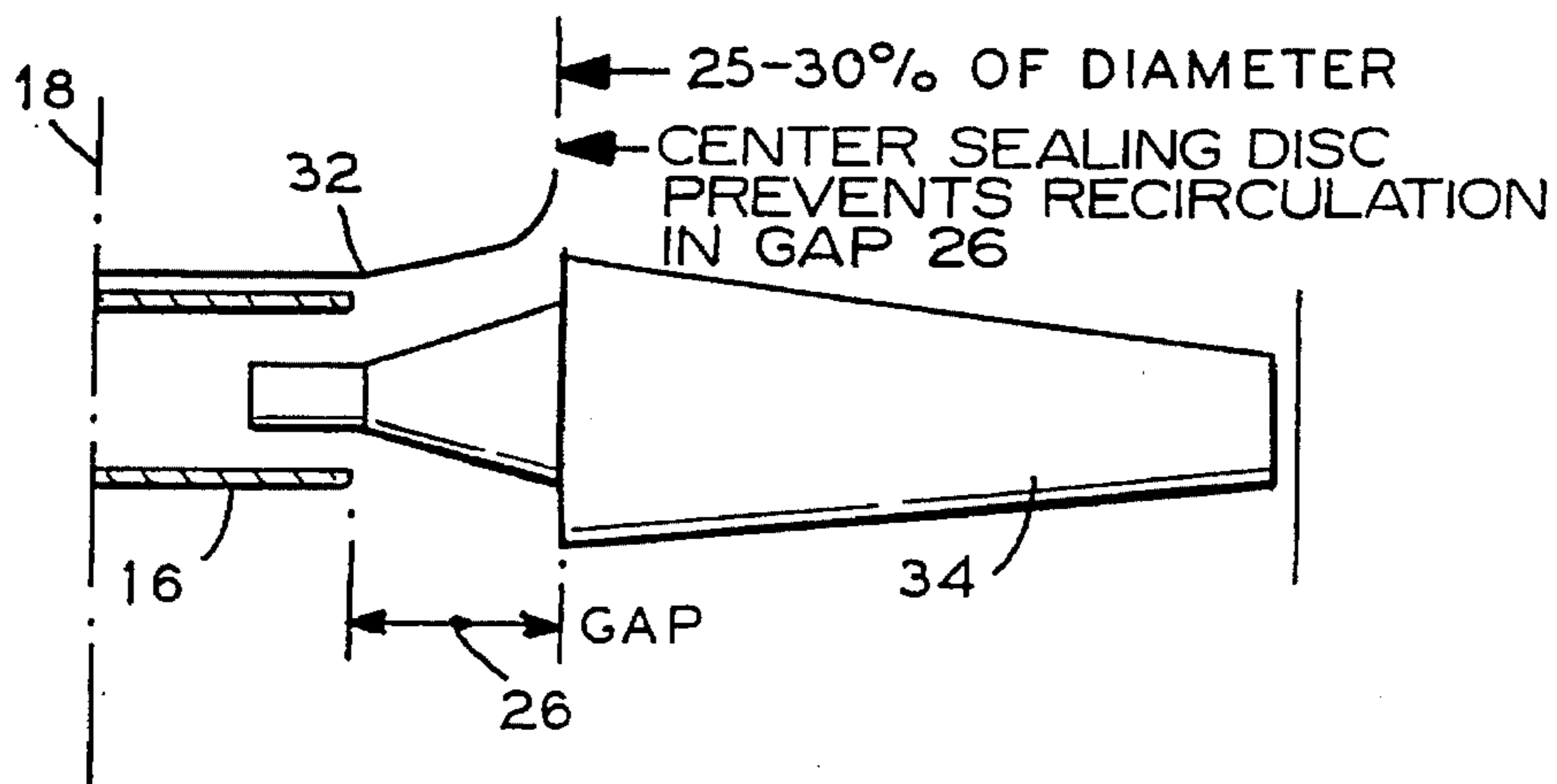
FIG. 3 (PRIOR ART)
