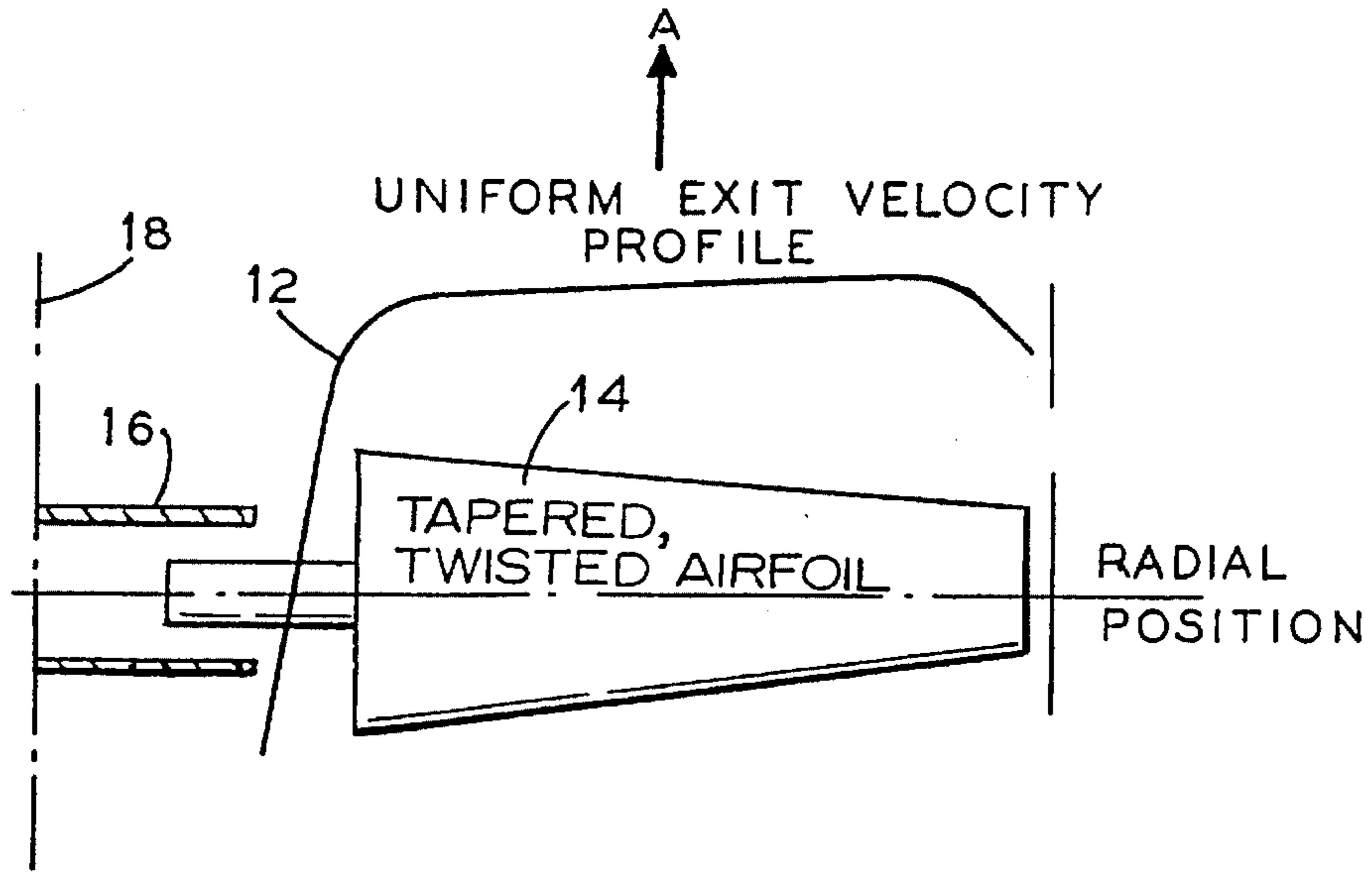
FIG. 1 (PRIOR ART)
